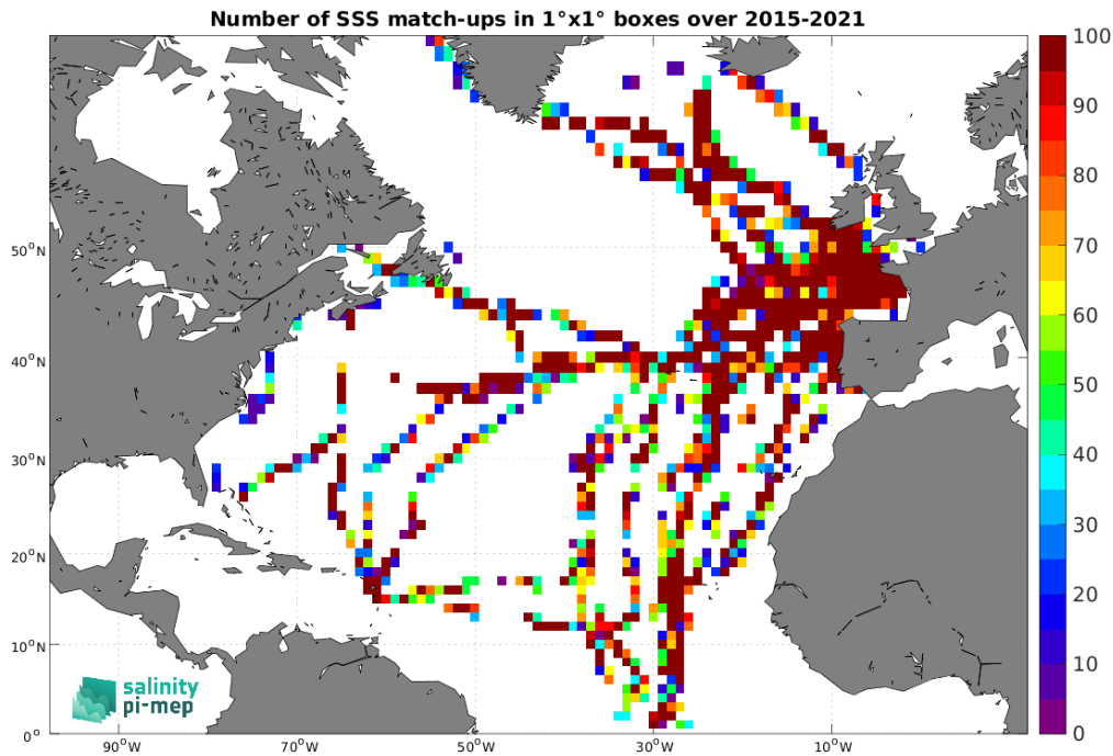
Figure 5: Number of SSS match-ups between TSG (GOSUD-Sailing-ship) SSS and the SMAP SSS L2 v6 (RSS) SSS product for the North Atlantic Ocean Pi-MEP region over 1^\circ \times 1^\circ boxes and for the full satellite product period.
