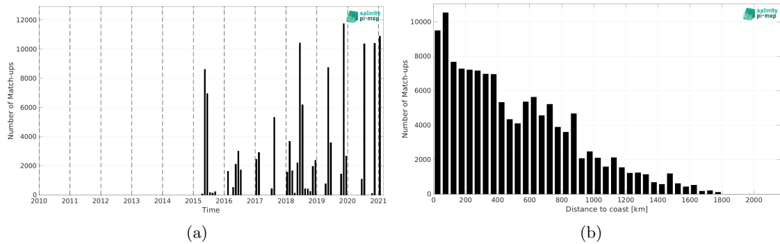
Figure 2: Number of match-ups between TSG (GOSUD-Sailing-ship) and SMAP SSS L2 v6 (RSS) SSS as a function of time (a) and as function of the distance to coast (b) over the North Atlantic Ocean Pi-MEP region and for the full satellite product period.
