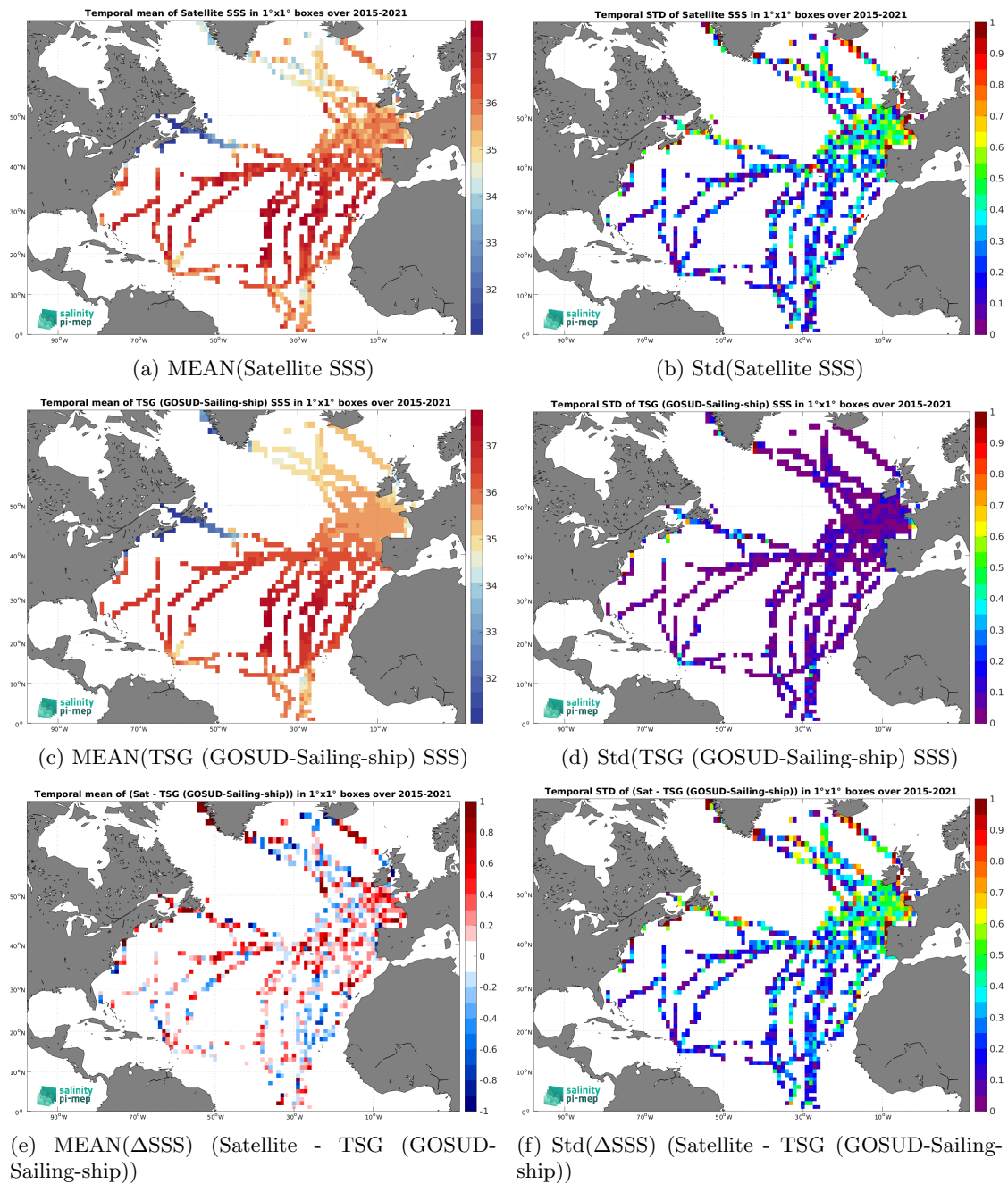
Figure 7: Temporal mean (left) and Std (right) of SSS from SMAP SSS L2 v6 (RSS) (top), TSG (GOSUD-Sailing-ship) (middle), and of \Delta SSS (Satellite - TSG (GOSUD-Sailing-ship)). Only match-up pairs are used to generate these maps.
