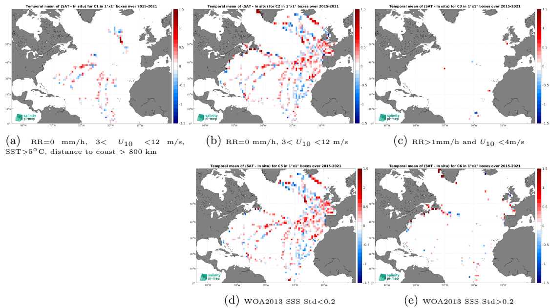
Figure 14: Temporal mean gridded over spatial boxes of size 1^\circ \times 1^\circ of \Delta\text{SSS} (SMAP SSS L2 v6 (RSS) - TSG (GOSUD-Sailing-ship)) for 5 different subdatasets corresponding to:RR=0 mm/h, 3 < U_{10} < 12 m/s, SST > 5°C, distance to coast > 800 km (a), RR=0 mm/h, 3 < U_{10} < 12 m/s (b), RR > 1mm/h and U_{10} < 4 m/s (c), WOA2013 SSS Std < 0.2 (d), WOA2013 SSS Std > 0.2 (e).
