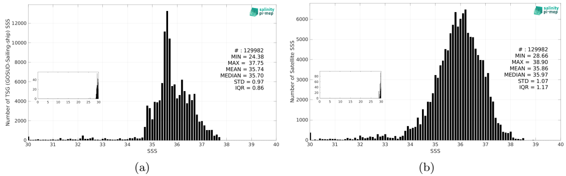
Figure 3: Histograms of SSS from TSG (GOSUD-Sailing-ship) (a) and SMAP SSS L2 v6 (RSS) (b) considering all match-up pairs per bins of 0.1 over the North Atlantic Ocean Pi-MEP region and for the full satellite product period.
