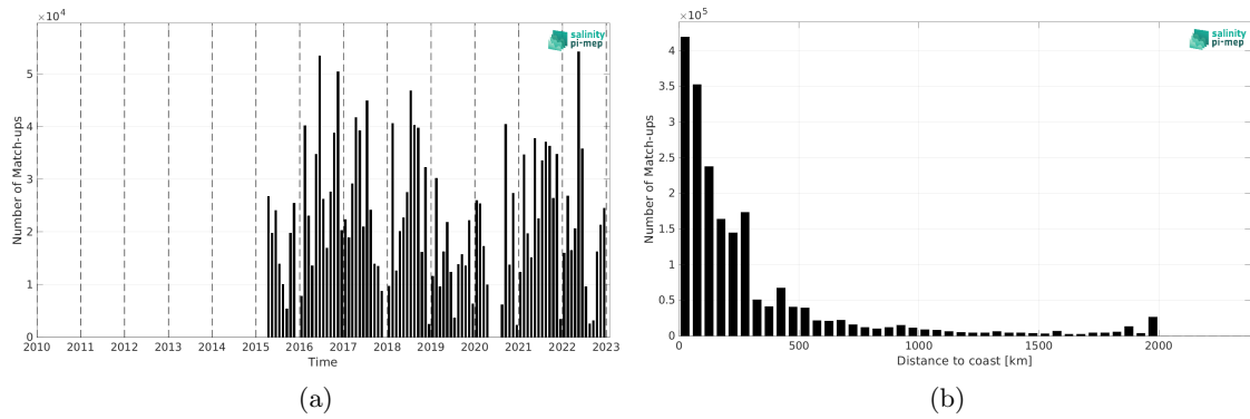
Figure 2: Number of match-ups between TSG (GOSUD-Research-vessel) and SMAP SSS L2 v6 (RSS) SSS as a function of time (a) and as function of the distance to coast (b) over the North Atlantic Ocean Pi-MEP region and for the full satellite product period.
