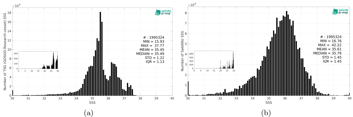
Figure 3: Histograms of SSS from TSG (GOSUD-Research-vessel) (a) and SMAP SSS L2 v6 (RSS) (b) considering all match-up pairs per bins of 0.1 over the North Atlantic Ocean Pi-MEP region and for the full satellite product period.
