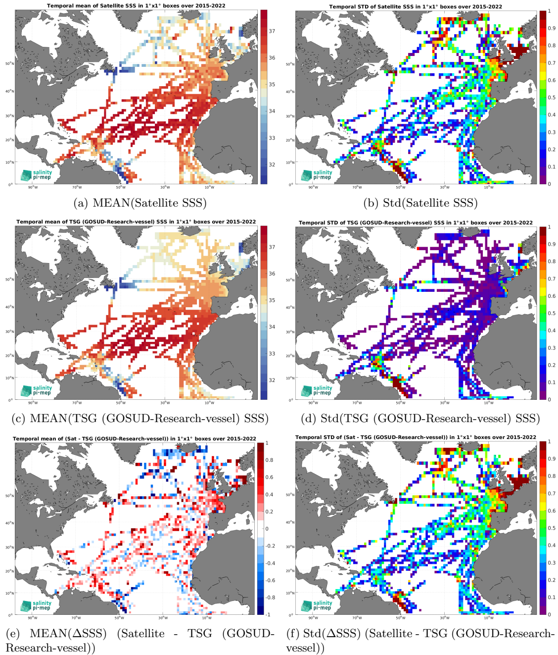
Figure 7: Temporal mean (left) and Std (right) of SSS from SMAP SSS L2 v6 (RSS) (top), TSG (GOSUD-Research-vessel) (middle), and of \Delta SSS (Satellite - TSG (GOSUD-Research-vessel)). Only match-up pairs are used to generate these maps.
