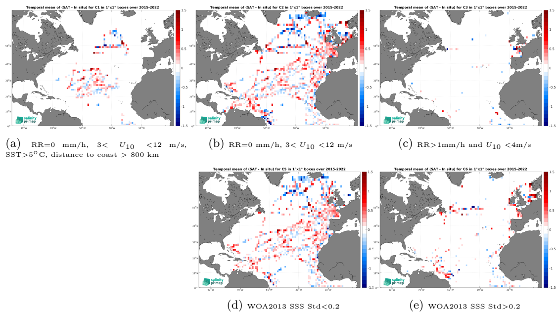
Figure 14: Temporal mean gridded over spatial boxes of size 1^\circ \times 1^\circ of \Delta\text{SSS} (SMAP SSS L2 v6 (RSS) - TSG (GOSUD-Research-vessel)) for 5 different subdatasets corresponding to:RR=0 mm/h, 3 < U_{10} < 12 m/s, SST >5^\circ\text{C} , distance to coast > 800 km (a), RR=0 mm/h, 3 < U_{10} < 12 m/s (b), RR >1 mm/h and U_{10} < 4 m/s (c), WOA2013 SSS Std <0.2 (d), WOA2013 SSS Std >0.2 (e).
