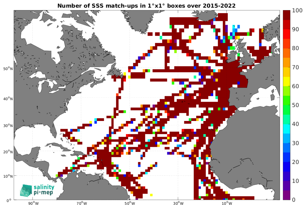
Figure 5: Number of SSS match-ups between TSG (GOSUD-Research-vessel) SSS and the SMAP SSS L2 v6 (RSS) SSS product for the North Atlantic Ocean Pi-MEP region over 1^\circ \times 1^\circ boxes and for the full satellite product period.
