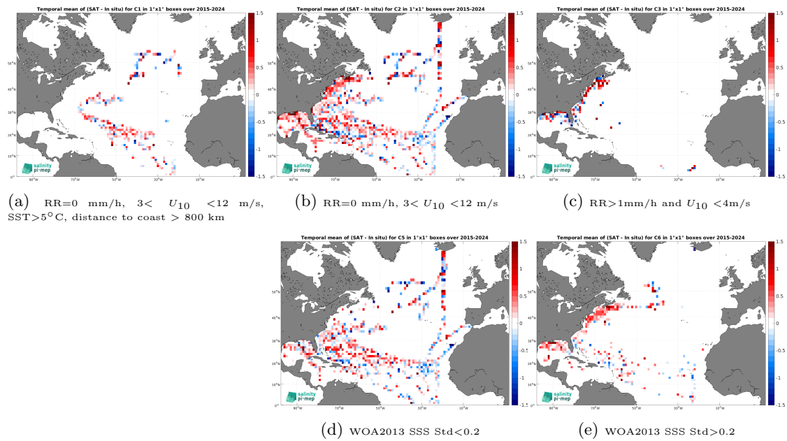
Figure 14: Temporal mean gridded over spatial boxes of size 1^\circ \times 1^\circ of \Delta\text{SSS} (SMAP SSS L2 v6 - 40 km (RSS) - TSG (SAMOS)) for 5 different subdatasets corresponding to: RR=0 mm/h, 3 < U_{10} < 12 m/s, SST > 5^\circ\text{C} , distance to coast > 800 km (a), RR=0 mm/h, 3 < U_{10} < 12 m/s (b), RR > 1 mm/h and U_{10} < 4 m/s (c), WOA2013 SSS Std < 0.2 (d), WOA2013 SSS Std > 0.2 (e).
