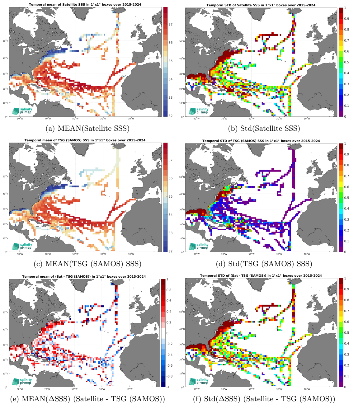
Figure 7: Temporal mean (left) and Std (right) of SSS from SMAP SSS L2 v6 - 40 km (RSS) (top), TSG (SAMOS) (middle), and of \Delta SSS (Satellite - TSG (SAMOS)). Only match-up pairs are used to generate these maps.
