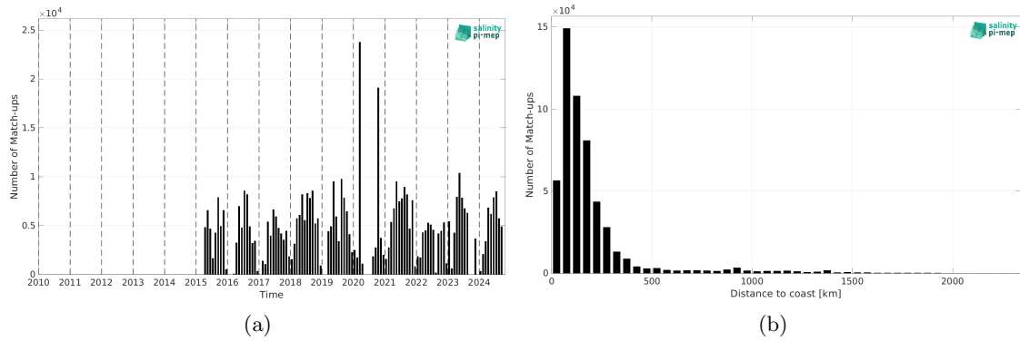
Figure 2: Number of match-ups between TSG (SAMOS) and SMAP SSS L2 v6 - 40 km (RSS) SSS as a function of time (a) and as function of the distance to coast (b) over the North Atlantic Ocean Pi-MEP region and for the full satellite product period.
