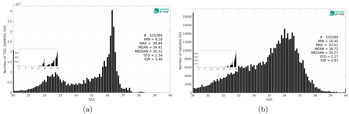
Figure 3: Histograms of SSS from TSG (SAMOS) (a) and SMAP SSS L2 v6 - 40 km (RSS) (b) considering all match-up pairs per bins of 0.1 over the North Atlantic Ocean Pi-MEP region and for the full satellite product period.
