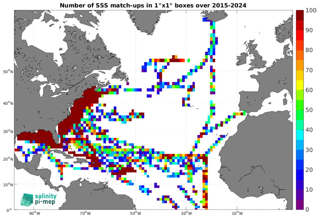
Figure 5: Number of SSS match-ups between TSG (SAMOS) SSS and the SMAP SSS L2 v6 - 40 km (RSS) SSS product for the North Atlantic Ocean Pi-MEP region over 1^\circ \times 1^\circ boxes and for the full satellite product period.
