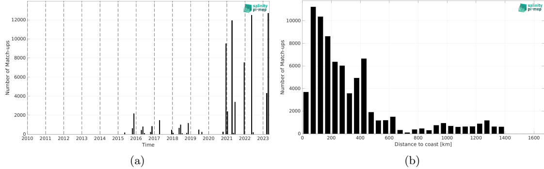
Figure 2: Number of match-ups between TSG (Polarstern) and SMAP SSS L2 v6 - 40 km (RSS) SSS as a function of time (a) and as function of the distance to coast (b) over the North Atlantic Ocean Pi-MEP region and for the full satellite product period.
