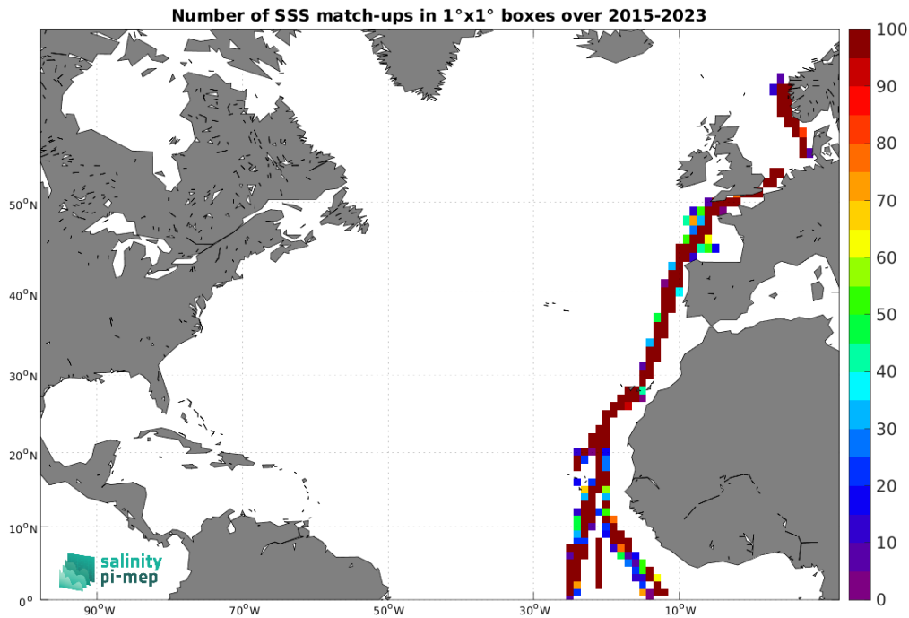
Figure 5: Number of SSS match-ups between TSG (Polarstern) SSS and the SMAP SSS L2 v6 - 40 km (RSS) SSS product for the North Atlantic Ocean Pi-MEP region over 1^\circ \times 1^\circ boxes and for the full satellite product period.
