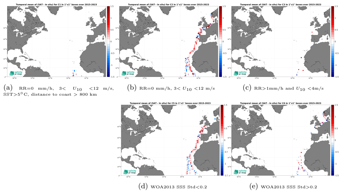
Figure 14: Temporal mean gridded over spatial boxes of size 1^\circ \times 1^\circ of \Delta\text{SSS} (SMAP SSS L2 v6 - 40 km (RSS) - TSG (Polarstern)) for 5 different subdatasets corresponding to:RR=0 mm/h, 3 < U_{10} < 12 m/s, SST > 5°C, distance to coast > 800 km (a), RR=0 mm/h, 3 < U_{10} < 12 m/s (b), RR > 1mm/h and U_{10} < 4 m/s (c), WOA2013 SSS Std < 0.2 (d), WOA2013 SSS Std > 0.2 (e).
