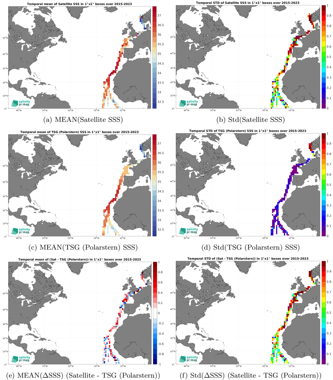
Figure 7: Temporal mean (left) and Std (right) of SSS from SMAP SSS L2 v6 - 40 km (RSS) (top), TSG (Polarstern) (middle), and of \Delta SSS (Satellite - TSG (Polarstern)). Only match-up pairs are used to generate these maps.
