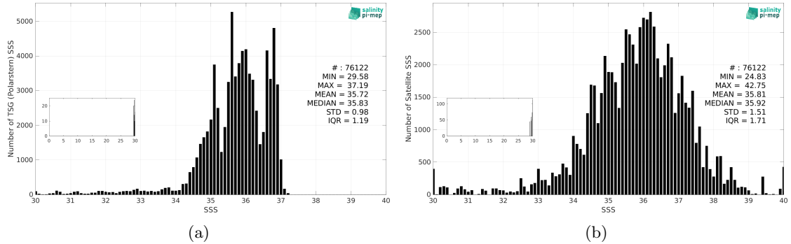
Figure 3: Histograms of SSS from TSG (Polarstern) (a) and SMAP SSS L2 v6 - 40 km (RSS) (b) considering all match-up pairs per bins of 0.1 over the North Atlantic Ocean Pi-MEP region and for the full satellite product period.
