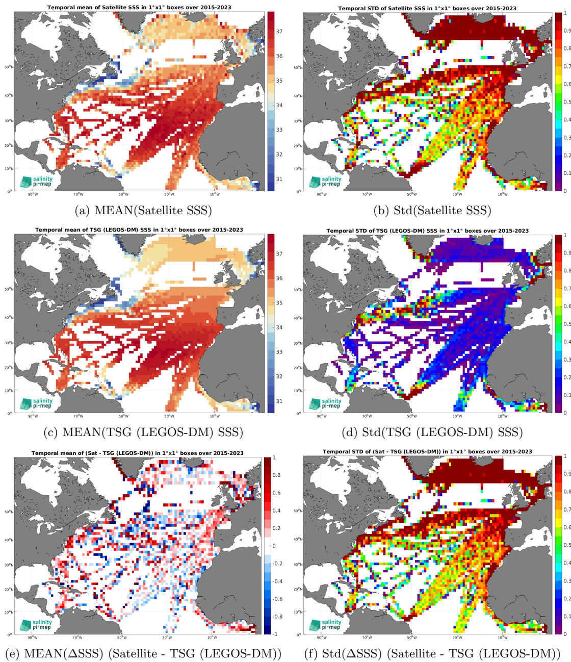
Figure 7: Temporal mean (left) and Std (right) of SSS from SMAP SSS L2 v6 - 40 km (RSS) (top), TSG (LEGOS-DM) (middle), and of \Delta SSS (Satellite - TSG (LEGOS-DM)). Only match-up pairs are used to generate these maps.
