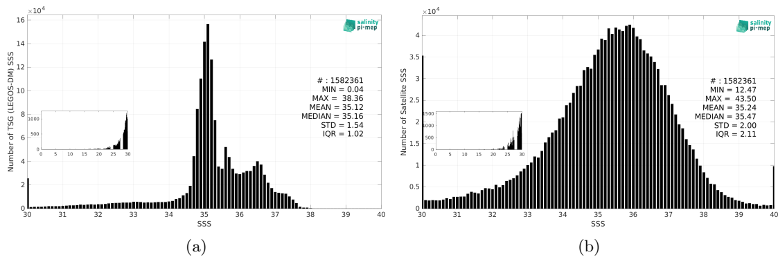
Figure 3: Histograms of SSS from TSG (LEGOS-DM) (a) and SMAP SSS L2 v6 - 40 km (RSS) (b) considering all match-up pairs per bins of 0.1 over the North Atlantic Ocean Pi-MEP region and for the full satellite product period.
