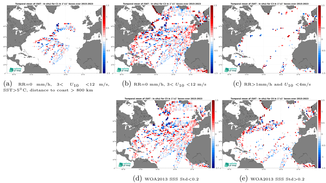
Figure 14: Temporal mean gridded over spatial boxes of size 1^\circ \times 1^\circ of \Delta\text{SSS} (SMAP SSS L2 v6 - 40 km (RSS) - TSG (LEGOS-DM)) for 5 different subdatasets corresponding to:RR=0 mm/h, 3 < U_{10} < 12 m/s, SST >5^\circ\text{C} , distance to coast > 800 km (a), RR=0 mm/h, 3 < U_{10} < 12 m/s (b), RR >1 mm/h and U_{10} < 4 m/s (c), WOA2013 SSS Std <0.2 (d), WOA2013 SSS Std >0.2 (e).
