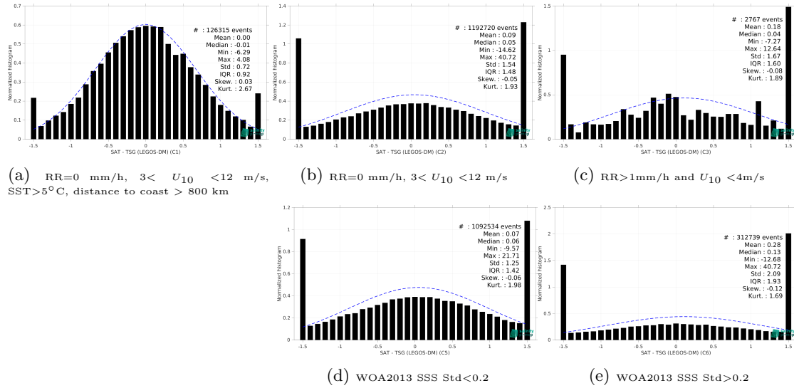
Figure 15: Normalized histogram of \Delta\text{SSS} (SMAP SSS L2 v6 - 40 km (RSS) - TSG (LEGOS-DM)) for 5 different subdatasets corresponding to: RR=0 mm/h, 3 < U_{10} < 12 m/s, SST>5°C, distance to coast > 800 km (a), RR=0 mm/h, 3 < U_{10} < 12 m/s (b), RR>1mm/h and U_{10} < 4 m/s (c), WOA2013 SSS Std<0.2 (d), WOA2013 SSS Std>0.2 (e).
