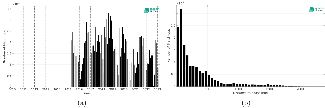
Figure 2: Number of match-ups between TSG (LEGOS-DM) and SMAP SSS L2 v6 - 40 km (RSS) SSS as a function of time (a) and as function of the distance to coast (b) over the North Atlantic Ocean Pi-MEP region and for the full satellite product period.
