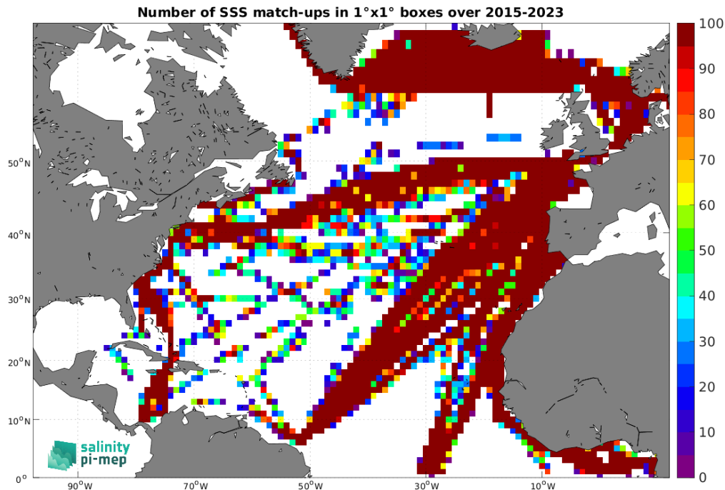
Figure 5: Number of SSS match-ups between TSG (LEGOS-DM) SSS and the SMAP SSS L2 v6 - 40 km (RSS) SSS product for the North Atlantic Ocean Pi-MEP region over 1^\circ \times 1^\circ boxes and for the full satellite product period.
