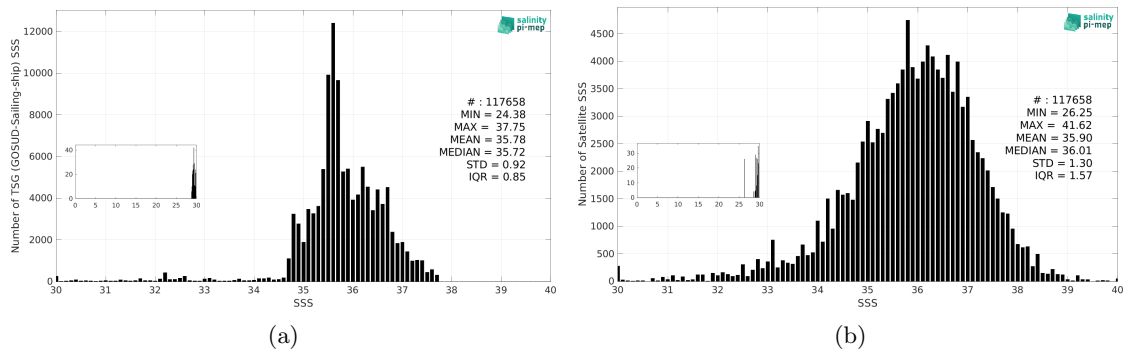
Figure 3: Histograms of SSS from TSG (GOSUD-Sailing-ship) (a) and SMAP SSS L2 v6 - 40 km (RSS) (b) considering all match-up pairs per bins of 0.1 over the North Atlantic Ocean Pi-MEP region and for the full satellite product period.
