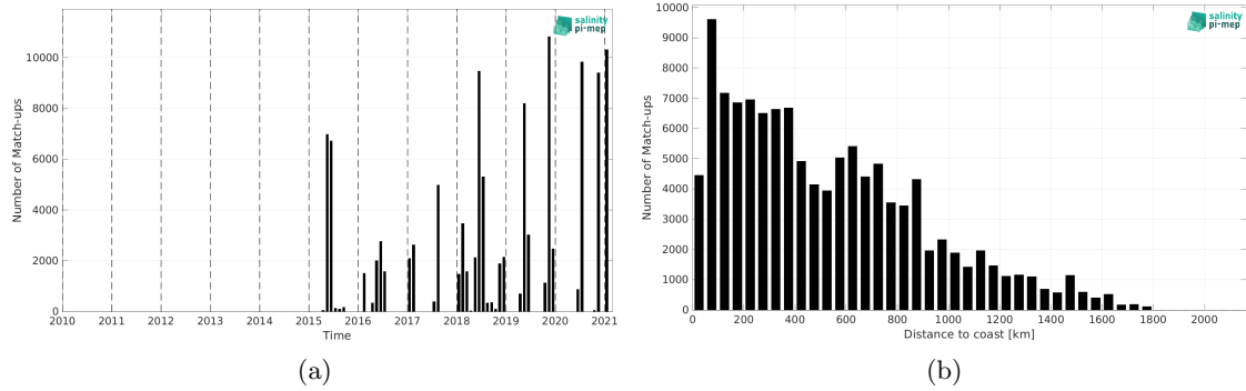
Figure 2: Number of match-ups between TSG (GOSUD-Sailing-ship) and SMAP SSS L2 v6 - 40 km (RSS) SSS as a function of time (a) and as function of the distance to coast (b) over the North Atlantic Ocean Pi-MEP region and for the full satellite product period.
