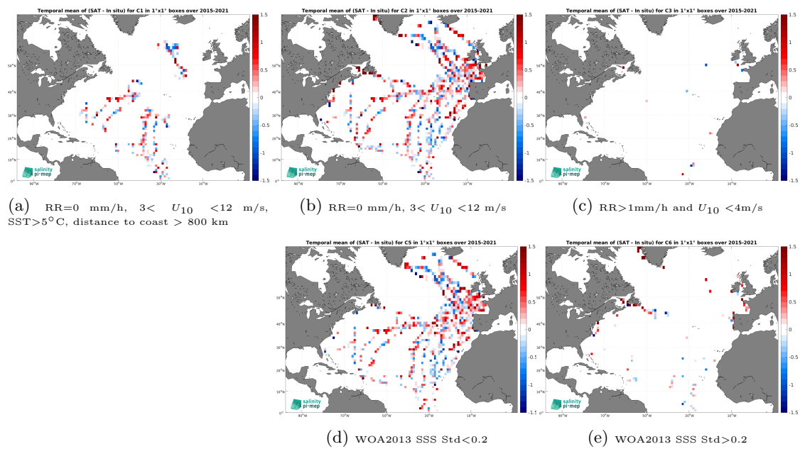
Figure 14: Temporal mean gridded over spatial boxes of size 1^\circ \times 1^\circ of \Delta\text{SSS} (SMAP SSS L2 v6 - 40 km (RSS) - TSG (GOSUD-Sailing-ship)) for 5 different subdatasets corresponding to:RR=0 mm/h, 3 < U_{10} < 12 m/s, SST >5^\circ\text{C} , distance to coast > 800 km (a), RR=0 mm/h, 3 < U_{10} < 12 m/s (b), RR >1 mm/h and U_{10} < 4 m/s (c), WOA2013 SSS Std <0.2 (d), WOA2013 SSS Std >0.2 (e).
