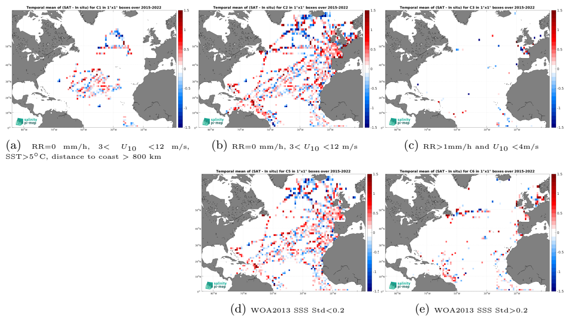
Figure 14: Temporal mean gridded over spatial boxes of size 1^\circ \times 1^\circ of \Delta\text{SSS} (SMAP SSS L2 v6 - 40 km (RSS) - TSG (GOSUD-Research-vessel)) for 5 different subdatasets corresponding to:RR=0 mm/h, 3 < U_{10} < 12 m/s, SST > 5°C, distance to coast > 800 km (a), RR=0 mm/h, 3 < U_{10} < 12 m/s (b), RR > 1mm/h and U_{10} < 4 m/s (c), WOA2013 SSS Std < 0.2 (d), WOA2013 SSS Std > 0.2 (e).
