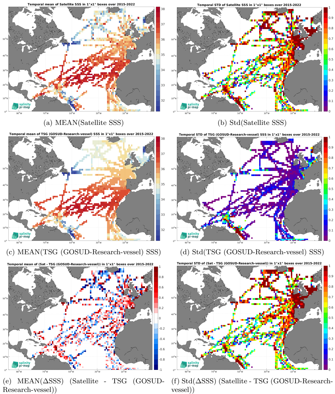
Figure 7: Temporal mean (left) and Std (right) of SSS from SMAP SSS L2 v6 - 40 km (RSS) (top), TSG (GOSUD-Research-vessel) (middle), and of \Delta SSS (Satellite - TSG (GOSUD-Research-vessel)). Only match-up pairs are used to generate these maps.
