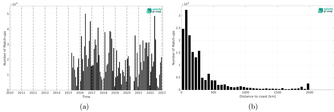
Figure 2: Number of match-ups between TSG (GOSUD-Research-vessel) and SMAP SSS L2 v6 - 40 km (RSS) SSS as a function of time (a) and as function of the distance to coast (b) over the North Atlantic Ocean Pi-MEP region and for the full satellite product period.
