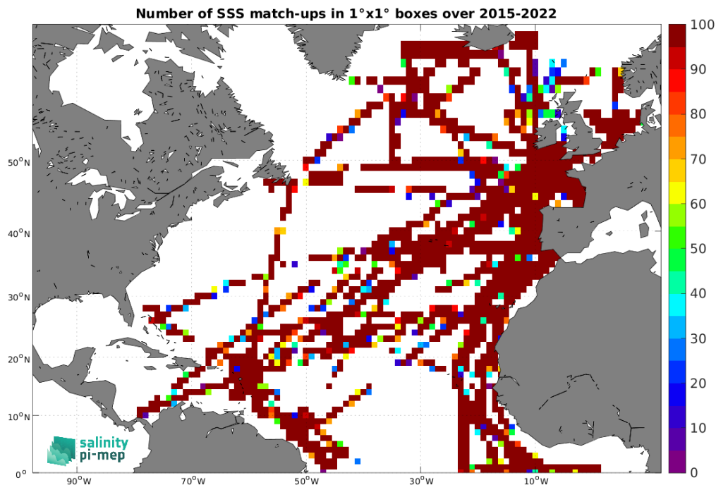
Figure 5: Number of SSS match-ups between TSG (GOSUD-Research-vessel) SSS and the SMAP SSS L2 v6 - 40 km (RSS) SSS product for the North Atlantic Ocean Pi-MEP region over 1^\circ \times 1^\circ boxes and for the full satellite product period.
