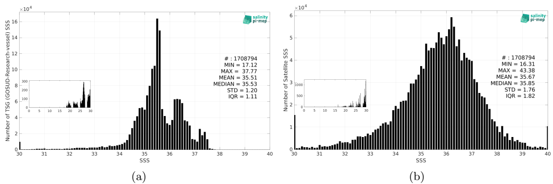
Figure 3: Histograms of SSS from TSG (GOSUD-Research-vessel) (a) and SMAP SSS L2 v6 - 40 km (RSS) (b) considering all match-up pairs per bins of 0.1 over the North Atlantic Ocean Pi-MEP region and for the full satellite product period.
