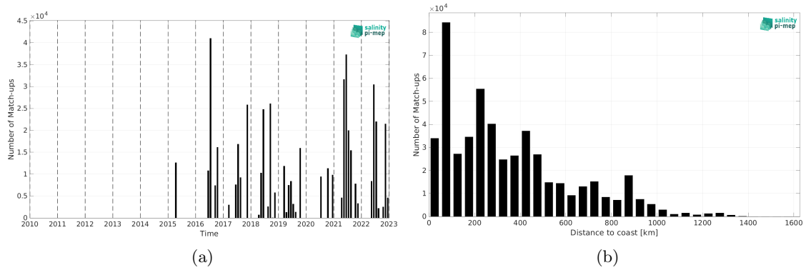
Figure 2: Number of match-ups between TSG (CSIC-UTM) and SMAP SSS L2 v6 - 40 km (RSS) SSS as a function of time (a) and as function of the distance to coast (b) over the North Atlantic Ocean Pi-MEP region and for the full satellite product period.
