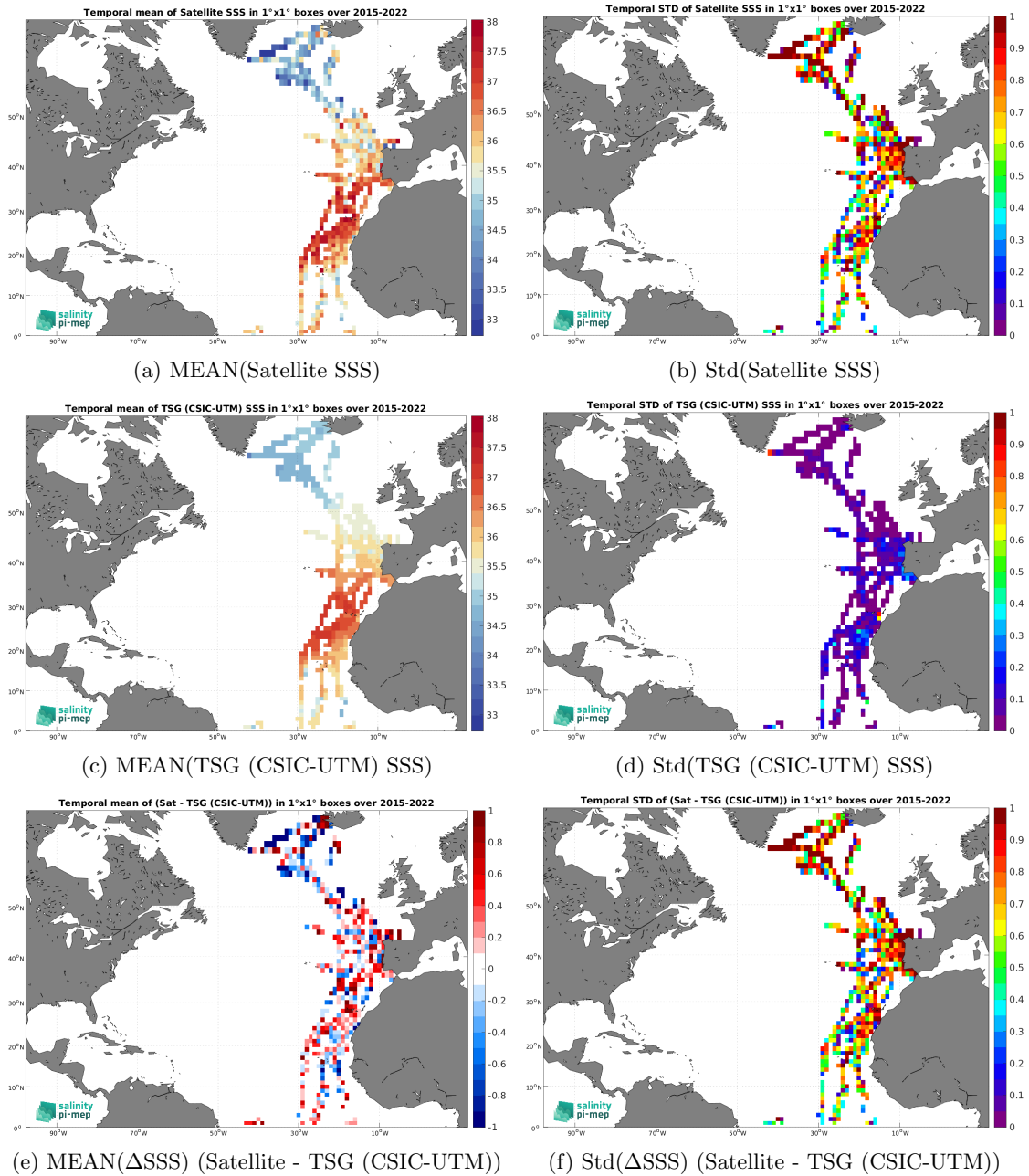
Figure 7: Temporal mean (left) and Std (right) of SSS from SMAP SSS L2 v6 - 40 km (RSS) (top), TSG (CSIC-UTM) (middle), and of \Delta SSS (Satellite - TSG (CSIC-UTM)). Only match-up pairs are used to generate these maps.
