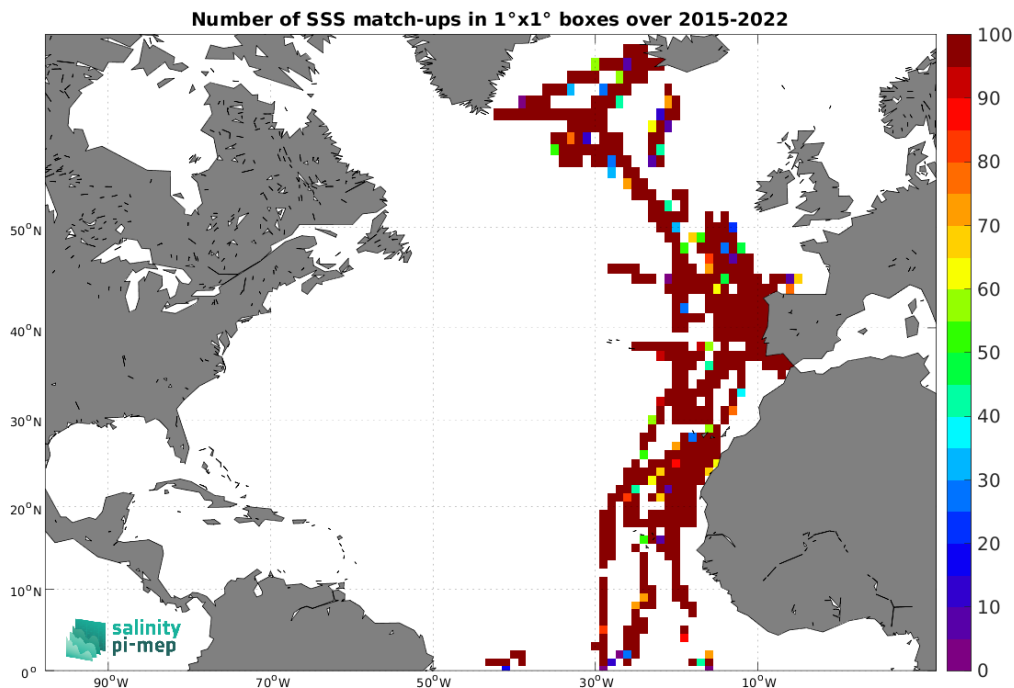
Figure 5: Number of SSS match-ups between TSG (CSIC-UTM) SSS and the SMAP SSS L2 v6 - 40 km (RSS) SSS product for the North Atlantic Ocean Pi-MEP region over 1^\circ \times 1^\circ boxes and for the full satellite product period.
