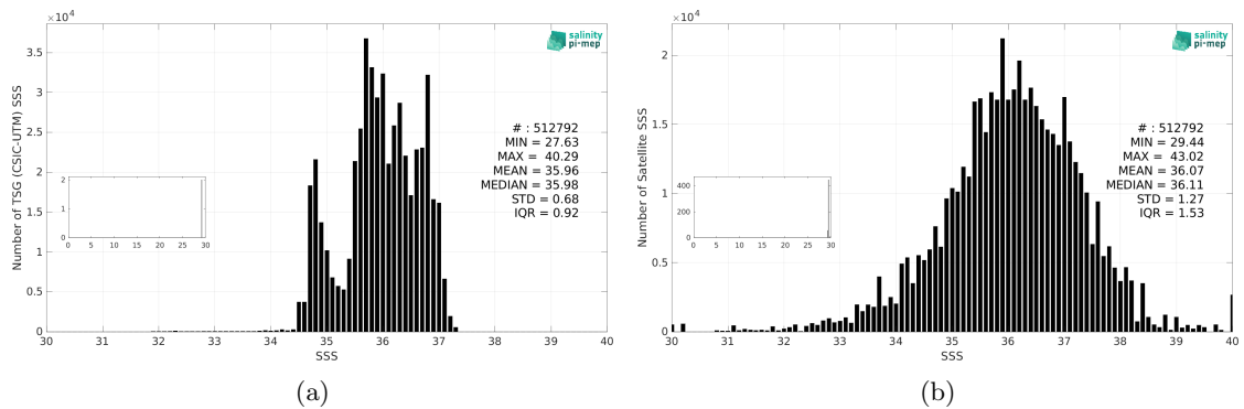
Figure 3: Histograms of SSS from TSG (CSIC-UTM) (a) and SMAP SSS L2 v6 - 40 km (RSS) (b) considering all match-up pairs per bins of 0.1 over the North Atlantic Ocean Pi-MEP region and for the full satellite product period.
