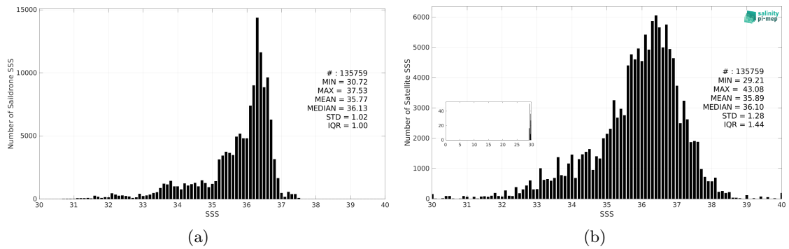
Figure 3: Histograms of SSS from Saildrone (a) and SMAP SSS L2 v6 - 40 km (RSS) (b) considering all match-up pairs per bins of 0.1 over the North Atlantic Ocean Pi-MEP region and for the full satellite product period.
