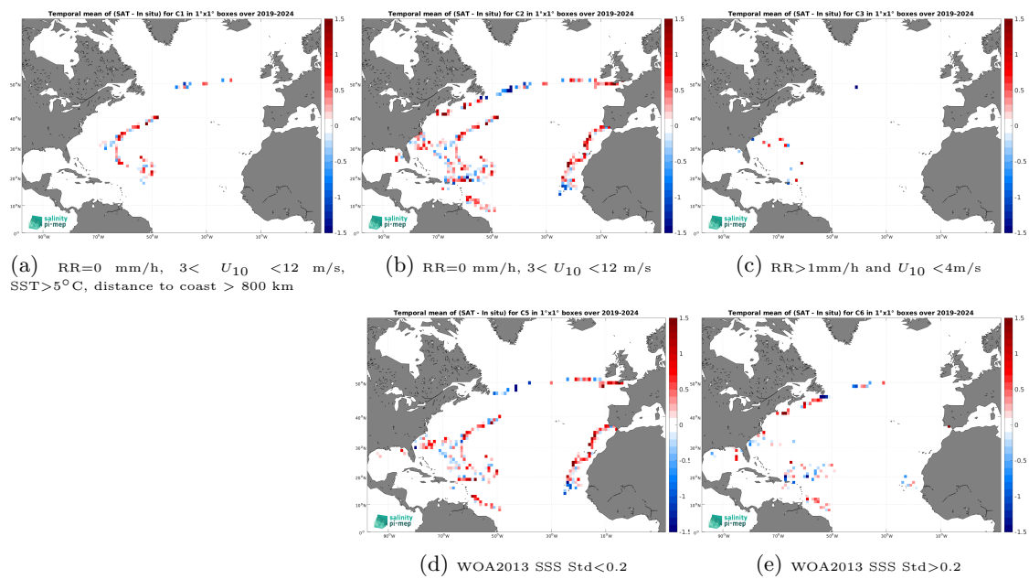
Figure 14: Temporal mean gridded over spatial boxes of size 1^\circ \times 1^\circ of \Delta\text{SSS} (SMAP SSS L2 v6 - 40 km (RSS) - Saldrone) for 5 different subdatasets corresponding to:RR=0 mm/h, 3 < U_{10} < 12 m/s, SST>5°C, distance to coast > 800 km (a), RR=0 mm/h, 3 < U_{10} < 12 m/s (b), RR>1mm/h and U_{10} < 4 m/s (c), WOA2013 SSS Std<0.2 (d), WOA2013 SSS Std>0.2 (e).
