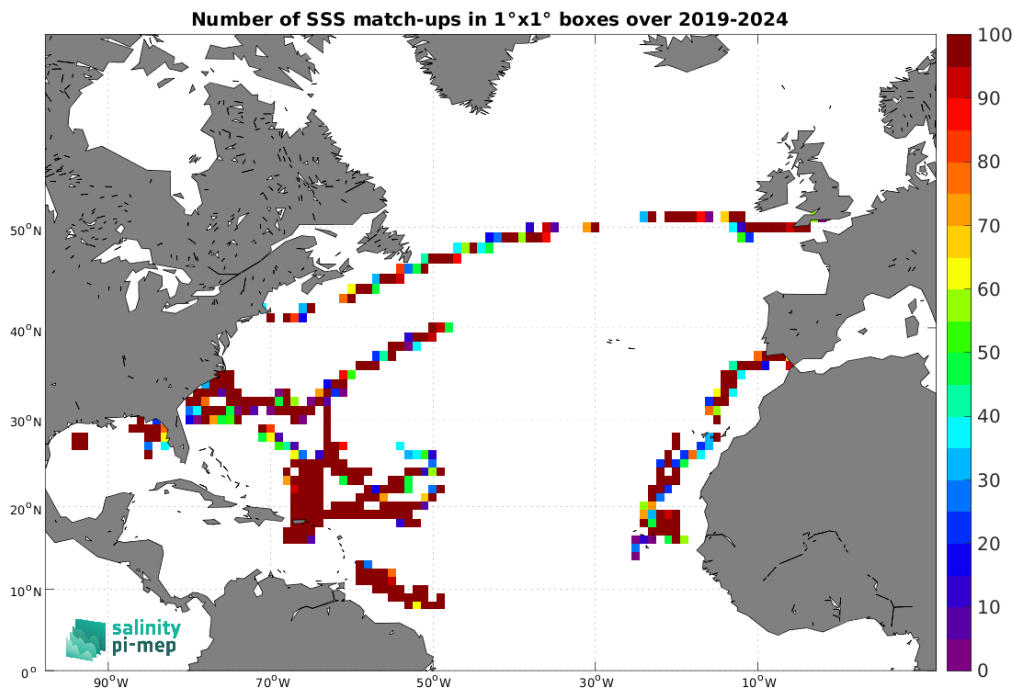
Figure 5: Number of SSS match-ups between Saildrone SSS and the SMAP SSS L2 v6 - 40 km (RSS) SSS product for the North Atlantic Ocean Pi-MEP region over 1^\circ \times 1^\circ boxes and for the full satellite product period.
