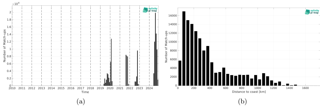
Figure 2: Number of match-ups between Saildrone and SMAP SSS L2 v6 - 40 km (RSS) SSS as a function of time (a) and as function of the distance to coast (b) over the North Atlantic Ocean Pi-MEP region and for the full satellite product period.
