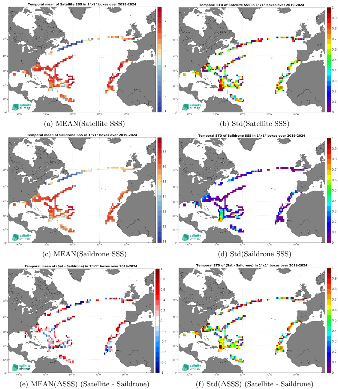
Figure 7: Temporal mean (left) and Std (right) of SSS from SMAP SSS L2 v6 - 40 km (RSS) (top), Sailldrone (middle), and of \Delta SSS (Satellite - Sailldrone). Only match-up pairs are used to generate these maps.
