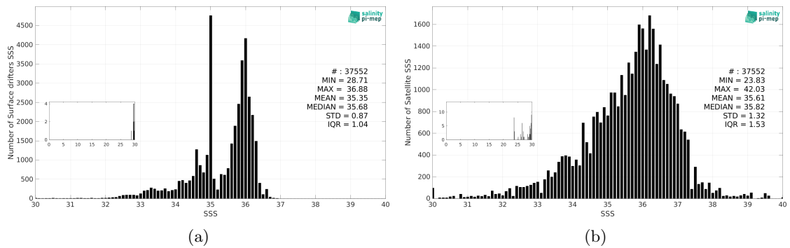
Figure 3: Histograms of SSS from Surface drifters (a) and SMAP SSS L2 v6 - 40 km (RSS) (b) considering all match-up pairs per bins of 0.1 over the North Atlantic Ocean Pi-MEP region and for the full satellite product period.
