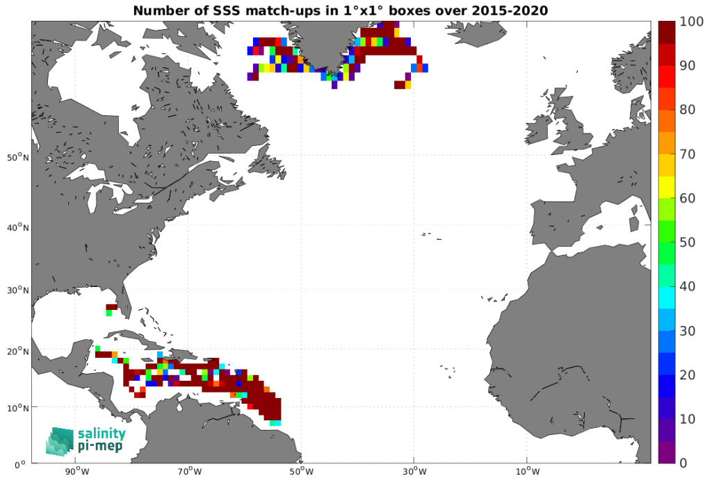
Figure 4: Number of SSS match-ups between Surface drifters SSS and the SMAP SSS L2 v6 - 40 km (RSS) SSS product for the North Atlantic Ocean Pi-MEP region over 1^\circ \times 1^\circ boxes and for the full satellite product period.
