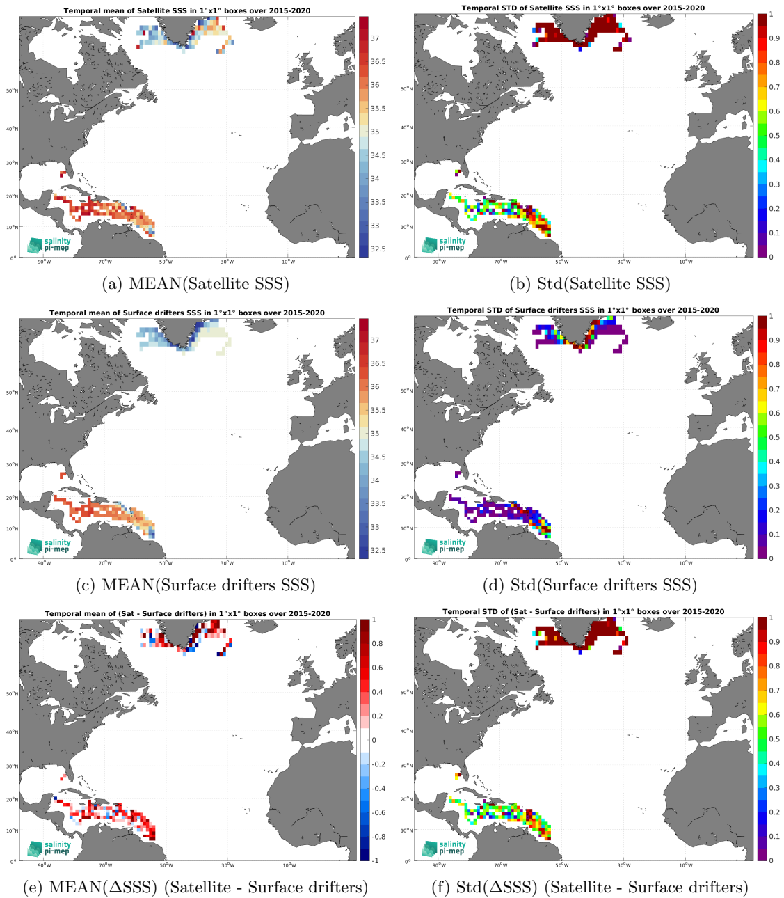
Figure 6: Temporal mean (left) and Std (right) of SSS from SMAP SSS L2 v6 - 40 km (RSS) (top), Surface drifters (middle), and of \Delta SSS (Satellite - Surface drifters). Only match-up pairs are used to generate these maps.
