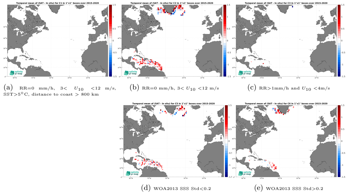
Figure 13: Temporal mean gridded over spatial boxes of size 1^\circ \times 1^\circ of \Delta\text{SSS} (SMAP SSS L2 v6 - 40 km (RSS) - Surface drifters) for 5 different subdatasets corresponding to:RR=0 mm/h, 3 < U_{10} < 12 m/s, SST >5^\circ\text{C} , distance to coast > 800 km (a), RR=0 mm/h, 3 < U_{10} < 12 m/s (b), RR >1 mm/h and U_{10} < 4 m/s (c), WOA2013 SSS Std <0.2 (d), WOA2013 SSS Std >0.2 (e).
