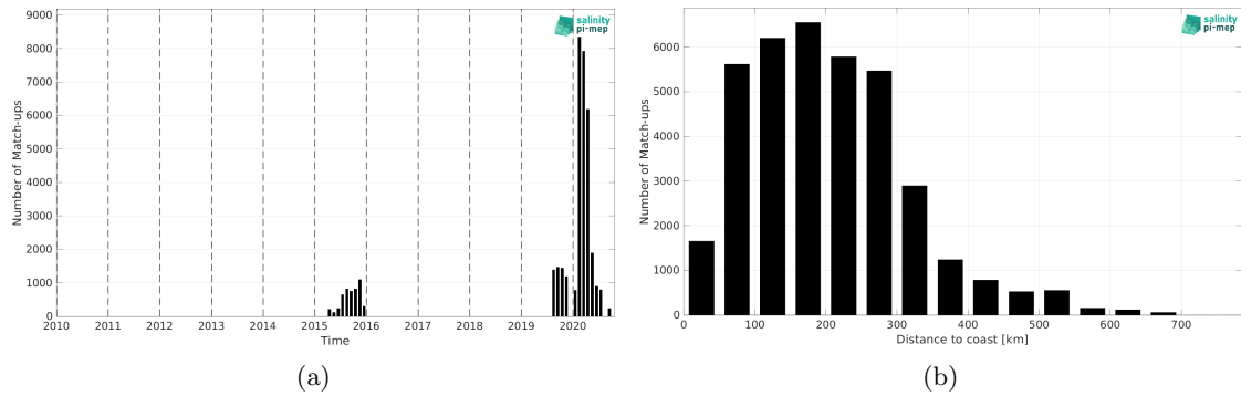
Figure 2: Number of match-ups between Surface drifters and SMAP SSS L2 v6 - 40 km (RSS) SSS as a function of time (a) and as function of the distance to coast (b) over the North Atlantic Ocean Pi-MEP region and for the full satellite product period.
