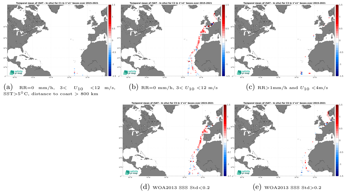
Figure 12: Temporal mean gridded over spatial boxes of size 1^\circ \times 1^\circ of \Delta\text{SSS} (SMAP SSS L2 v5 (RSS) - TSG (Polarstern)) for 5 different subdatasets corresponding to:RR=0 mm/h, 3 < U_{10} < 12 m/s, SST >5^\circ\text{C} , distance to coast > 800 km (a), RR=0 mm/h, 3 < U_{10} < 12 m/s (b), RR >1 mm/h and U_{10} < 4 m/s (c), WOA2013 SSS Std <0.2 (d), WOA2013 SSS Std >0.2 (e).
