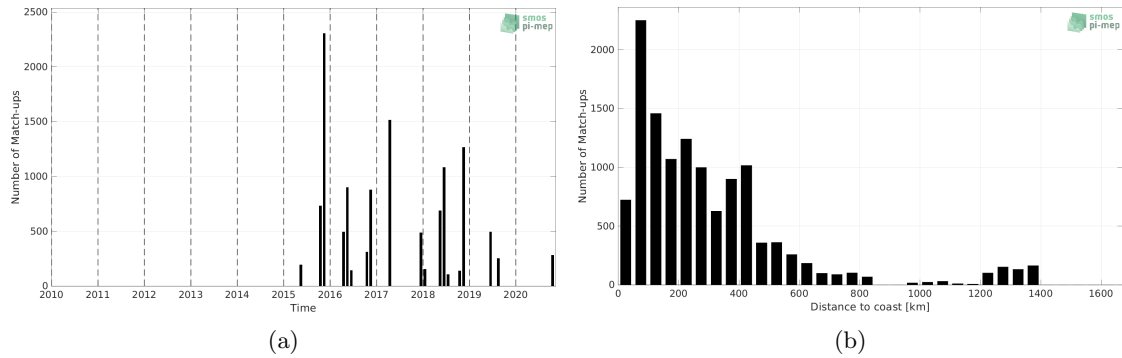
Figure 1: Number of match-ups between TSG (Polarstern) and SMAP SSS L2 v5 (RSS) SSS as a function of time (a) and as function of the distance to coast (b) over the North Atlantic Ocean Pi-MEP region and for the full satellite product period.
