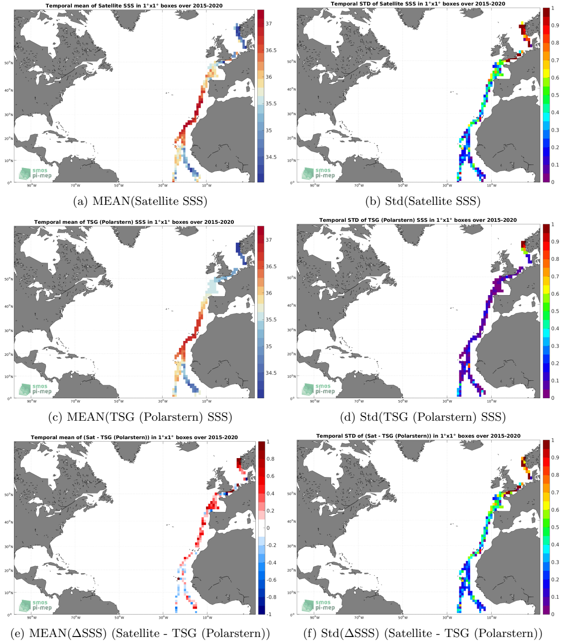
Figure 6: Temporal mean (left) and Std (right) of SSS from SMAP SSS L2 v5 (RSS) (top), TSG (Polarstern) (middle), and of \Delta SSS (Satellite - TSG (Polarstern)). Only match-up pairs are used to generate these maps.
