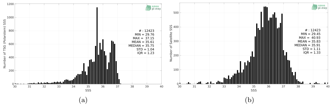
Figure 2: Histograms of SSS from TSG (Polarstern) (a) and SMAP SSS L2 v5 (RSS) (b) considering all match-up pairs per bins of 0.1 over the North Atlantic Ocean Pi-MEP region and for the full satellite product period.
