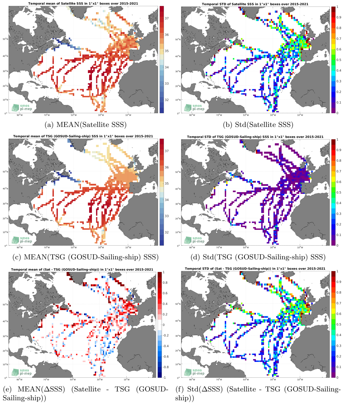
Figure 6: Temporal mean (left) and Std (right) of SSS from SMAP SSS L2 v5 (RSS) (top), TSG (GOSUD-Sailing-ship) (middle), and of \Delta SSS (Satellite - TSG (GOSUD-Sailing-ship)). Only match-up pairs are used to generate these maps.
