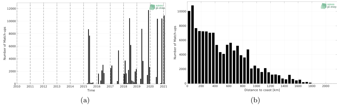
Figure 1: Number of match-ups between TSG (GOSUD-Sailing-ship) and SMAP SSS L2 v5 (RSS) SSS as a function of time (a) and as function of the distance to coast (b) over the North Atlantic Ocean Pi-MEP region and for the full satellite product period.
