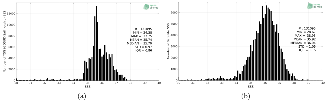
Figure 2: Histograms of SSS from TSG (GOSUD-Sailing-ship) (a) and SMAP SSS L2 v5 (RSS) (b) considering all match-up pairs per bins of 0.1 over the North Atlantic Ocean Pi-MEP region and for the full satellite product period.
