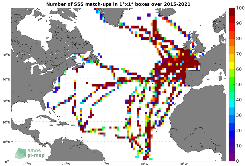
Figure 4: Number of SSS match-ups between TSG (GOSUD-Sailing-ship) SSS and the SMAP SSS L2 v5 (RSS) SSS product for the North Atlantic Ocean Pi-MEP region over 1^\circ \times 1^\circ boxes and for the full satellite product period.
