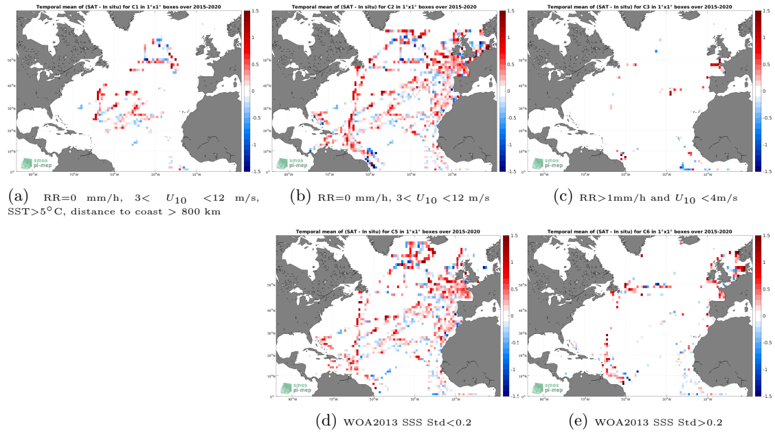
Figure 12: Temporal mean gridded over spatial boxes of size 1^\circ \times 1^\circ of \Delta\text{SSS} (SMAP SSS L2 v5 (RSS) - TSG (GOSUD-Research-vessel)) for 5 different subdatasets corresponding to:RR=0 mm/h, 3 < U_{10} < 12 m/s, SST >5^\circ\text{C} , distance to coast > 800 km (a), RR=0 mm/h, 3 < U_{10} < 12 m/s (b), RR >1 mm/h and U_{10} < 4 m/s (c), WOA2013 SSS Std <0.2 (d), WOA2013 SSS Std >0.2 (e).
