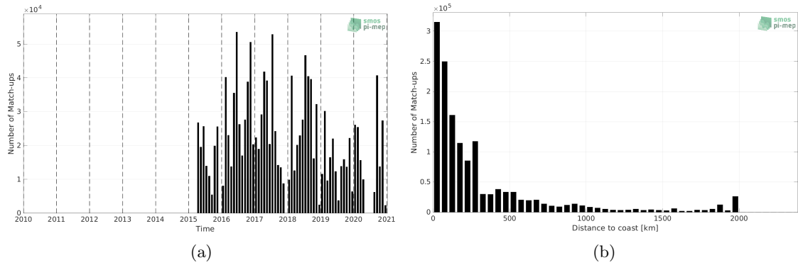
Figure 1: Number of match-ups between TSG (GOSUD-Research-vessel) and SMAP SSS L2 v5 (RSS) SSS as a function of time (a) and as function of the distance to coast (b) over the North Atlantic Ocean Pi-MEP region and for the full satellite product period.
