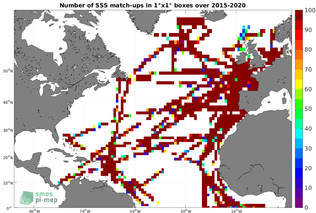
Figure 4: Number of SSS match-ups between TSG (GOSUD-Research-vessel) SSS and the SMAP SSS L2 v5 (RSS) SSS product for the North Atlantic Ocean Pi-MEP region over 1^\circ \times 1^\circ boxes and for the full satellite product period.
