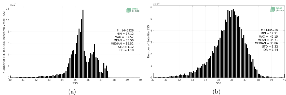
Figure 2: Histograms of SSS from TSG (GOSUD-Research-vessel) (a) and SMAP SSS L2 v5 (RSS) (b) considering all match-up pairs per bins of 0.1 over the North Atlantic Ocean Pi-MEP region and for the full satellite product period.
