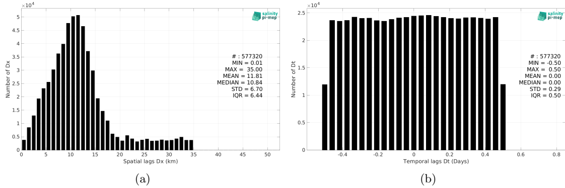
Figure 5: Histograms of the spatial (a) and temporal (b) lags between the location/time of the TSG (CSIC-UTM) measurement and the date of the corresponding SMAP SSS L2 v5 (RSS) SSS pixel.
