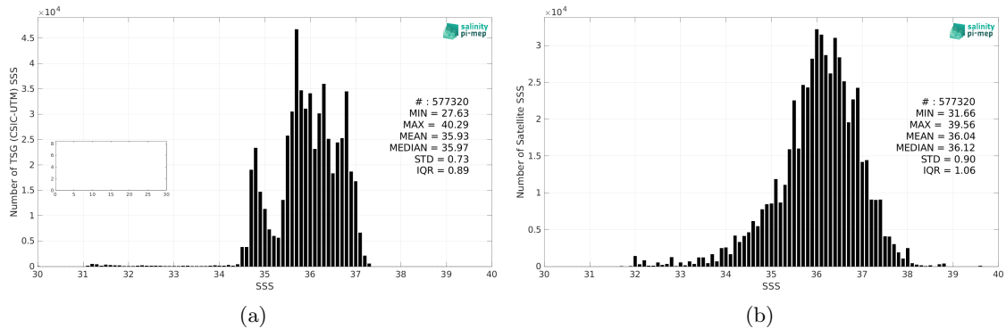
Figure 2: Histograms of SSS from TSG (CSIC-UTM) (a) and SMAP SSS L2 v5 (RSS) (b) considering all match-up pairs per bins of 0.1 over the North Atlantic Ocean Pi-MEP region and for the full satellite product period.
