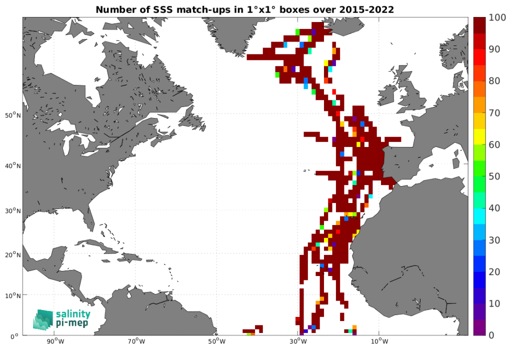
Figure 4: Number of SSS match-ups between TSG (CSIC-UTM) SSS and the SMAP SSS L2 v5 (RSS) SSS product for the North Atlantic Ocean Pi-MEP region over 1^\circ \times 1^\circ boxes and for the full satellite product period.
