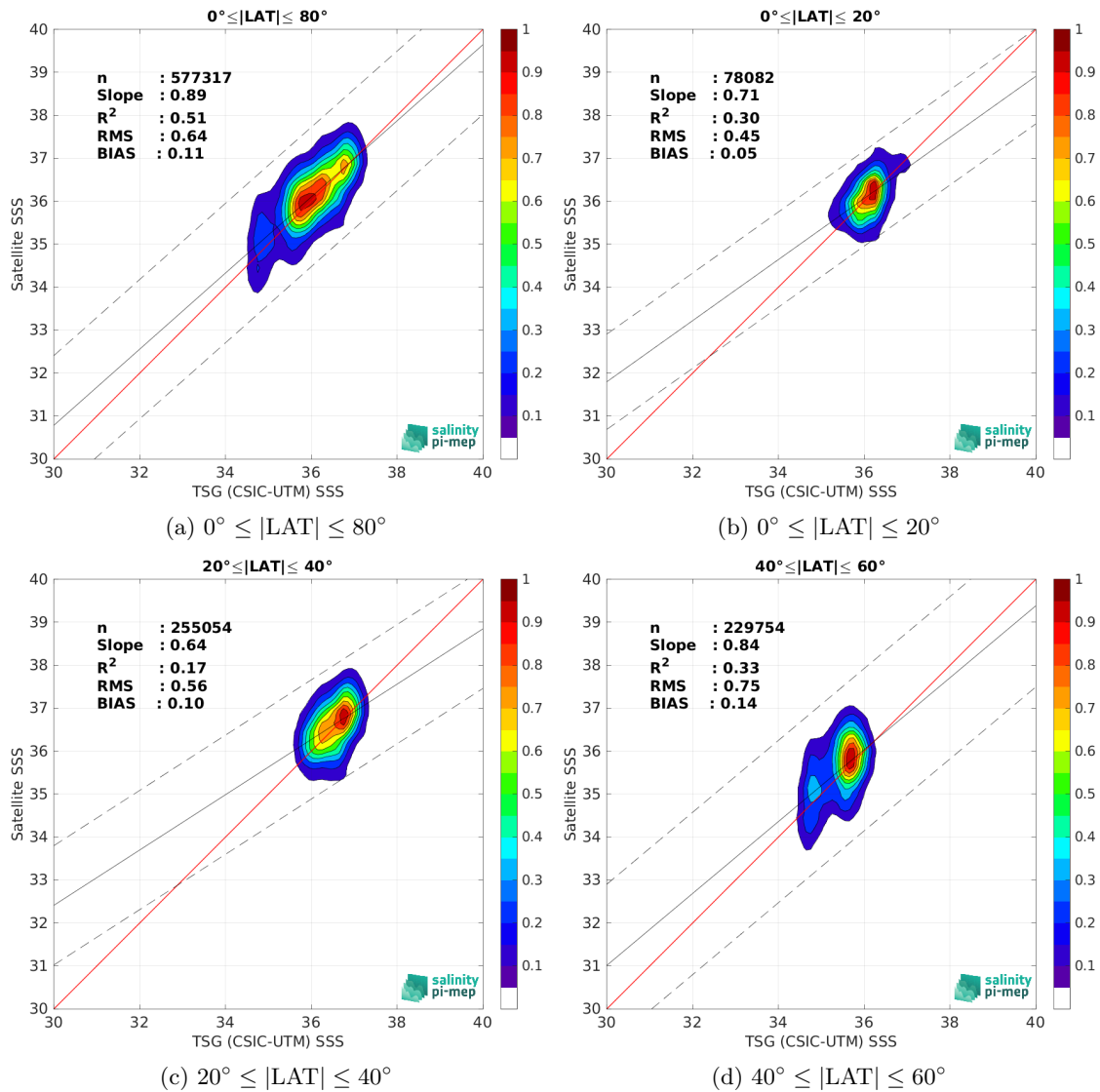
Figure 9: Contour maps of the concentration of SMAP SSS L2 v5 (RSS) SSS (y-axis) versus TSG (CSIC-UTM) SSS (x-axis) at match-up pairs for different latitude bands. For each plot, the red line shows x=y . The black thin and dashed lines indicate a linear fit through the data cloud and the \pm 95\% confidence levels, respectively. The number match-up pairs n , the slope and R^2 coefficient of the linear fit, the root mean square (RMS) and the mean bias between satellite and in situ data are indicated for each latitude band in each plots.
