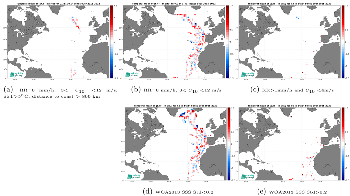
Figure 12: Temporal mean gridded over spatial boxes of size 1^\circ \times 1^\circ of \Delta SSS (SMAP SSS L2 v5 (RSS) - TSG (CSIC-UTM)) for 5 different subdatasets corresponding to:RR=0 mm/h, 3 < U_{10} < 12 m/s, SST >5^\circ C, distance to coast > 800 km (a), RR=0 mm/h, 3 < U_{10} < 12 m/s (b), RR >1 mm/h and U_{10} < 4 m/s (c), WOA2013 SSS Std <0.2 (d), WOA2013 SSS Std >0.2 (e).
