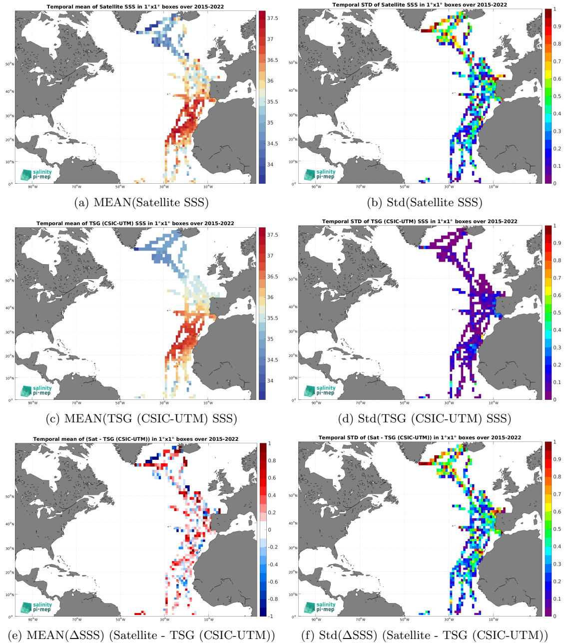
Figure 6: Temporal mean (left) and Std (right) of SSS from SMAP SSS L2 v5 (RSS) (top), TSG (CSIC-UTM) (middle), and of \Delta SSS (Satellite - TSG (CSIC-UTM)). Only match-up pairs are used to generate these maps.
