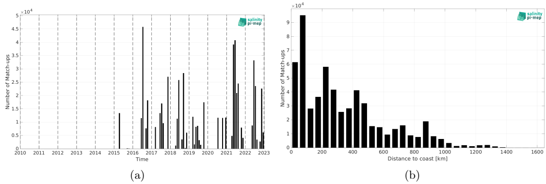
Figure 1: Number of match-ups between TSG (CSIC-UTM) and SMAP SSS L2 v5 (RSS) SSS as a function of time (a) and as function of the distance to coast (b) over the North Atlantic Ocean Pi-MEP region and for the full satellite product period.
