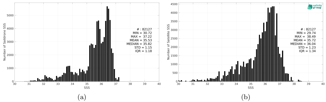
Figure 2: Histograms of SSS from Sairdron (a) and SMAP SSS L2 v5 (RSS) (b) considering all match-up pairs per bins of 0.1 over the North Atlantic Ocean Pi-MEP region and for the full satellite product period.
