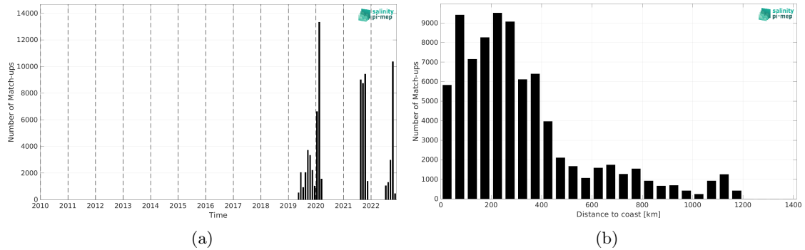
Figure 1: Number of match-ups between Sairdron and SMAP SSS L2 v5 (RSS) SSS as a function of time (a) and as function of the distance to coast (b) over the North Atlantic Ocean Pi-MEP region and for the full satellite product period.
