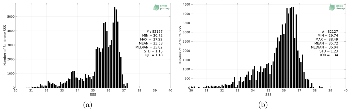
Figure 2: Histograms of SSS from Sairdrone (a) and SMAP SSS L2 v5 (RSS) (b) considering all match-up pairs per bins of 0.1 over the North Atlantic Ocean Pi-MEP region and for the full satellite product period.
