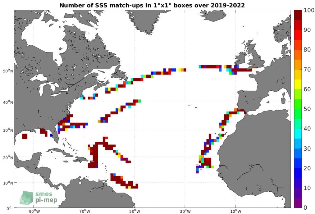
Figure 4: Number of SSS match-ups between Saildrone SSS and the SMAP SSS L2 v5 (RSS) SSS product for the North Atlantic Ocean Pi-MEP region over 1^\circ \times 1^\circ boxes and for the full satellite product period.
