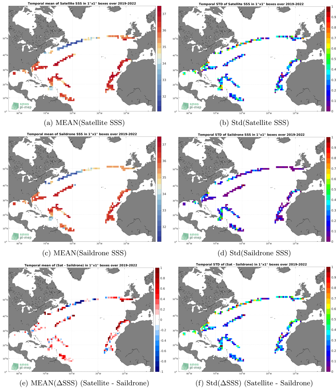
Figure 6: Temporal mean (left) and Std (right) of SSS from SMAP SSS L2 v5 (RSS) (top), Saildrone (middle), and of \Delta SSS (Satellite - Saildrone). Only match-up pairs are used to generate these maps.
