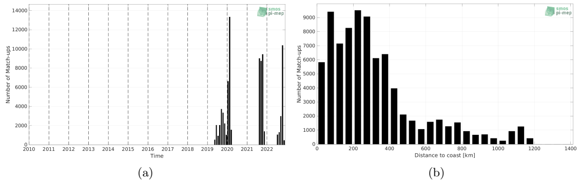
Figure 1: Number of match-ups between Sairdrone and SMAP SSS L2 v5 (RSS) SSS as a function of time (a) and as function of the distance to coast (b) over the North Atlantic Ocean Pi-MEP region and for the full satellite product period.
