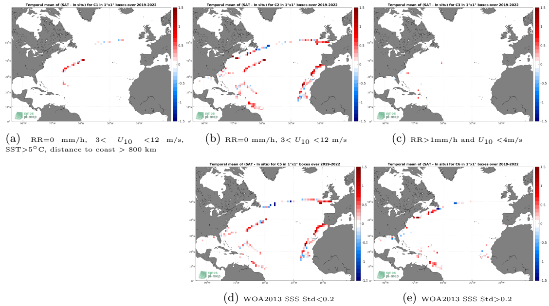
Figure 12: Temporal mean gridded over spatial boxes of size 1^\circ \times 1^\circ of \Delta SSS (SMAP SSS L2 v5 (RSS) - Saildrone) for 5 different subdatasets corresponding to:RR=0 mm/h, 3 < U_{10} < 12 m/s, SST >5^\circ\text{C} , distance to coast > 800 km (a), RR=0 mm/h, 3 < U_{10} < 12 m/s (b), RR >1 mm/h and U_{10} < 4 m/s (c), WOA2013 SSS Std <0.2 (d), WOA2013 SSS Std >0.2 (e).
