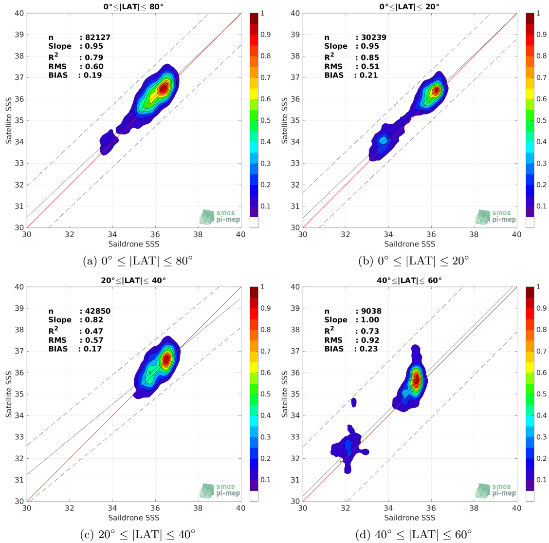
Figure 9: Contour maps of the concentration of SMAP SSS L2 v5 (RSS) SSS (y-axis) versus Saildrone SSS (x-axis) at match-up pairs for different latitude bands. For each plot, the red line shows x=y . The black thin and dashed lines indicate a linear fit through the data cloud and the \pm 95\% confidence levels, respectively. The number match-up pairs n , the slope and R^2 coefficient of the linear fit, the root mean square (RMS) and the mean bias between satellite and in situ data are indicated for each latitude band in each plots.
