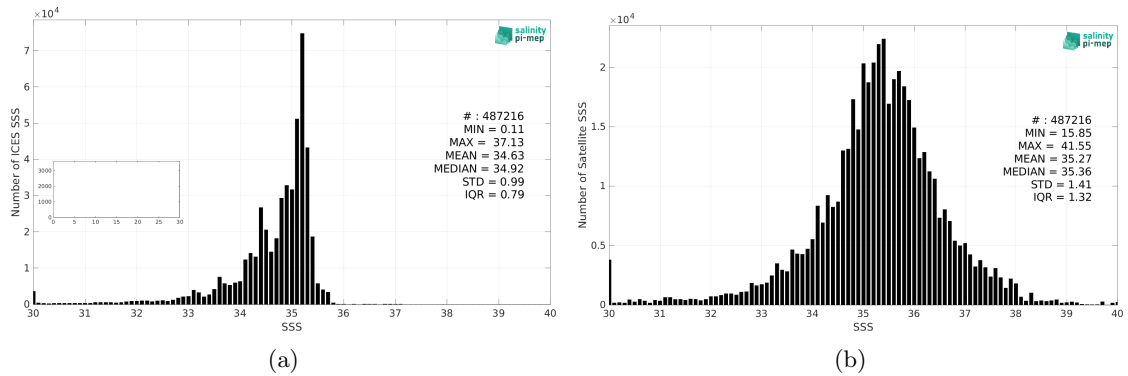
Figure 2: Histograms of SSS from ICES (a) and SMAP SSS L2 v5 (RSS) (b) considering all match-up pairs per bins of 0.1 over the North Atlantic Ocean Pi-MEP region and for the full satellite product period.
