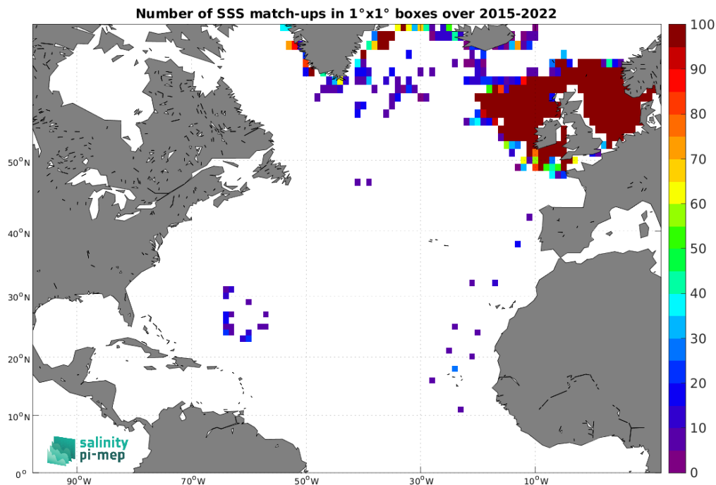
Figure 4: Number of SSS match-ups between ICES SSS and the SMAP SSS L2 v5 (RSS) SSS product for the North Atlantic Ocean Pi-MEP region over 1^\circ \times 1^\circ boxes and for the full satellite product period.
