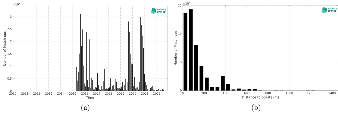
Figure 1: Number of match-ups between ICES and SMAP SSS L2 v5 (RSS) SSS as a function of time (a) and as function of the distance to coast (b) over the North Atlantic Ocean Pi-MEP region and for the full satellite product period.
