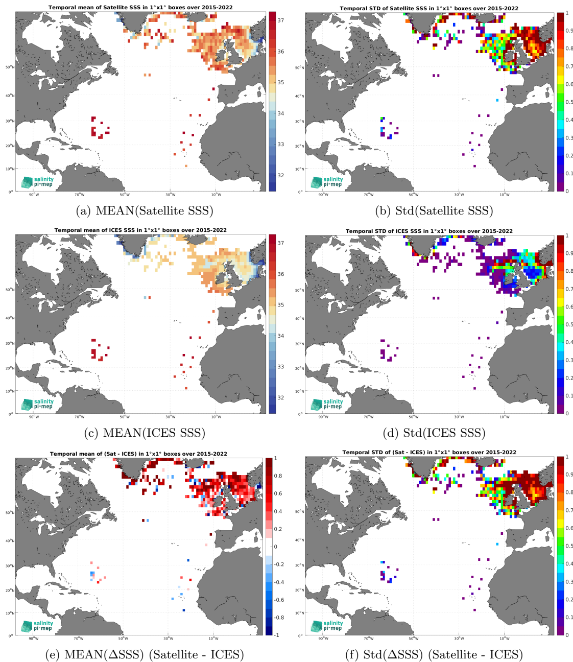
Figure 6: Temporal mean (left) and Std (right) of SSS from SMAP SSS L2 v5 (RSS) (top), ICES (middle), and of \Delta SSS (Satellite - ICES). Only match-up pairs are used to generate these maps.
