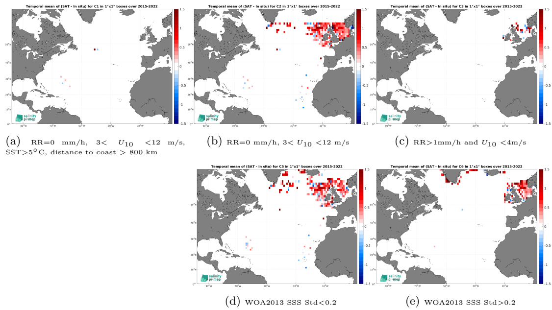
Figure 12: Temporal mean gridded over spatial boxes of size 1^\circ \times 1^\circ of \Delta SSS (SMAP SSS L2 v5 (RSS) - ICES) for 5 different subdatasets corresponding to: RR=0 mm/h, 3 < U_{10} < 12 m/s, SST > 5^\circ\text{C} , distance to coast > 800 km (a), RR=0 mm/h, 3 < U_{10} < 12 m/s (b), RR > 1 mm/h and U_{10} < 4 m/s (c), WOA2013 SSS Std < 0.2 (d), WOA2013 SSS Std > 0.2 (e).
