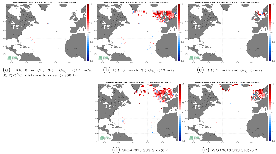
Figure 12: Temporal mean gridded over spatial boxes of size 1^\circ \times 1^\circ of \Delta SSS (SMAP SSS L2 v5 (RSS) - ICES) for 5 different subdatasets corresponding to:RR=0 mm/h, 3 < U_{10} < 12 m/s, SST >5^\circ C, distance to coast > 800 km (a), RR=0 mm/h, 3 < U_{10} < 12 m/s (b), RR >1 mm/h and U_{10} < 4 m/s (c), WOA2013 SSS Std <0.2 (d), WOA2013 SSS Std >0.2 (e).
