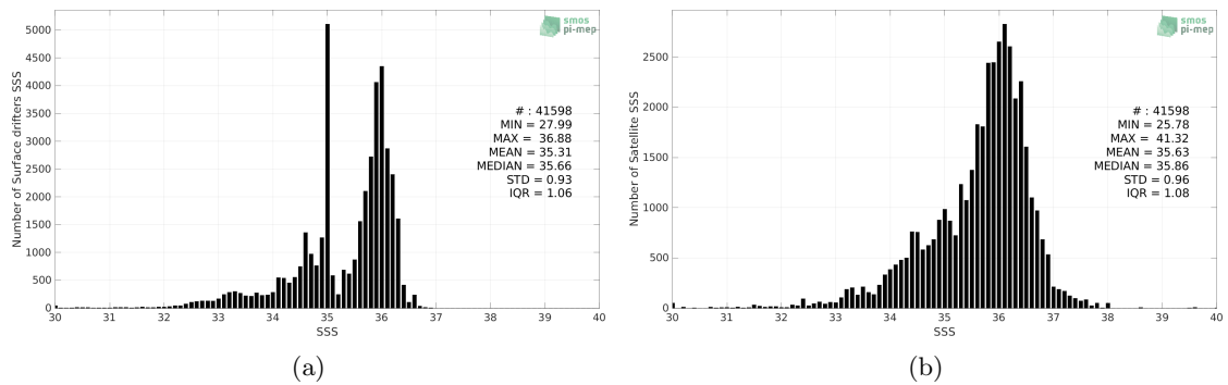
Figure 2: Histograms of SSS from Surface drifters (a) and SMAP SSS L2 v5 (RSS) (b) considering all match-up pairs per bins of 0.1 over the North Atlantic Ocean Pi-MEP region and for the full satellite product period.
