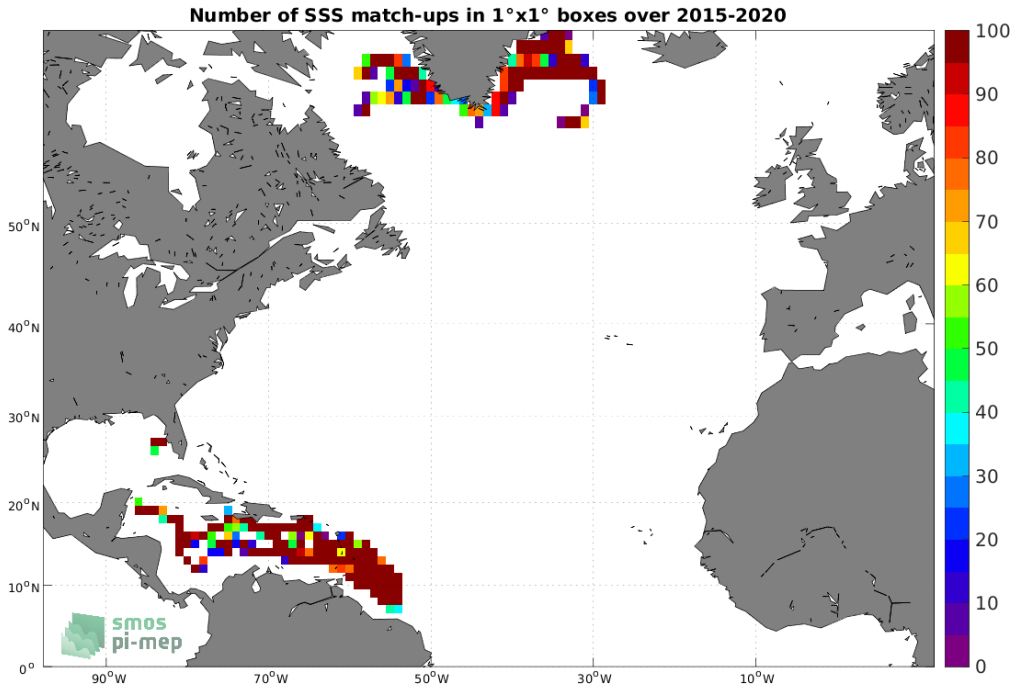
Figure 3: Number of SSS match-ups between Surface drifters SSS and the SMAP SSS L2 v5 (RSS) SSS product for the North Atlantic Ocean Pi-MEP region over 1^\circ \times 1^\circ boxes and for the full satellite product period.
