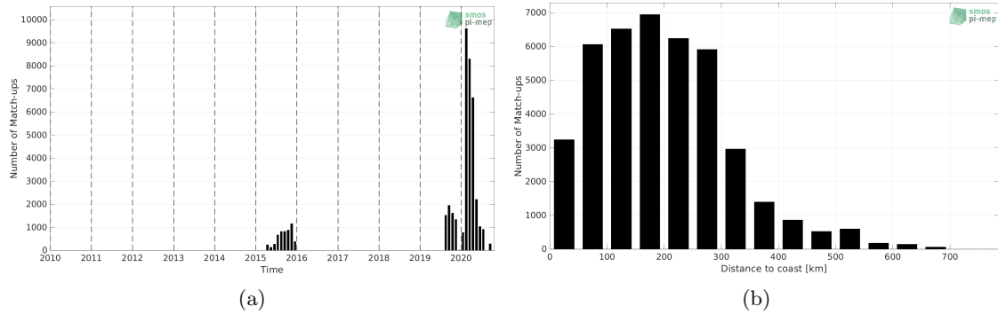
Figure 1: Number of match-ups between Surface drifters and SMAP SSS L2 v5 (RSS) SSS as a function of time (a) and as function of the distance to coast (b) over the North Atlantic Ocean Pi-MEP region and for the full satellite product period.
