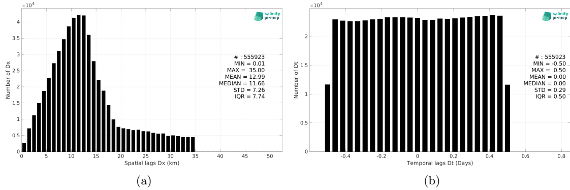
Figure 6: Histograms of the spatial (a) and temporal (b) lags between the location/time of the TSG (SAMOS) measurement and the date of the corresponding SMAP SSS L2 v5.3 (RSS) SSS pixel.
