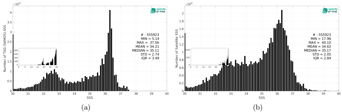
Figure 3: Histograms of SSS from TSG (SAMOS) (a) and SMAP SSS L2 v5.3 (RSS) (b) considering all match-up pairs per bins of 0.1 over the North Atlantic Ocean Pi-MEP region and for the full satellite product period.
