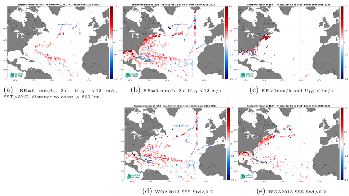
Figure 14: Temporal mean gridded over spatial boxes of size 1^\circ \times 1^\circ of \Delta\text{SSS} (SMAP SSS L2 v5.3 (RSS) - TSG (SAMOS)) for 5 different subdatasets corresponding to:RR=0 mm/h, 3 < U_{10} < 12 m/s, SST >5^\circ\text{C} , distance to coast > 800 km (a), RR=0 mm/h, 3 < U_{10} < 12 m/s (b), RR >1 mm/h and U_{10} < 4 m/s (c), WOA2013 SSS Std <0.2 (d), WOA2013 SSS Std >0.2 (e).
