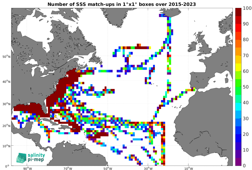
Figure 5: Number of SSS match-ups between TSG (SAMOS) SSS and the SMAP SSS L2 v5.3 (RSS) SSS product for the North Atlantic Ocean Pi-MEP region over 1^\circ \times 1^\circ boxes and for the full satellite product period.
