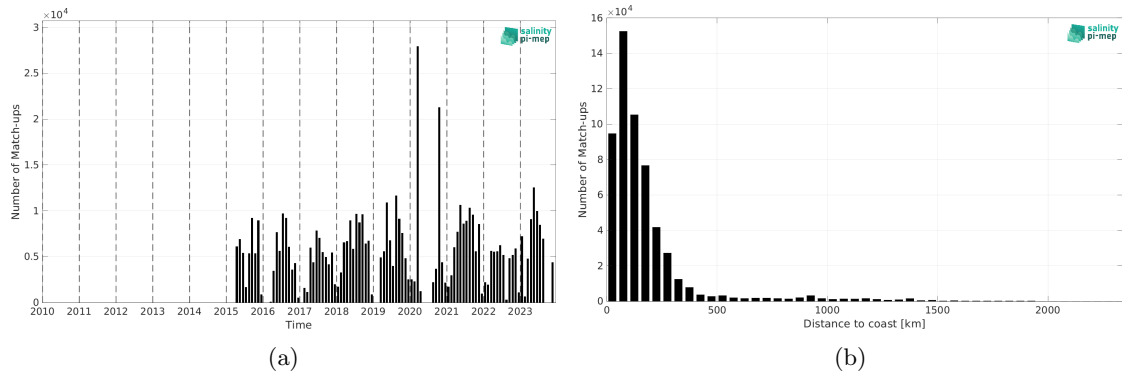
Figure 2: Number of match-ups between TSG (SAMOS) and SMAP SSS L2 v5.3 (RSS) SSS as a function of time (a) and as function of the distance to coast (b) over the North Atlantic Ocean Pi-MEP region and for the full satellite product period.
