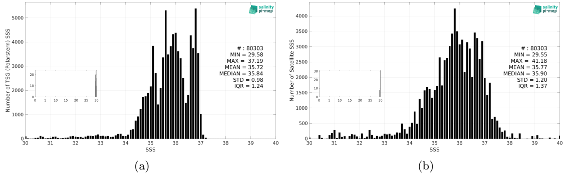
Figure 3: Histograms of SSS from TSG (Polarstern) (a) and SMAP SSS L2 v5.3 (RSS) (b) considering all match-up pairs per bins of 0.1 over the North Atlantic Ocean Pi-MEP region and for the full satellite product period.
