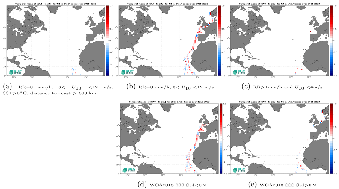
Figure 14: Temporal mean gridded over spatial boxes of size 1^\circ \times 1^\circ of \Delta SSS (SMAP SSS L2 v5.3 (RSS) - TSG (Polarstern)) for 5 different subdatasets corresponding to:RR=0 mm/h, 3 < U_{10} < 12 m/s, SST>5°C, distance to coast > 800 km (a), RR=0 mm/h, 3 < U_{10} < 12 m/s (b), RR>1mm/h and U_{10} < 4 m/s (c), WOA2013 SSS Std<0.2 (d), WOA2013 SSS Std>0.2 (e).
