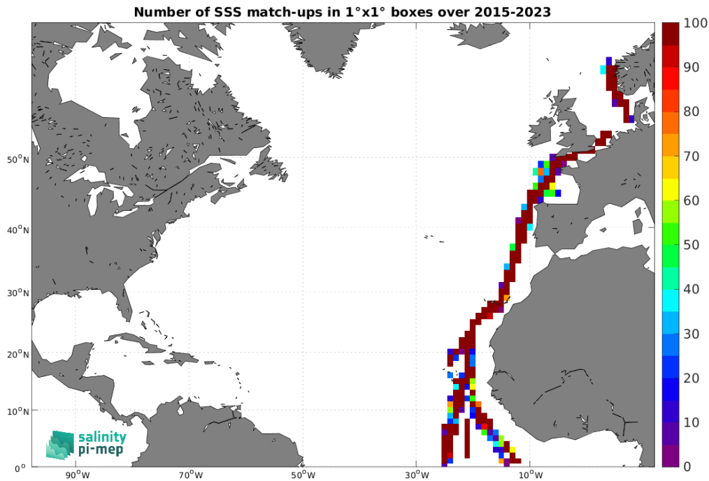
Figure 5: Number of SSS match-ups between TSG (Polarstern) SSS and the SMAP SSS L2 v5.3 (RSS) SSS product for the North Atlantic Ocean Pi-MEP region over 1^\circ \times 1^\circ boxes and for the full satellite product period.
