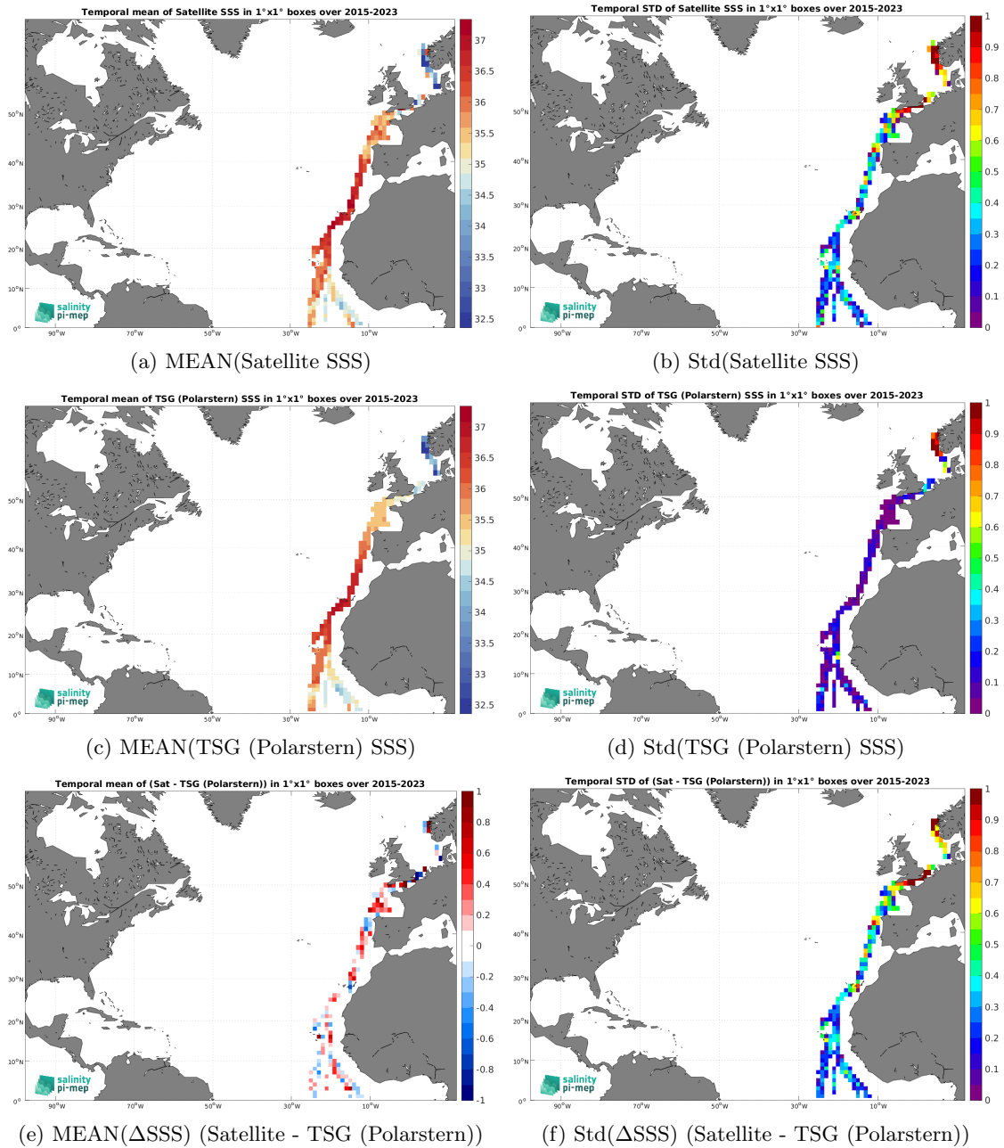
Figure 7: Temporal mean (left) and Std (right) of SSS from SMAP SSS L2 v5.3 (RSS) (top), TSG (Polarstern) (middle), and of \Delta SSS (Satellite - TSG (Polarstern)). Only match-up pairs are used to generate these maps.
