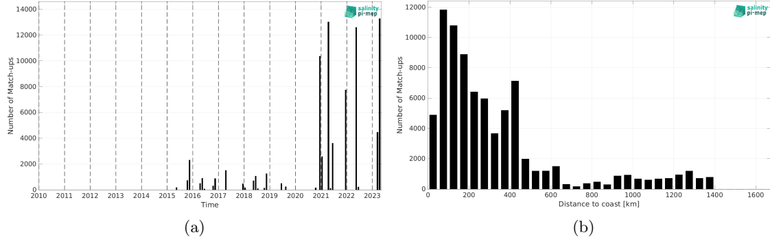
Figure 2: Number of match-ups between TSG (Polarstern) and SMAP SSS L2 v5.3 (RSS) SSS as a function of time (a) and as function of the distance to coast (b) over the North Atlantic Ocean Pi-MEP region and for the full satellite product period.
