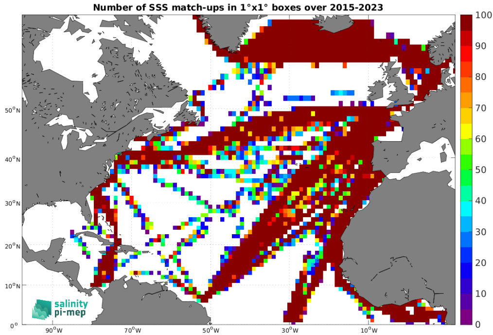
Figure 5: Number of SSS match-ups between TSG (LEGOS-DM) SSS and the SMAP SSS L2 v5.3 (RSS) SSS product for the North Atlantic Ocean Pi-MEP region over 1°x1° boxes and for the full satellite product period.
