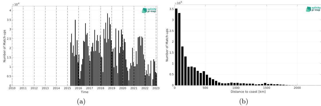
Figure 2: Number of match-ups between TSG (LEGOS-DM) and SMAP SSS L2 v5.3 (RSS) SSS as a function of time (a) and as function of the distance to coast (b) over the North Atlantic Ocean Pi-MEP region and for the full satellite product period.
