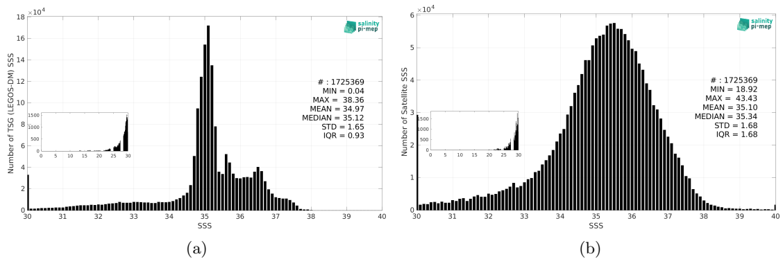
Figure 3: Histograms of SSS from TSG (LEGOS-DM) (a) and SMAP SSS L2 v5.3 (RSS) (b) considering all match-up pairs per bins of 0.1 over the North Atlantic Ocean Pi-MEP region and for the full satellite product period.
