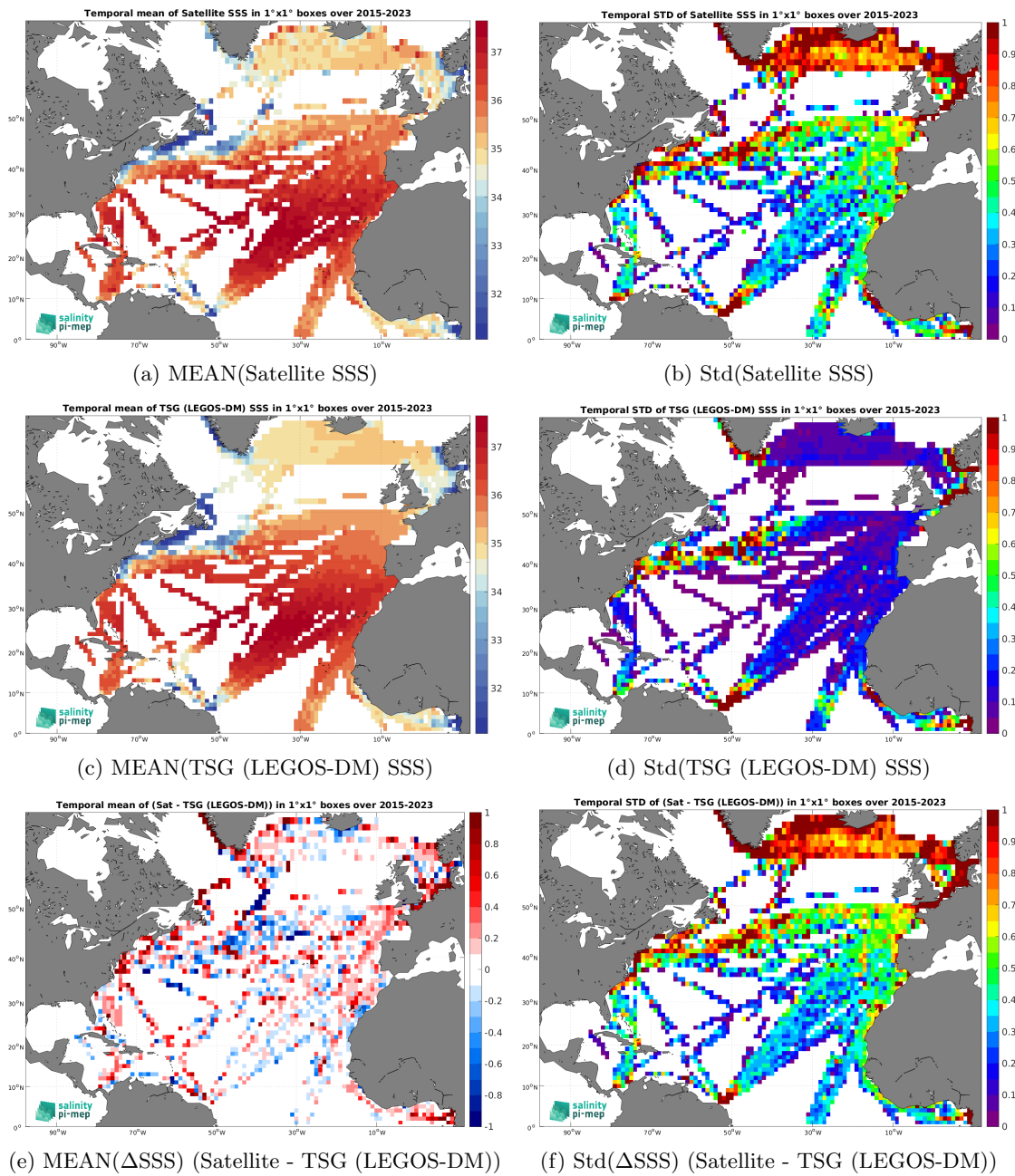
Figure 7: Temporal mean (left) and Std (right) of SSS from SMAP SSS L2 v5.3 (RSS) (top), TSG (LEGOS-DM) (middle), and of \Delta SSS (Satellite - TSG (LEGOS-DM)). Only match-up pairs are used to generate these maps.
