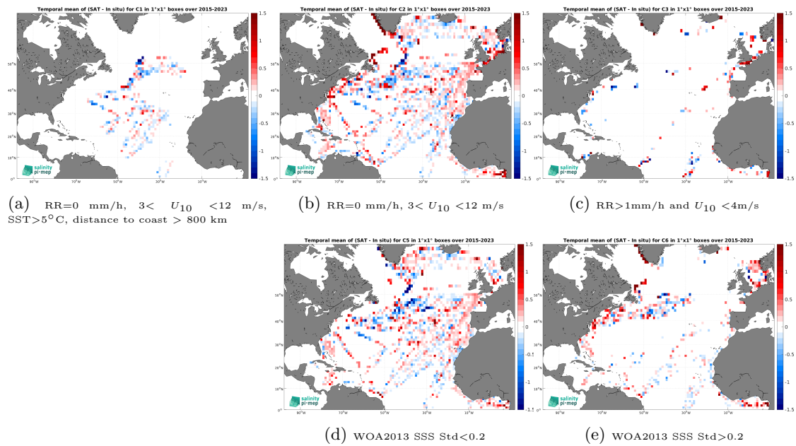
Figure 14: Temporal mean gridded over spatial boxes of size 1^\circ \times 1^\circ of \Delta\text{SSS} (SMAP SSS L2 v5.3 (RSS) - TSG (LEGOS-DM)) for 5 different subdatasets corresponding to:RR=0 mm/h, 3 < U_{10} < 12 m/s, SST > 5°C, distance to coast > 800 km (a), RR=0 mm/h, 3 < U_{10} < 12 m/s (b), RR > 1mm/h and U_{10} < 4 m/s (c), WOA2013 SSS Std < 0.2 (d), WOA2013 SSS Std > 0.2 (e).
