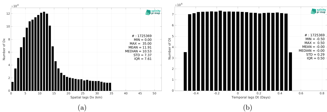
Figure 6: Histograms of the spatial (a) and temporal (b) lags between the location/time of the TSG (LEGOS-DM) measurement and the date of the corresponding SMAP SSS L2 v5.3 (RSS) SSS pixel.
