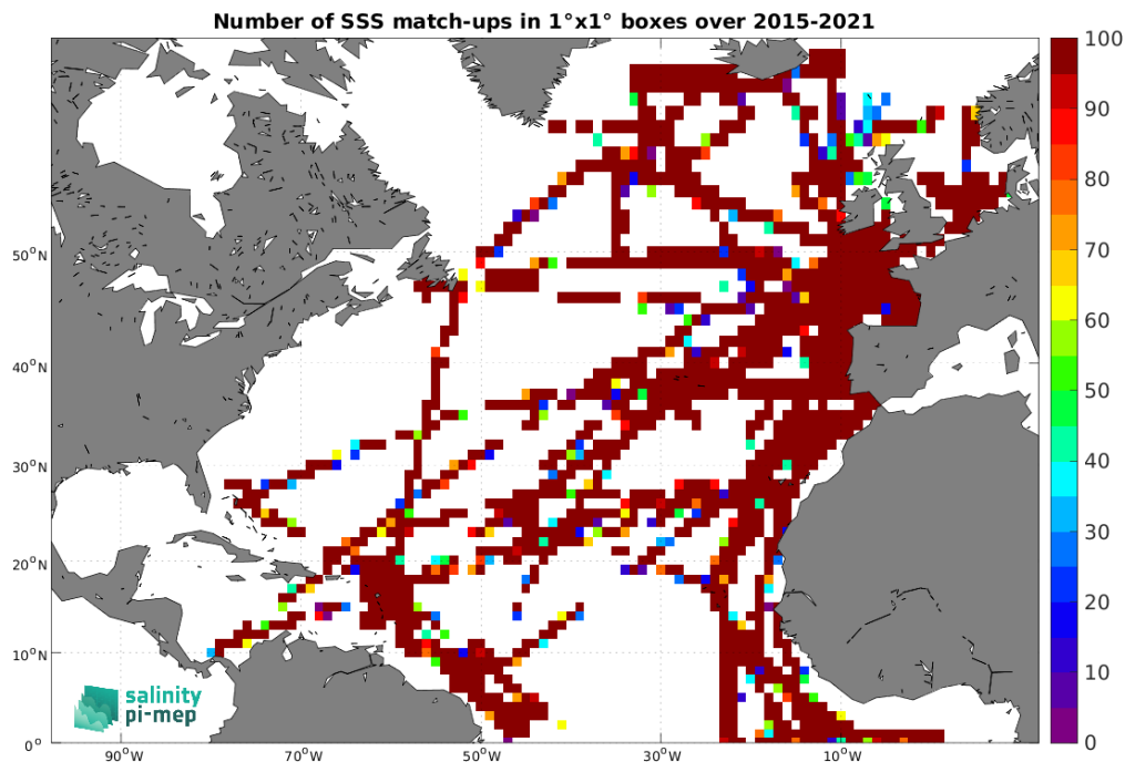
Figure 5: Number of SSS match-ups between TSG (GOSUD-Research-vessel) SSS and the SMAP SSS L2 v5.3 (RSS) SSS product for the North Atlantic Ocean Pi-MEP region over 1^\circ \times 1^\circ boxes and for the full satellite product period.
