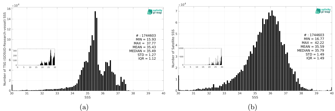
Figure 3: Histograms of SSS from TSG (GOSUD-Research-vessel) (a) and SMAP SSS L2 v5.3 (RSS) (b) considering all match-up pairs per bins of 0.1 over the North Atlantic Ocean Pi-MEP region and for the full satellite product period.
