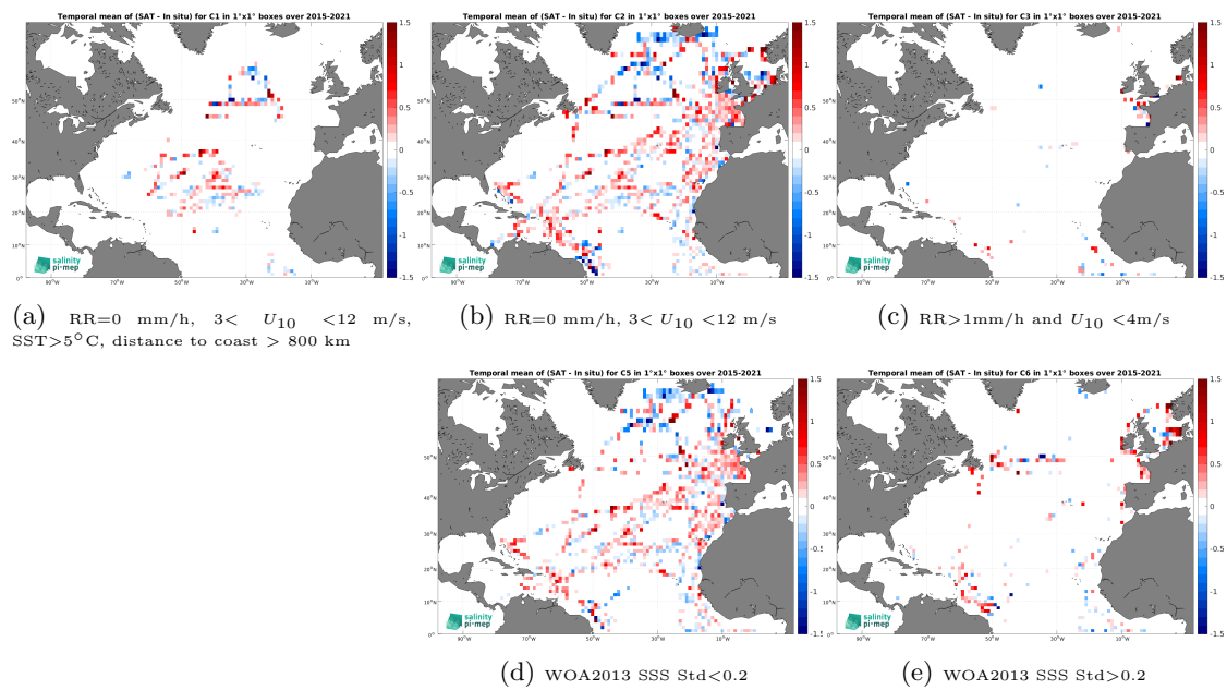
Figure 14: Temporal mean gridded over spatial boxes of size 1^\circ \times 1^\circ of \Delta\text{SSS} (SMAP SSS L2 v5.3 (RSS) - TSG (GOSUD-Research-vessel)) for 5 different subdatasets corresponding to:RR=0 mm/h, 3 < U_{10} < 12 m/s, SST >5^\circ\text{C} , distance to coast > 800 km (a), RR=0 mm/h, 3 < U_{10} < 12 m/s (b), RR >1 mm/h and U_{10} < 4 m/s (c), WOA2013 SSS Std <0.2 (d), WOA2013 SSS Std >0.2 (e).
