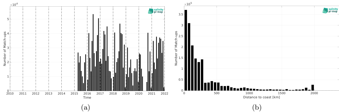
Figure 2: Number of match-ups between TSG (GOSUD-Research-vessel) and SMAP SSS L2 v5.3 (RSS) SSS as a function of time (a) and as function of the distance to coast (b) over the North Atlantic Ocean Pi-MEP region and for the full satellite product period.
