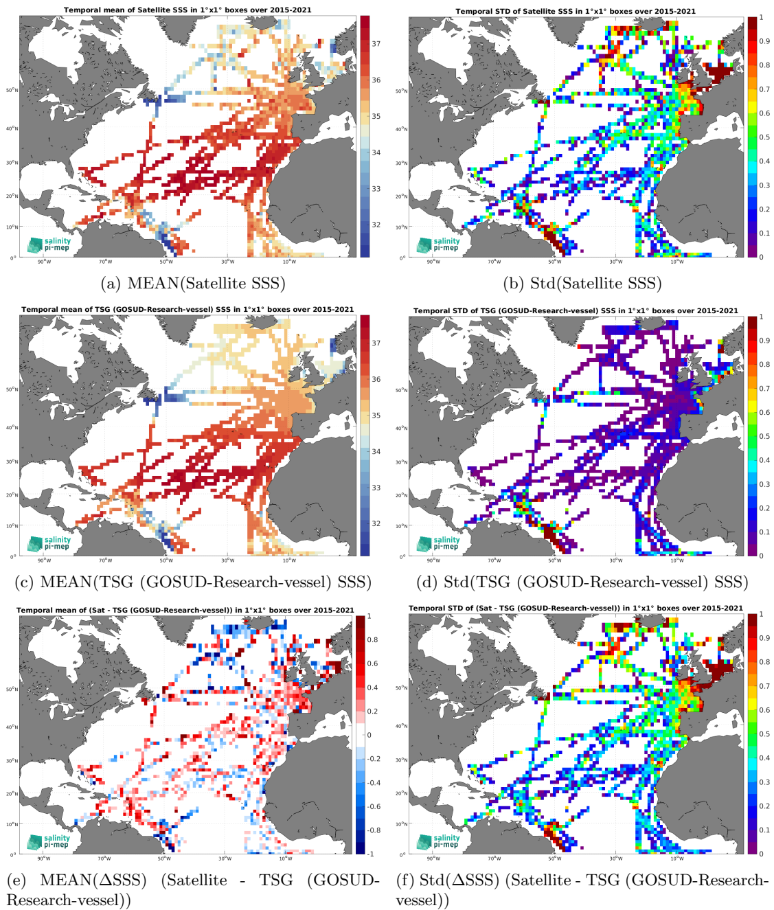
Figure 7: Temporal mean (left) and Std (right) of SSS from SMAP SSS L2 v5.3 (RSS) (top), TSG (GOSUD-Research-vessel) (middle), and of \Delta SSS (Satellite - TSG (GOSUD-Research-vessel)). Only match-up pairs are used to generate these maps.
