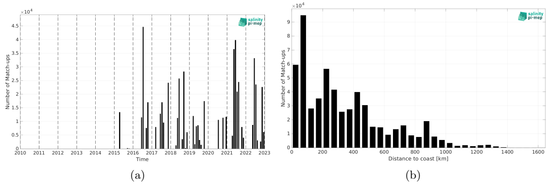
Figure 2: Number of match-ups between TSG (CSIC-UTM) and SMAP SSS L2 v5.3 (RSS) SSS as a function of time (a) and as function of the distance to coast (b) over the North Atlantic Ocean Pi-MEP region and for the full satellite product period.
