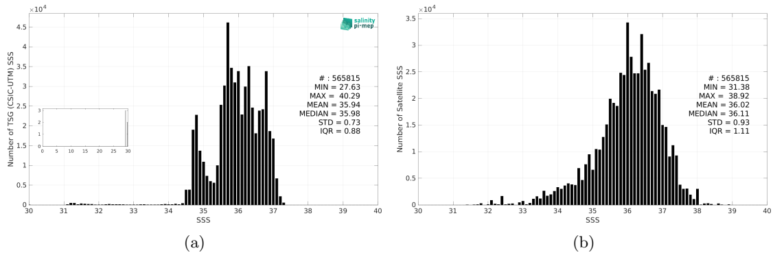
Figure 3: Histograms of SSS from TSG (CSIC-UTM) (a) and SMAP SSS L2 v5.3 (RSS) (b) considering all match-up pairs per bins of 0.1 over the North Atlantic Ocean Pi-MEP region and for the full satellite product period.
