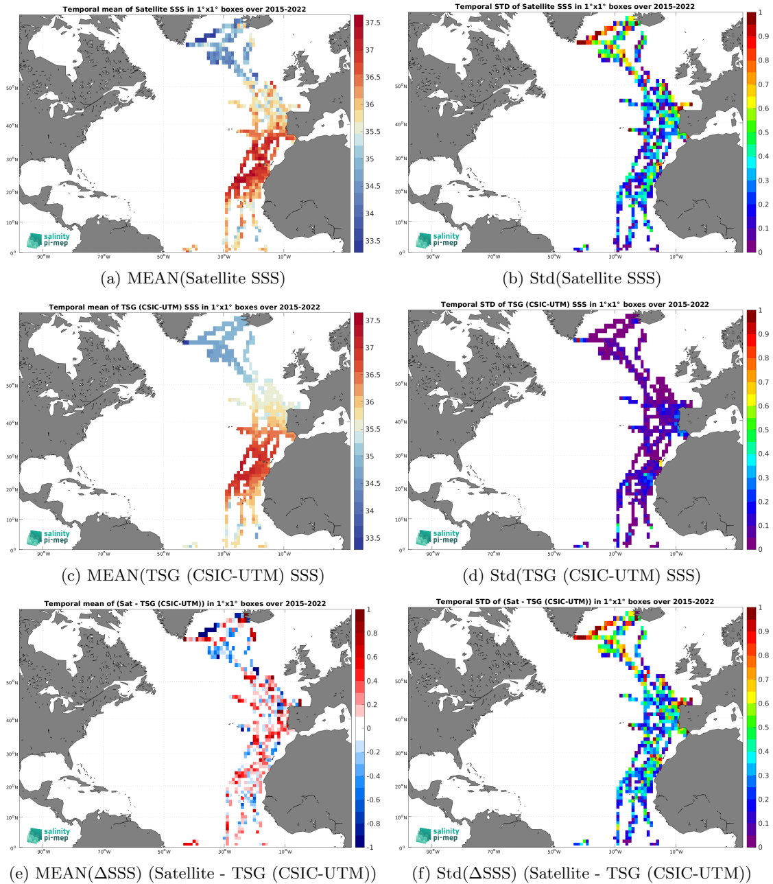
Figure 7: Temporal mean (left) and Std (right) of SSS from SMAP SSS L2 v5.3 (RSS), TSG (CSIC-UTM) (middle), and of \Delta SSS (Satellite - TSG (CSIC-UTM)). Only match-up pairs are used to generate these maps.
