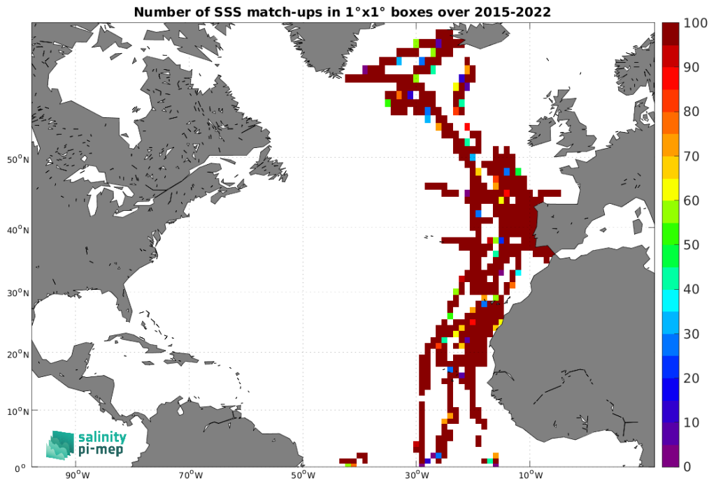
Figure 5: Number of SSS match-ups between TSG (CSIC-UTM) SSS and the SMAP SSS L2 v5.3 (RSS) SSS product for the North Atlantic Ocean Pi-MEP region over 1^\circ \times 1^\circ boxes and for the full satellite product period.
