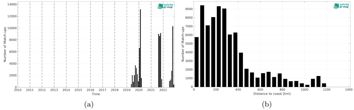
Figure 2: Number of match-ups between Saildrone and SMAP SSS L2 v5.3 (RSS) SSS as a function of time (a) and as function of the distance to coast (b) over the North Atlantic Ocean Pi-MEP region and for the full satellite product period.
