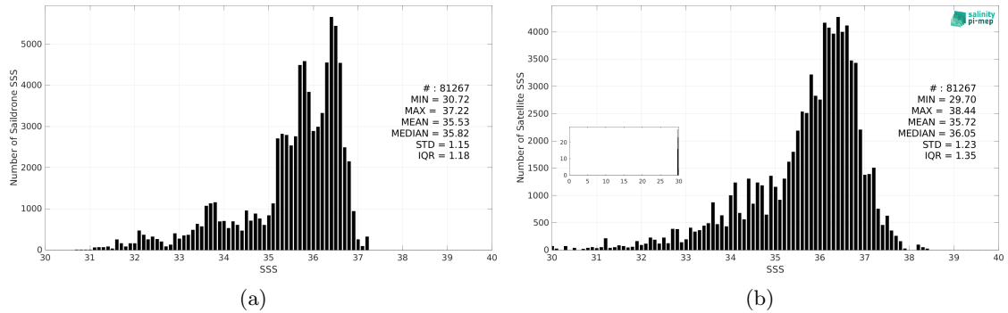
Figure 3: Histograms of SSS from Saildrone (a) and SMAP SSS L2 v5.3 (RSS) (b) considering all match-up pairs per bins of 0.1 over the North Atlantic Ocean Pi-MEP region and for the full satellite product period.
