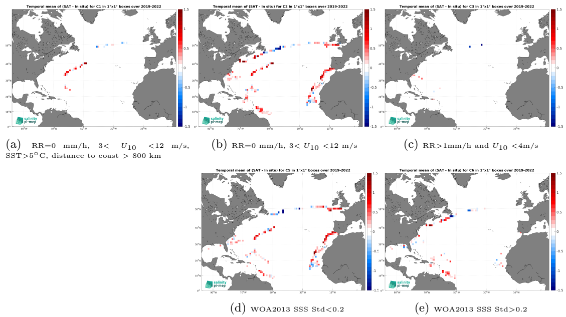
Figure 14: Temporal mean gridded over spatial boxes of size 1^\circ \times 1^\circ of \Delta SSS (SMAP SSS L2 v5.3 (RSS) - Saildrone) for 5 different subdatasets corresponding to:RR=0 mm/h, 3 < U_{10} < 12 m/s, SST>5°C, distance to coast > 800 km (a), RR=0 mm/h, 3 < U_{10} < 12 m/s (b), RR>1mm/h and U_{10} < 4 m/s (c), WOA2013 SSS Std<0.2 (d), WOA2013 SSS Std>0.2 (e).
