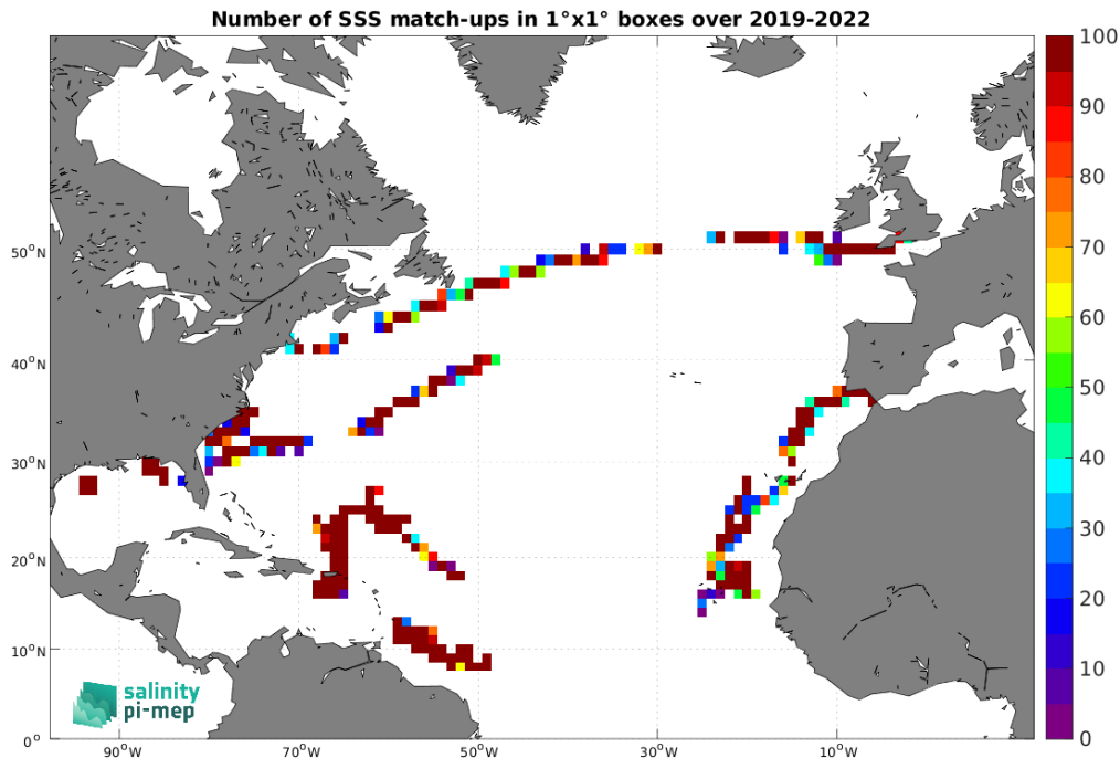
Figure 5: Number of SSS match-ups between Saildrone SSS and the SMAP SSS L2 v5.3 (RSS) SSS product for the North Atlantic Ocean Pi-MEP region over 1^\circ \times 1^\circ boxes and for the full satellite product period.
