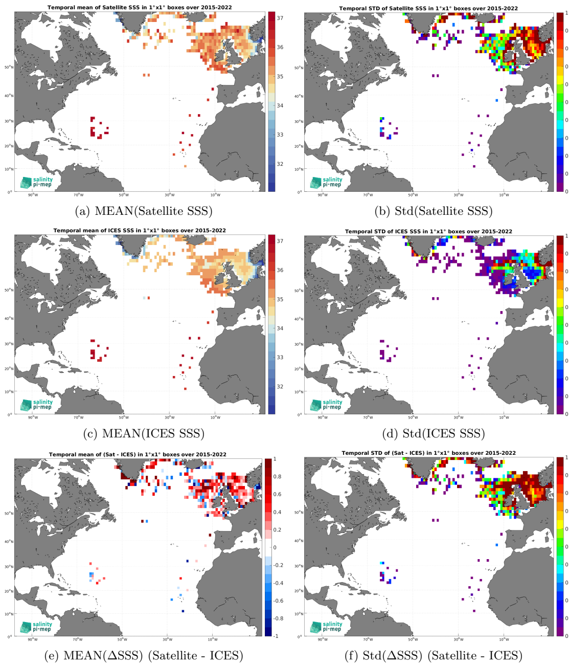
Figure 7: Temporal mean (left) and Std (right) of SSS from SMAP SSS L2 v5.3 (RSS) (top), ICES (middle), and of \Delta SSS (Satellite - ICES). Only match-up pairs are used to generate these maps.
