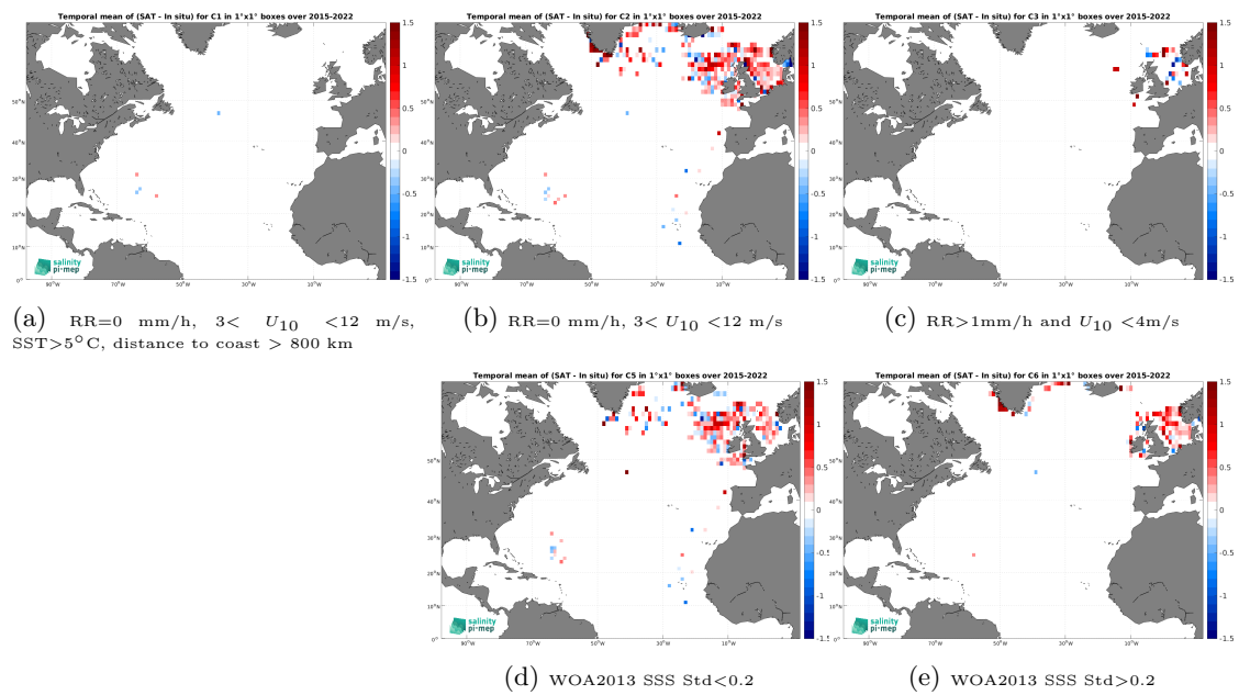
Figure 14: Temporal mean gridded over spatial boxes of size 1^\circ \times 1^\circ of \Delta SSS (SMAP SSS L2 v5.3 (RSS) - ICES) for 5 different subdatasets corresponding to:RR=0 mm/h, 3 < U_{10} < 12 m/s, SST>5°C, distance to coast > 800 km (a), RR=0 mm/h, 3 < U_{10} < 12 m/s (b), RR>1mm/h and U_{10} < 4 m/s (c), WOA2013 SSS Std<0.2 (d), WOA2013 SSS Std>0.2 (e).
