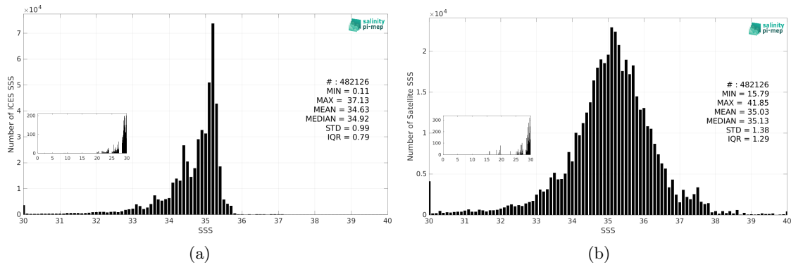
Figure 3: Histograms of SSS from ICES (a) and SMAP SSS L2 v5.3 (RSS) (b) considering all match-up pairs per bins of 0.1 over the North Atlantic Ocean Pi-MEP region and for the full satellite product period.
