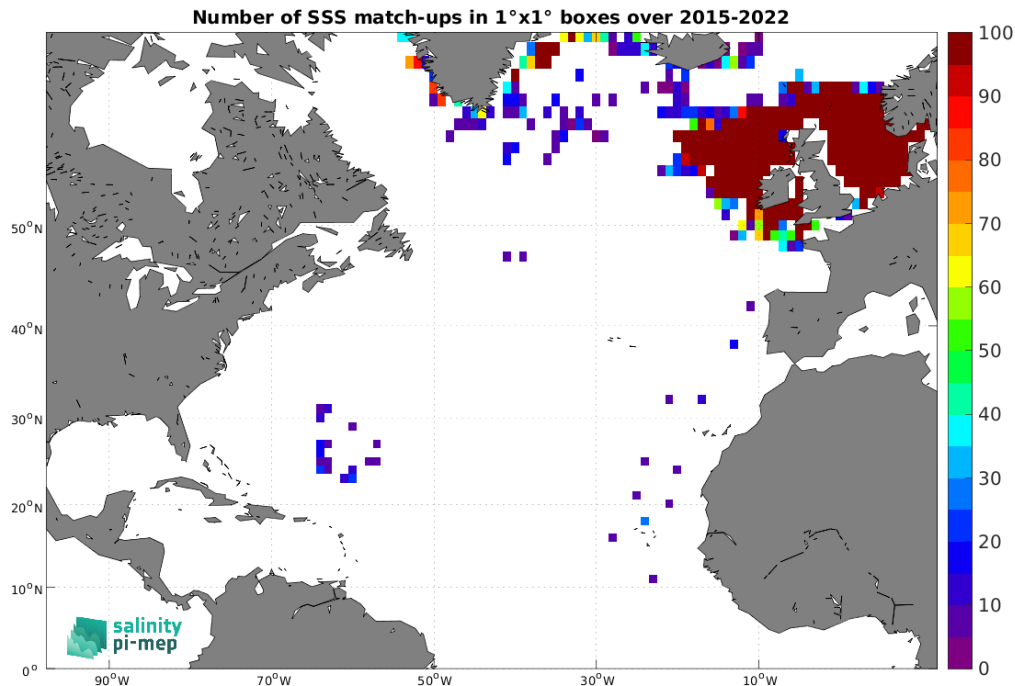
Figure 5: Number of SSS match-ups between ICES SSS and the SMAP SSS L2 v5.3 (RSS) SSS product for the North Atlantic Ocean Pi-MEP region over 1^\circ \times 1^\circ boxes and for the full satellite product period.
