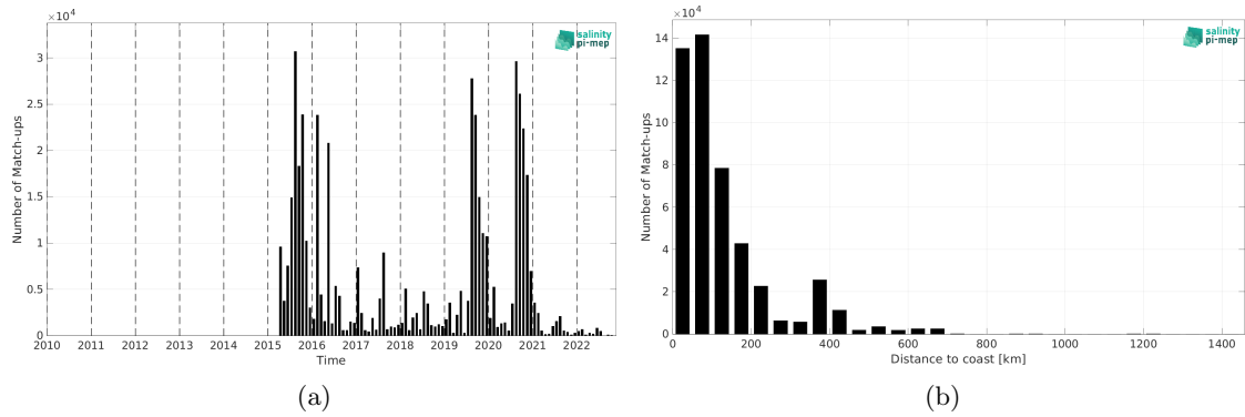
Figure 2: Number of match-ups between ICES and SMAP SSS L2 v5.3 (RSS) SSS as a function of time (a) and as function of the distance to coast (b) over the North Atlantic Ocean Pi-MEP region and for the full satellite product period.
