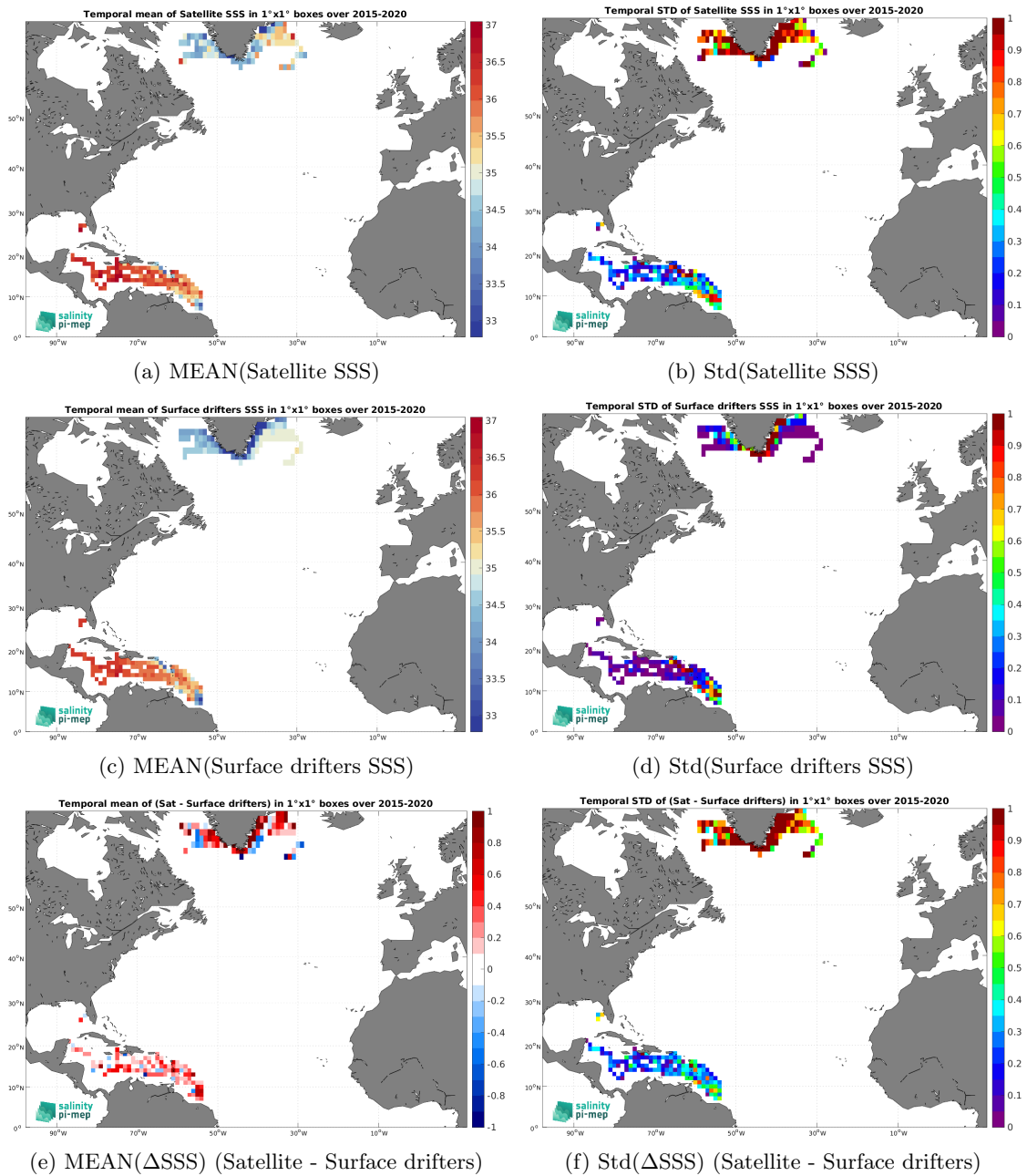
Figure 6: Temporal mean (left) and Std (right) of SSS from SMAP SSS L2 v5.3 (RSS) (top), Surface drifters (middle), and of \Delta SSS (Satellite - Surface drifters). Only match-up pairs are used to generate these maps.
