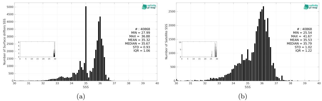
Figure 3: Histograms of SSS from Surface drifters (a) and SMAP SSS L2 v5.3 (RSS) (b) considering all match-up pairs per bins of 0.1 over the North Atlantic Ocean Pi-MEP region and for the full satellite product period.
