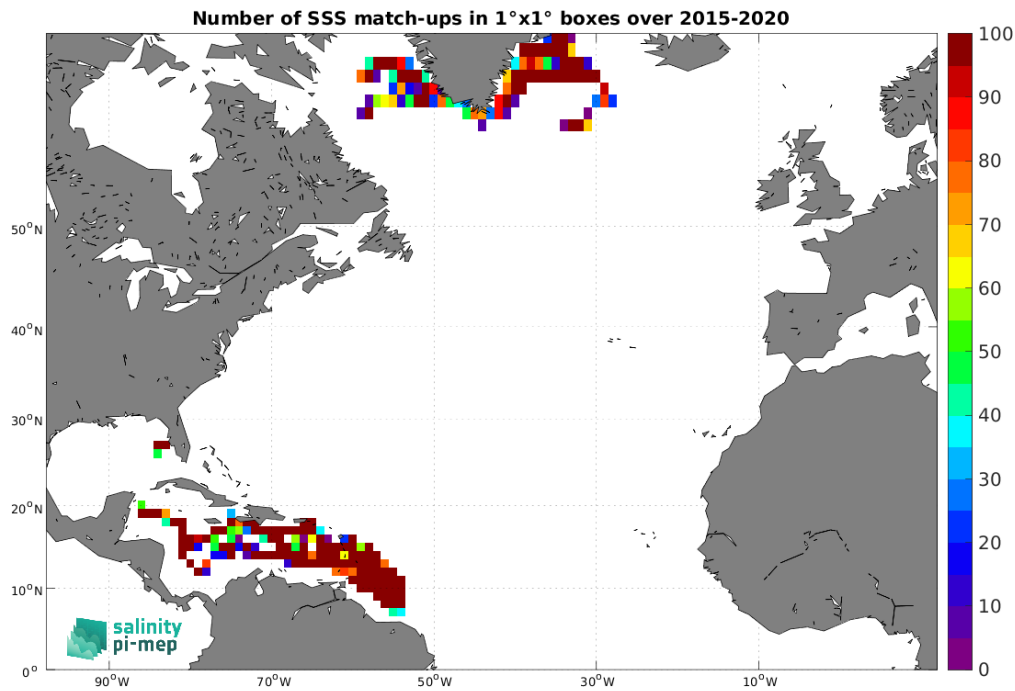
Figure 4: Number of SSS match-ups between Surface drifters SSS and the SMAP SSS L2 v5.3 (RSS) SSS product for the North Atlantic Ocean Pi-MEP region over 1^\circ \times 1^\circ boxes and for the full satellite product period.
