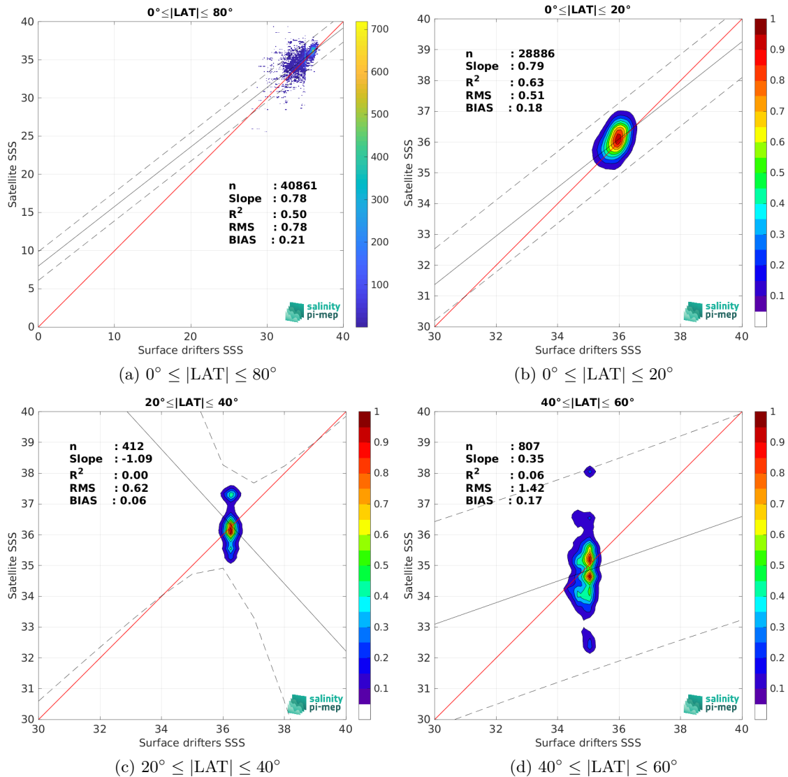
Figure 9: Contour maps of the concentration of SMAP SSS L2 v5.3 (RSS) SSS (y-axis) versus Surface drifters SSS (x-axis) at match-up pairs for different latitude bands. For each plot, the red line shows x=y . The black thin and dashed lines indicate a linear fit through the data cloud and the \pm 95\% confidence levels, respectively. The number match-up pairs n , the slope and R^2 coefficient of the linear fit, the root mean square (RMS) and the mean bias between satellite and in situ data are indicated for each latitude band in each plots.
