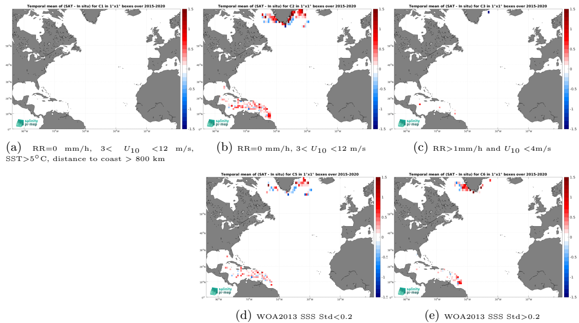
Figure 13: Temporal mean gridded over spatial boxes of size 1^\circ \times 1^\circ of \Delta SSS (SMAP SSS L2 v5.3 (RSS) - Surface drifters) for 5 different subdatasets corresponding to:RR=0 mm/h, 3 < U_{10} < 12 m/s, SST >5^\circ\text{C} , distance to coast > 800 km (a), RR=0 mm/h, 3 < U_{10} < 12 m/s (b), RR >1 mm/h and U_{10} < 4 m/s (c), WOA2013 SSS Std <0.2 (d), WOA2013 SSS Std >0.2 (e).
