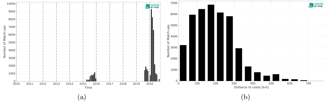
Figure 2: Number of match-ups between Surface drifters and SMAP SSS L2 v5.3 (RSS) SSS as a function of time (a) and as function of the distance to coast (b) over the North Atlantic Ocean Pi-MEP region and for the full satellite product period.
