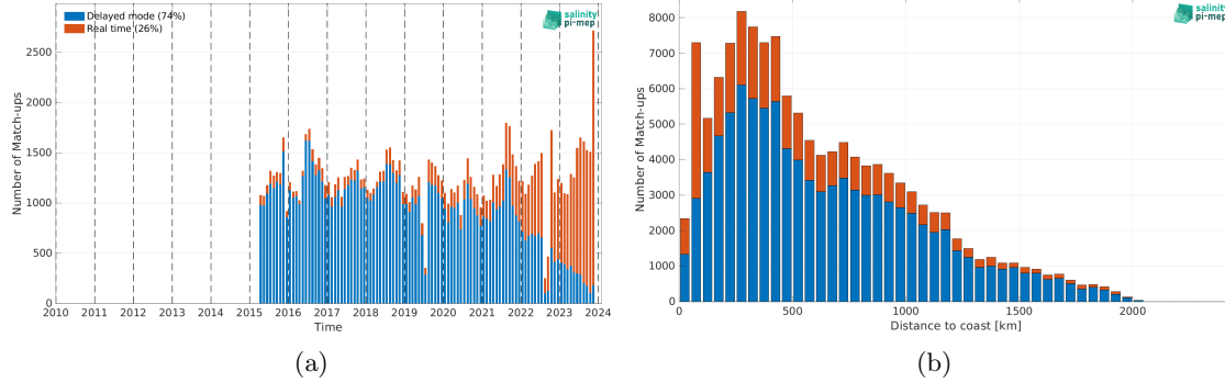
Figure 2: Number of match-ups between Argo and SMAP SSS L2 v5.3 (RSS) SSS as a function of time (a) and as function of the distance to coast (b) over the North Atlantic Ocean Pi-MEP region and for the full satellite product period.
