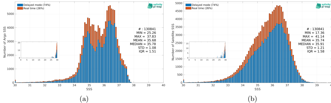
Figure 3: Histograms of SSS from Argo (a) and SMAP SSS L2 v5.3 (RSS) (b) considering all match-up pairs per bins of 0.1 over the North Atlantic Ocean Pi-MEP region and for the full satellite product period.
