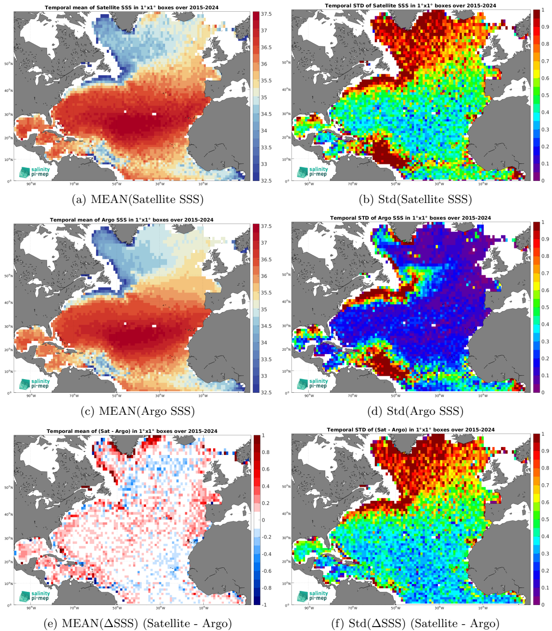
Figure 7: Temporal mean (left) and Std (right) of SSS from SMAP SSS L2 v5.3 (RSS) (top), Argo (middle), and of \Delta SSS (Satellite - Argo). Only match-up pairs are used to generate these maps.
