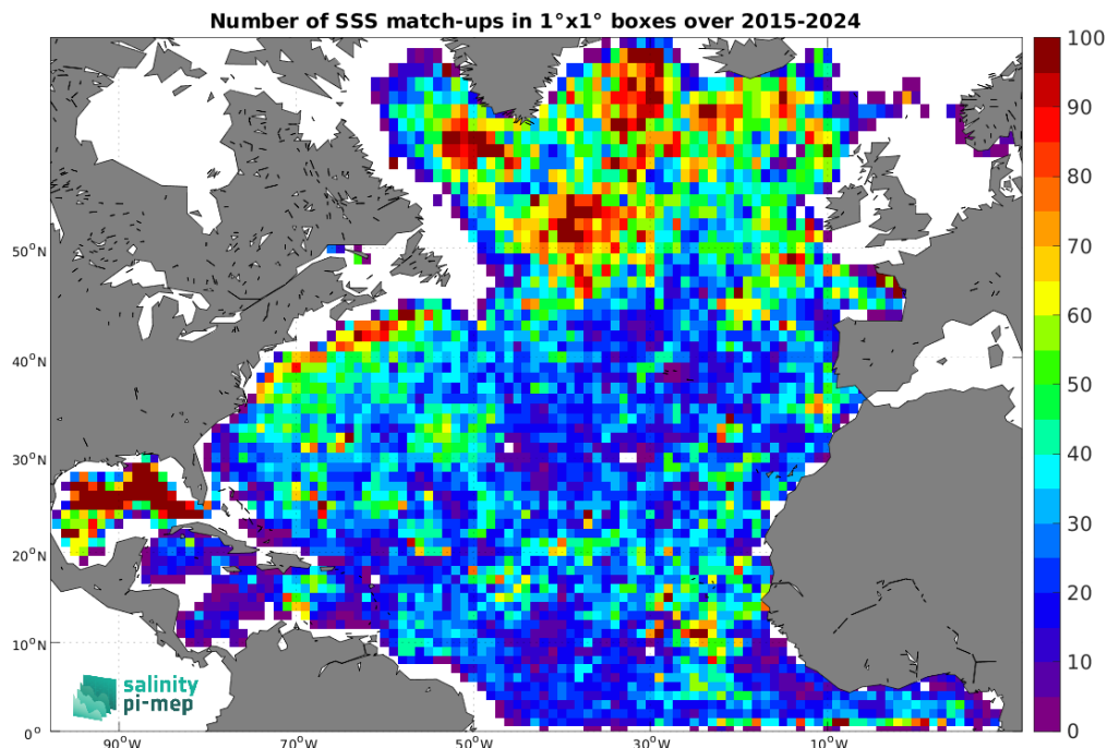
Figure 5: Number of SSS match-ups between Argo SSS and the SMAP SSS L2 v5.3 (RSS) SSS product for the North Atlantic Ocean Pi-MEP region over 1^\circ \times 1^\circ boxes and for the full satellite product period.
