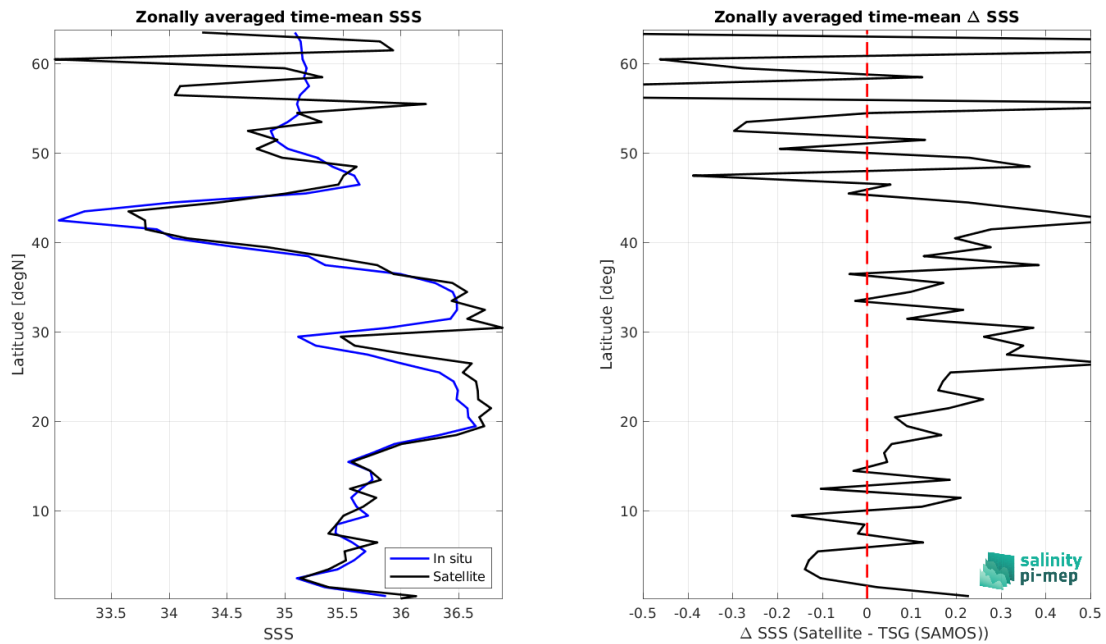
Figure 9: Left panel: Zonal mean SSS from SMAP SSS L2 v5.3 - 40 km (RSS) satellite product (black) and from TSG (SAMOS) (blue). Right panel: Zonal mean of \Delta SSS (Satellite - TSG (SAMOS)) for all the collected Pi-MEP match-up pairs estimated over the full satellite product period.
