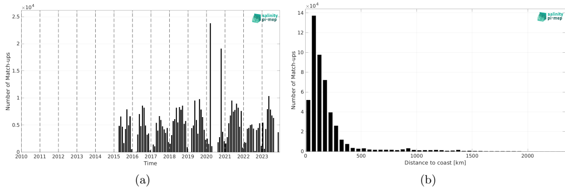
Figure 2: Number of match-ups between TSG (SAMOS) and SMAP SSS L2 v5.3 - 40 km (RSS) SSS as a function of time (a) and as function of the distance to coast (b) over the North Atlantic Ocean Pi-MEP region and for the full satellite product period.
