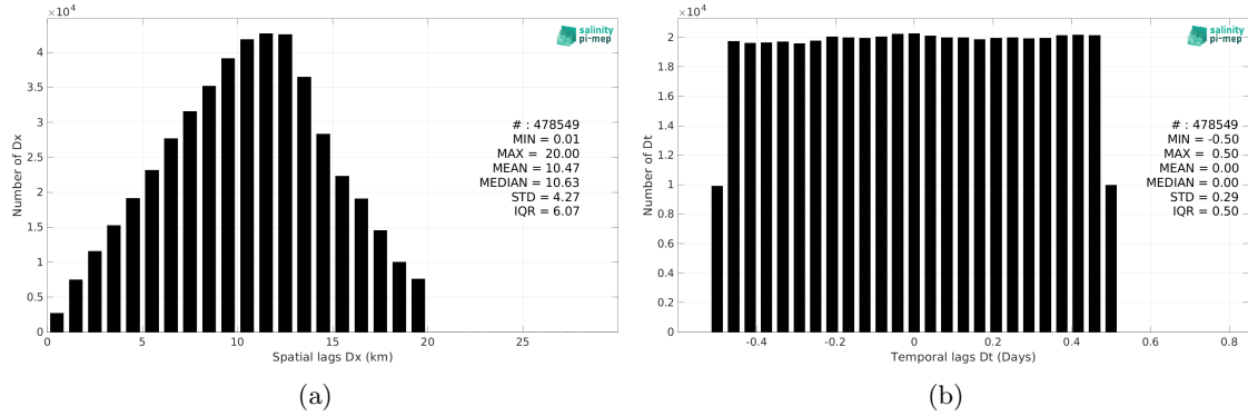
Figure 6: Histograms of the spatial (a) and temporal (b) lags between the location/time of the TSG (SAMOS) measurement and the date of the corresponding SMAP SSS L2 v5.3 - 40 km (RSS) SSS pixel.
