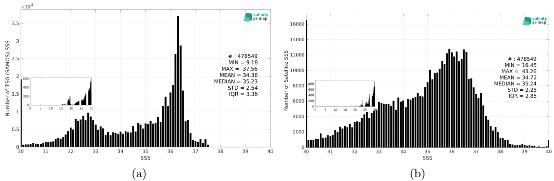
Figure 3: Histograms of SSS from TSG (SAMOS) (a) and SMAP SSS L2 v5.3 - 40 km (RSS) (b) considering all match-up pairs per bins of 0.1 over the North Atlantic Ocean Pi-MEP region and for the full satellite product period.
