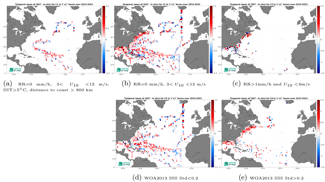
Figure 14: Temporal mean gridded over spatial boxes of size 1^\circ \times 1^\circ of \Delta\text{SSS} (SMAP SSS L2 v5.3 - 40 km (RSS) - TSG (SAMOS)) for 5 different subdatasets corresponding to:RR=0 mm/h, 3 < U_{10} < 12 m/s, SST > 5°C, distance to coast > 800 km (a), RR=0 mm/h, 3 < U_{10} < 12 m/s (b), RR > 1mm/h and U_{10} < 4 m/s (c), WOA2013 SSS Std < 0.2 (d), WOA2013 SSS Std > 0.2 (e).
