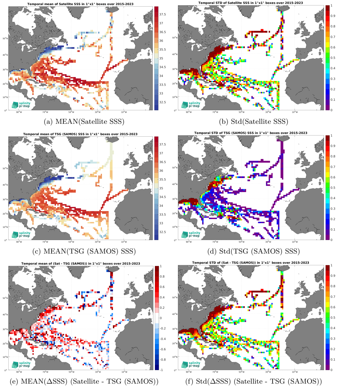
Figure 7: Temporal mean (left) and Std (right) of SSS from SMAP SSS L2 v5.3 - 40 km (RSS) (top), TSG (SAMOS) (middle), and of \Delta SSS (Satellite - TSG (SAMOS)). Only match-up pairs are used to generate these maps.
