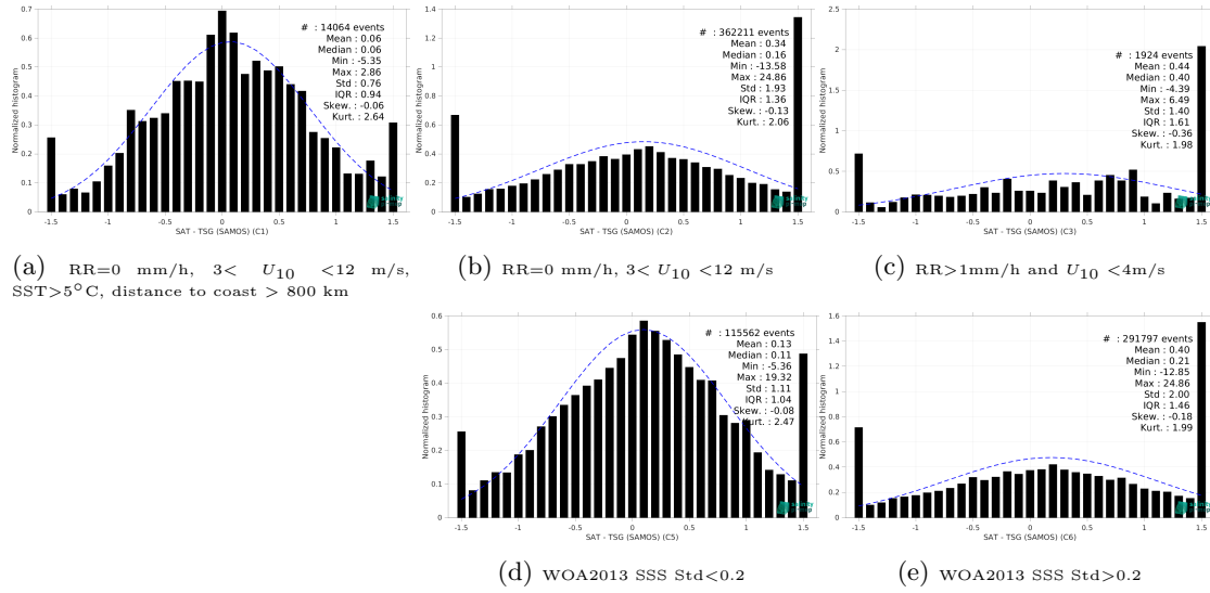
Figure 15: Normalized histogram of \Delta SSS (SMAP SSS L2 v5.3 - 40 km (RSS) - TSG (SAMOS)) for 5 different subdatasets corresponding to: RR=0 mm/h, 3 < U_{10} < 12 m/s, SST > 5°C, distance to coast > 800 km (a), RR=0 mm/h, 3 < U_{10} < 12 m/s (b), RR > 1mm/h and U_{10} < 4 m/s (c), WOA2013 SSS Std < 0.2 (d), WOA2013 SSS Std > 0.2 (e).
