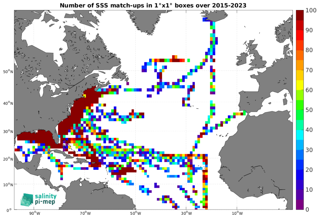
Figure 5: Number of SSS match-ups between TSG (SAMOS) SSS and the SMAP SSS L2 v5.3 - 40 km (RSS) SSS product for the North Atlantic Ocean Pi-MEP region over 1^\circ \times 1^\circ boxes and for the full satellite product period.
