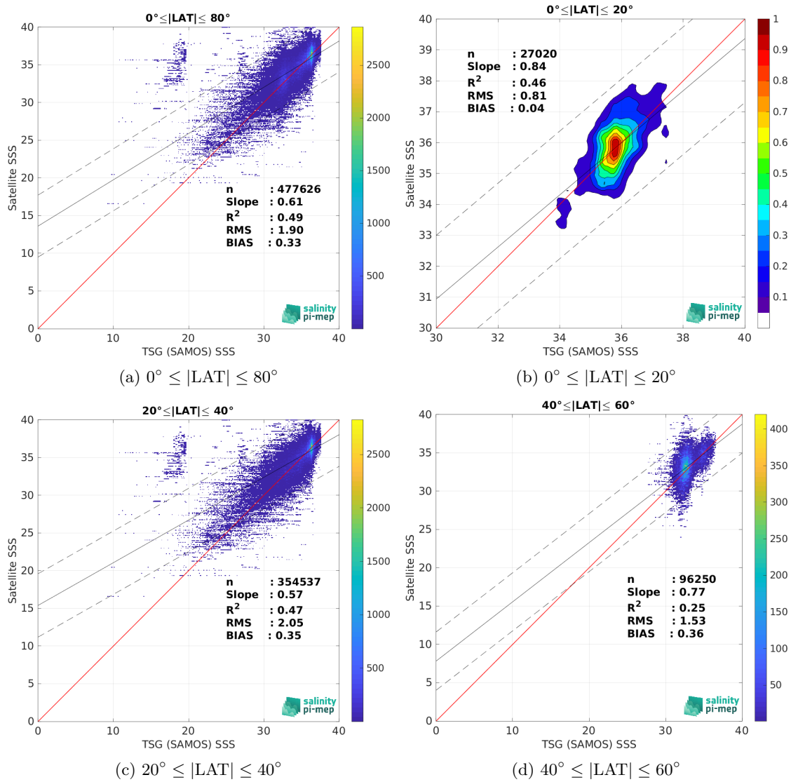
Figure 10: Contour maps of the concentration of SMAP SSS L2 v5.3 - 40 km (RSS) SSS (y-axis) versus TSG (SAMOS) SSS (x-axis) at match-up pairs for different latitude bands. For each plot, the red line shows x=y . The black thin and dashed lines indicate a linear fit through the data cloud and the \pm 95\% confidence levels, respectively. The number match-up pairs n , the slope and R^2 coefficient of the linear fit, the root mean square (RMS) and the mean bias between satellite and in situ data are indicated for each latitude band in each plots.
