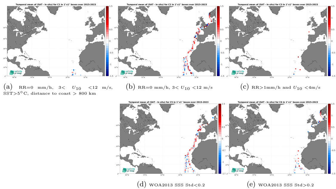
Figure 14: Temporal mean gridded over spatial boxes of size 1^\circ \times 1^\circ of \Delta\text{SSS} (SMAP SSS L2 v5.3 - 40 km (RSS) - TSG (Polarstern)) for 5 different subdatasets corresponding to:RR=0 mm/h, 3 < U_{10} < 12 m/s, SST > 5°C, distance to coast > 800 km (a), RR=0 mm/h, 3 < U_{10} < 12 m/s (b), RR > 1mm/h and U_{10} < 4 m/s (c), WOA2013 SSS Std < 0.2 (d), WOA2013 SSS Std > 0.2 (e).
