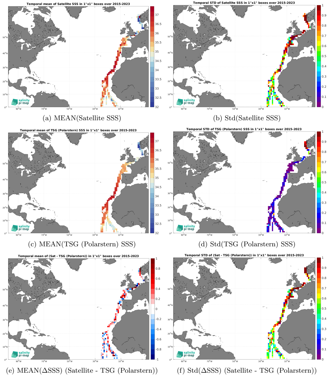
Figure 7: Temporal mean (left) and Std (right) of SSS from SMAP SSS L2 v5.3 - 40 km (RSS) (top), TSG (Polarstern) (middle), and of \Delta SSS (Satellite - TSG (Polarstern)). Only match-up pairs are used to generate these maps.
