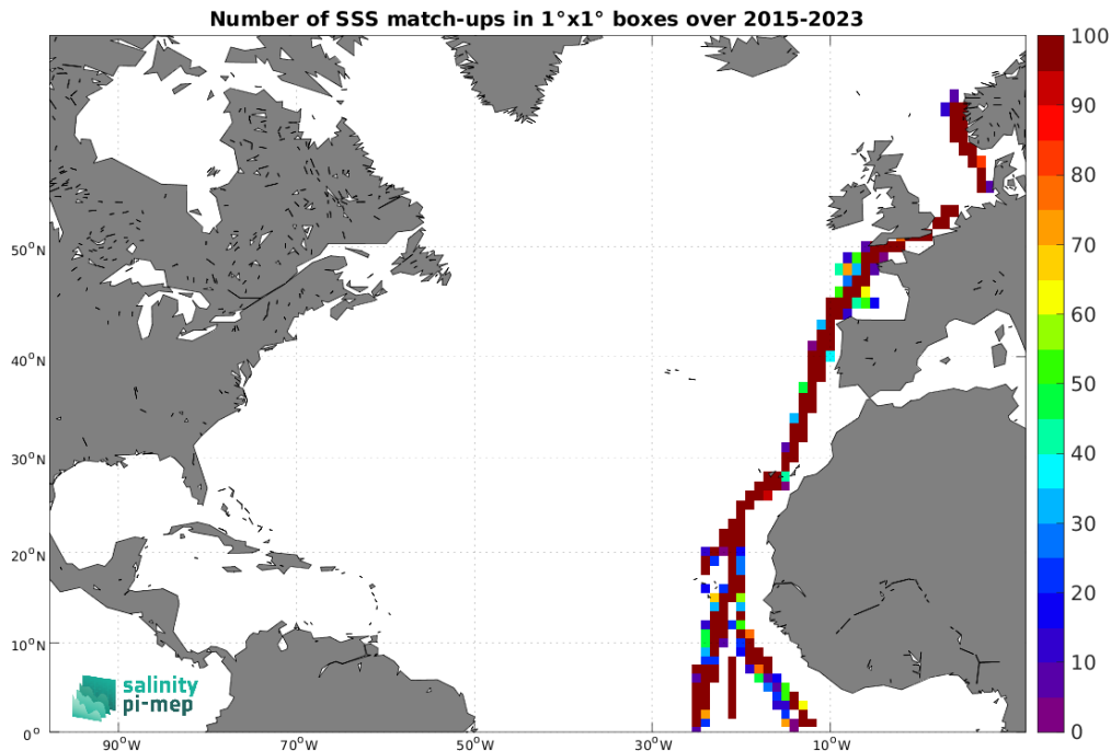
Figure 5: Number of SSS match-ups between TSG (Polarstern) SSS and the SMAP SSS L2 v5.3 - 40 km (RSS) SSS product for the North Atlantic Ocean Pi-MEP region over 1^\circ \times 1^\circ boxes and for the full satellite product period.
