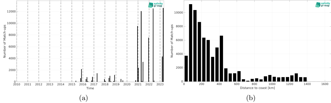
Figure 2: Number of match-ups between TSG (Polarstern) and SMAP SSS L2 v5.3 - 40 km (RSS) SSS as a function of time (a) and as function of the distance to coast (b) over the North Atlantic Ocean Pi-MEP region and for the full satellite product period.
