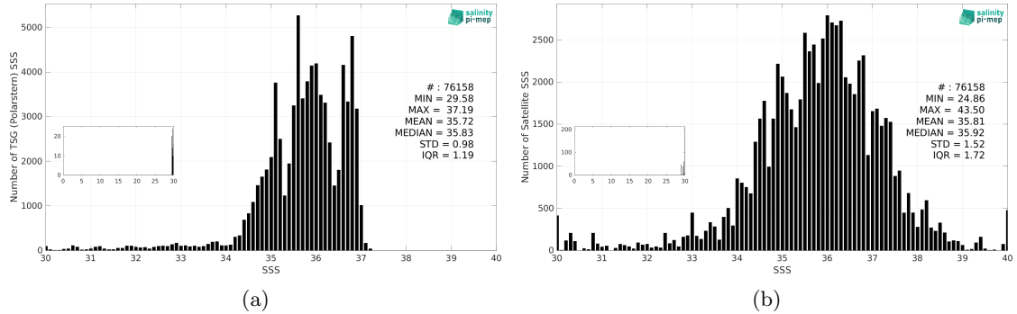
Figure 3: Histograms of SSS from TSG (Polarstern) (a) and SMAP SSS L2 v5.3 - 40 km (RSS) (b) considering all match-up pairs per bins of 0.1 over the North Atlantic Ocean Pi-MEP region and for the full satellite product period.
