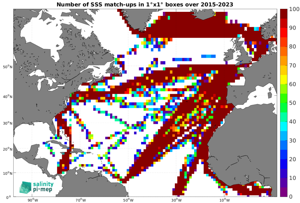
Figure 5: Number of SSS match-ups between TSG (LEGOS-DM) SSS and the SMAP SSS L2 v5.3 - 40 km (RSS) SSS product for the North Atlantic Ocean Pi-MEP region over 1^\circ \times 1^\circ boxes and for the full satellite product period.
