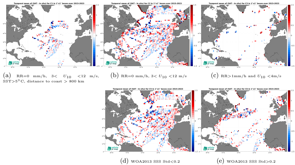
Figure 14: Temporal mean gridded over spatial boxes of size 1^\circ \times 1^\circ of \Delta\text{SSS} (SMAP SSS L2 v5.3 - 40 km (RSS) - TSG (LEGOS-DM)) for 5 different subdatasets corresponding to:RR=0 mm/h, 3 < U_{10} < 12 m/s, SST > 5°C, distance to coast > 800 km (a), RR=0 mm/h, 3 < U_{10} < 12 m/s (b), RR > 1mm/h and U_{10} < 4 m/s (c), WOA2013 SSS Std < 0.2 (d), WOA2013 SSS Std > 0.2 (e).
