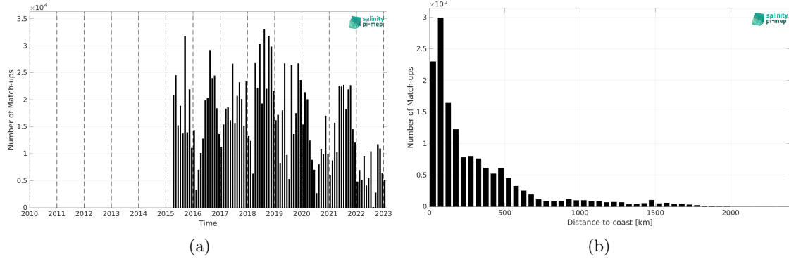
Figure 2: Number of match-ups between TSG (LEGOS-DM) and SMAP SSS L2 v5.3 - 40 km (RSS) SSS as a function of time (a) and as function of the distance to coast (b) over the North Atlantic Ocean Pi-MEP region and for the full satellite product period.
