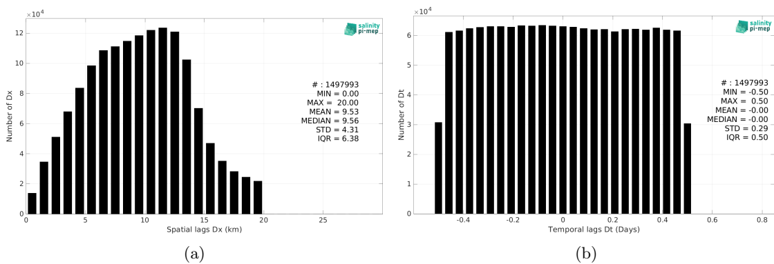
Figure 6: Histograms of the spatial (a) and temporal (b) lags between the location/time of the TSG (LEGOS-DM) measurement and the date of the corresponding SMAP SSS L2 v5.3 - 40 km (RSS) SSS pixel.
