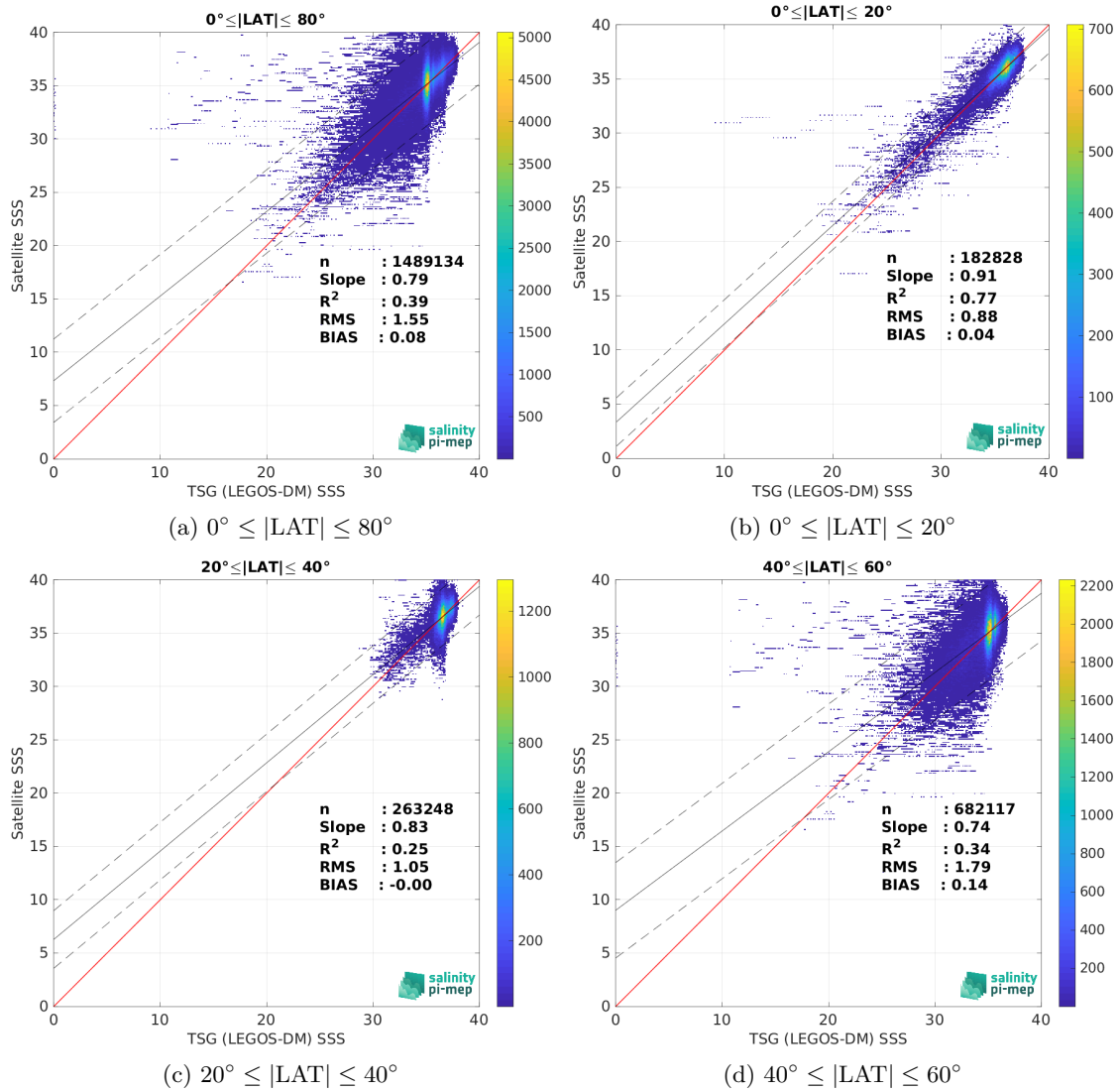
Figure 10: Contour maps of the concentration of SMAP SSS L2 v5.3 - 40 km (RSS) SSS (y-axis) versus TSG (LEGOS-DM) SSS (x-axis) at match-up pairs for different latitude bands. For each plot, the red line shows x=y . The black thin and dashed lines indicate a linear fit through the data cloud and the \pm 95\% confidence levels, respectively. The number match-up pairs n , the slope and R^2 coefficient of the linear fit, the root mean square (RMS) and the mean bias between satellite and in situ data are indicated for each latitude band in each plots.
