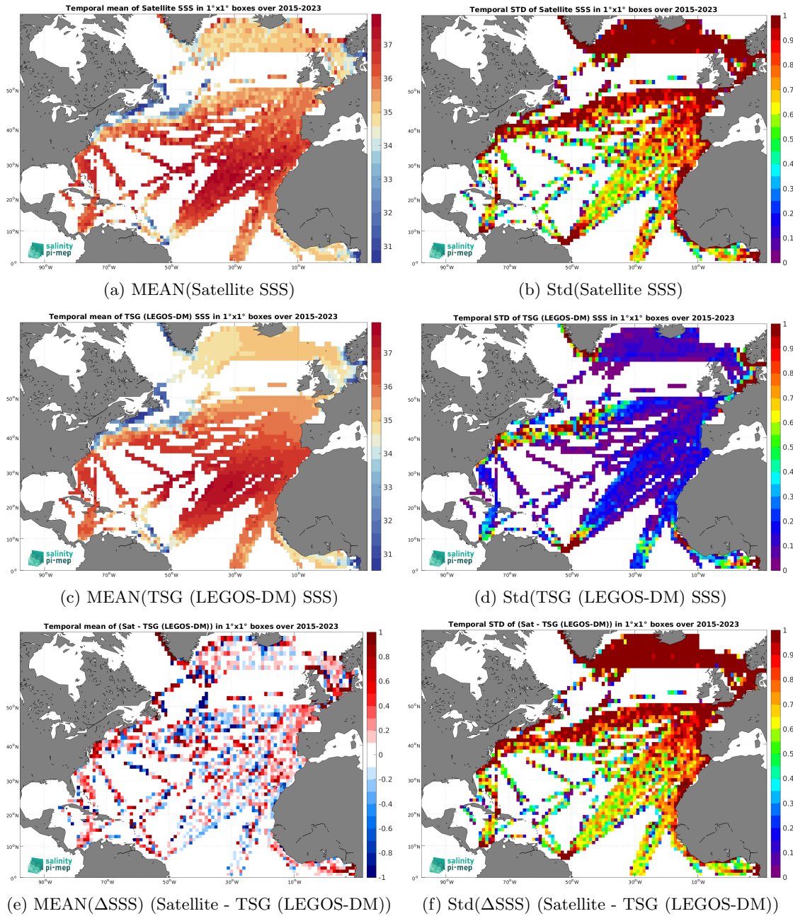
Figure 7: Temporal mean (left) and Std (right) of SSS from SMAP SSS L2 v5.3 - 40 km (RSS) (top), TSG (LEGOS-DM) (middle), and of \Delta SSS (Satellite - TSG (LEGOS-DM)). Only match-up pairs are used to generate these maps.
