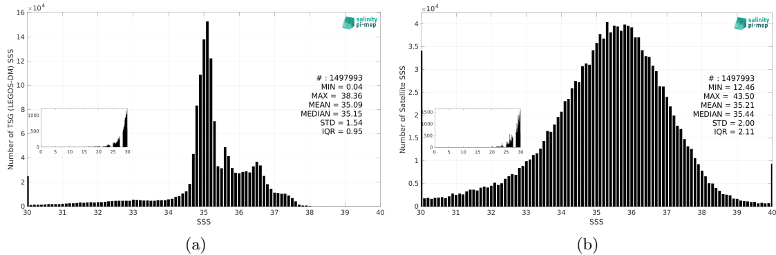
Figure 3: Histograms of SSS from TSG (LEGOS-DM) (a) and SMAP SSS L2 v5.3 - 40 km (RSS) (b) considering all match-up pairs per bins of 0.1 over the North Atlantic Ocean Pi-MEP region and for the full satellite product period.
