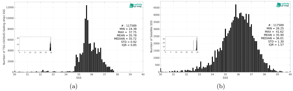
Figure 3: Histograms of SSS from TSG (GOSUD-Sailing-ship) (a) and SMAP SSS L2 v5.3 - 40 km (RSS) (b) considering all match-up pairs per bins of 0.1 over the North Atlantic Ocean Pi-MEP region and for the full satellite product period.
