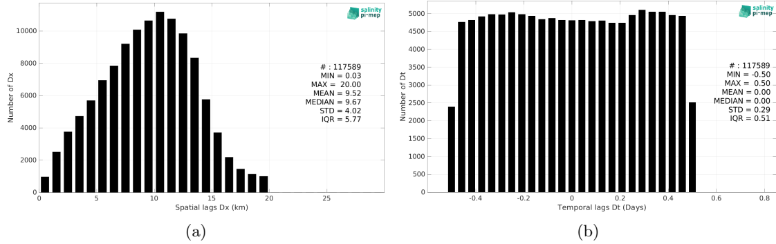
Figure 6: Histograms of the spatial (a) and temporal (b) lags between the location/time of the TSG (GOSUD-Sailing-ship) measurement and the date of the corresponding SMAP SSS L2 v5.3 - 40 km (RSS) SSS pixel.
