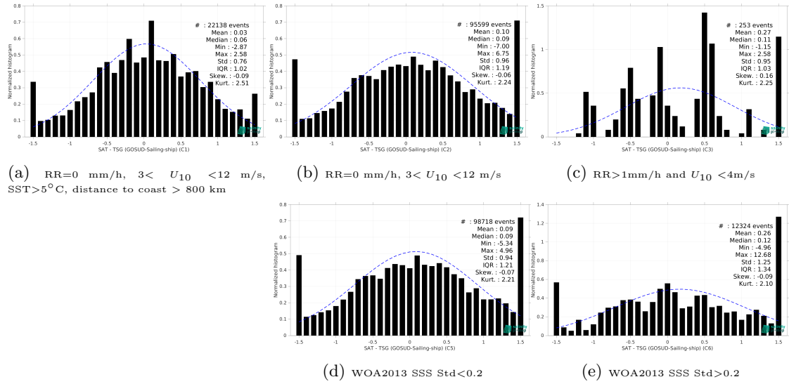
Figure 15: Normalized histogram of \Delta SSS (SMAP SSS L2 v5.3 - 40 km (RSS) - TSG (GOSUD-Sailing-ship)) for 5 different subdatasets corresponding to: RR=0 mm/h, 3 < U_{10} < 12 m/s, SST>5°C, distance to coast > 800 km (a), RR=0 mm/h, 3 < U_{10} < 12 m/s (b), RR>1mm/h and U_{10} < 4 m/s (c), WOA2013 SSS Std<0.2 (d), WOA2013 SSS Std>0.2 (e).
