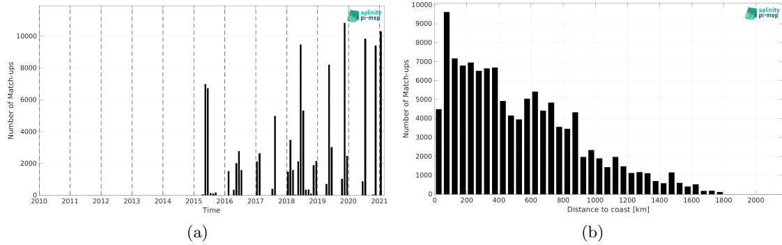
Figure 2: Number of match-ups between TSG (GOSUD-Sailing-ship) and SMAP SSS L2 v5.3 - 40 km (RSS) SSS as a function of time (a) and as function of the distance to coast (b) over the North Atlantic Ocean Pi-MEP region and for the full satellite product period.
