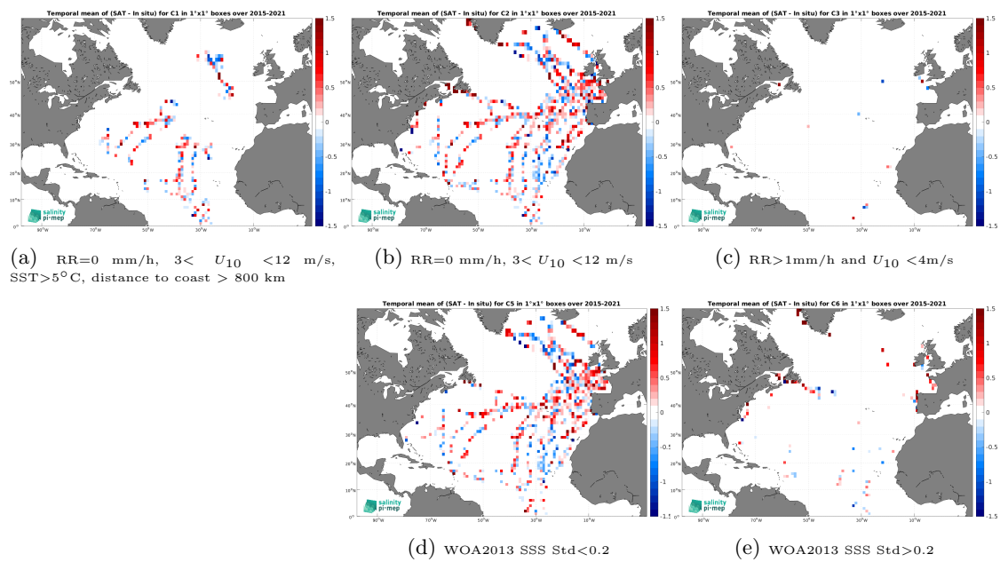
Figure 14: Temporal mean gridded over spatial boxes of size 1^\circ \times 1^\circ of \Delta\text{SSS} (SMAP SSS L2 v5.3 - 40 km (RSS) - TSG (GOSUD-Sailing-ship)) for 5 different subdatasets corresponding to:RR=0 mm/h, 3 < U_{10} < 12 m/s, SST >5^\circ\text{C} , distance to coast > 800 km (a), RR=0 mm/h, 3 < U_{10} < 12 m/s (b), RR >1 mm/h and U_{10} < 4 m/s (c), WOA2013 SSS Std <0.2 (d), WOA2013 SSS Std >0.2 (e).
