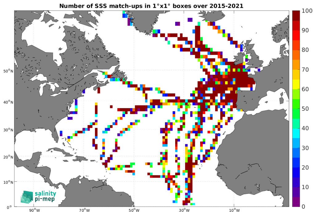
Figure 5: Number of SSS match-ups between TSG (GOSUD-Sailing-ship) SSS and the SMAP SSS L2 v5.3 - 40 km (RSS) SSS product for the North Atlantic Ocean Pi-MEP region over 1^\circ \times 1^\circ boxes and for the full satellite product period.
