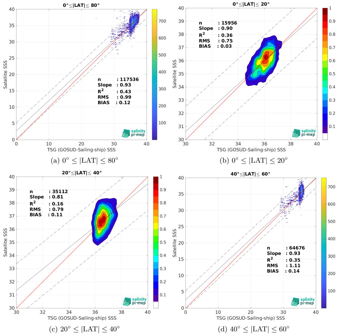
Figure 10: Contour maps of the concentration of SMAP SSS L2 v5.3 - 40 km (RSS) SSS (y-axis) versus TSG (GOSUD-Sailing-ship) SSS (x-axis) at match-up pairs for different latitude bands. For each plot, the red line shows x=y . The black thin and dashed lines indicate a linear fit through the data cloud and the \pm 95\% confidence levels, respectively. The number match-up pairs n , the slope and R^2 coefficient of the linear fit, the root mean square (RMS) and the mean bias between satellite and in situ data are indicated for each latitude band in each plots.
