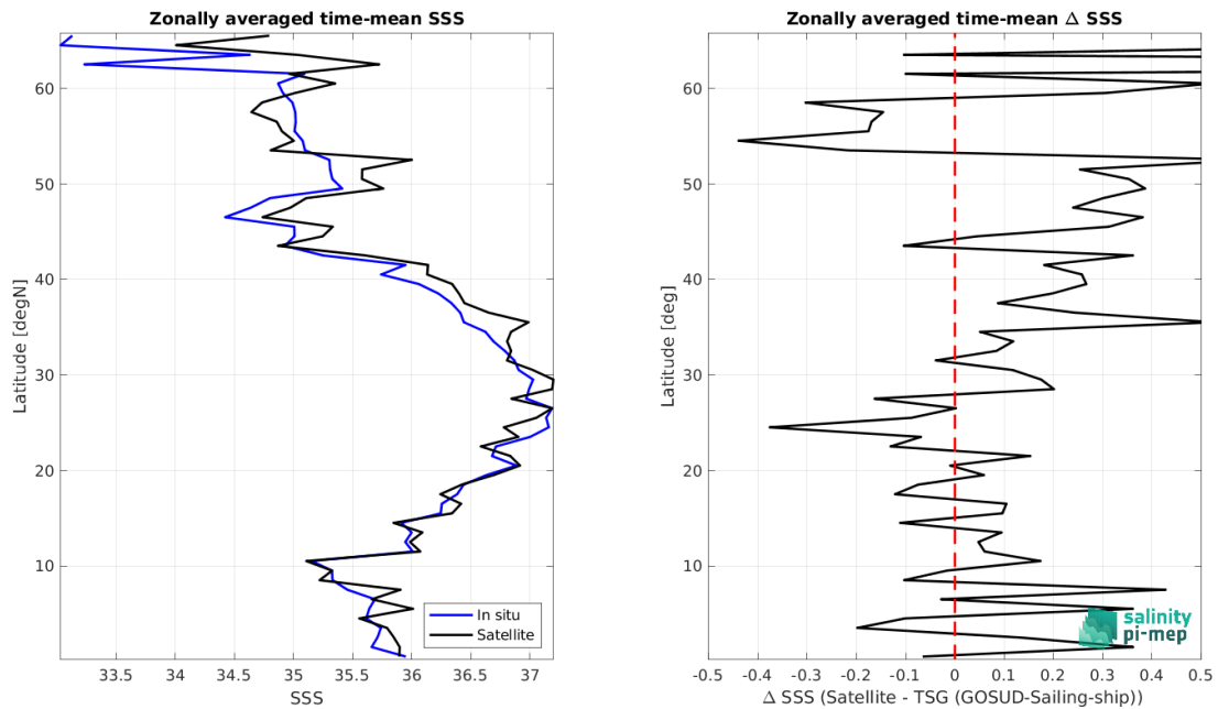
Figure 9: Left panel: Zonal mean SSS from SMAP SSS L2 v5.3 - 40 km (RSS) satellite product (black) and from TSG (GOSUD-Sailing-ship) (blue). Right panel: Zonal mean of \Delta SSS (Satellite - TSG (GOSUD-Sailing-ship)) for all the collected Pi-MEP match-up pairs estimated over the full satellite product period.
