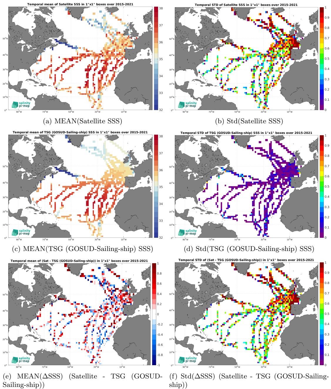
Figure 7: Temporal mean (left) and Std (right) of SSS from SMAP SSS L2 v5.3 - 40 km (RSS) (top), TSG (GOSUD-Sailing-ship) (middle), and of \Delta SSS (Satellite - TSG (GOSUD-Sailing-ship)). Only match-up pairs are used to generate these maps.
