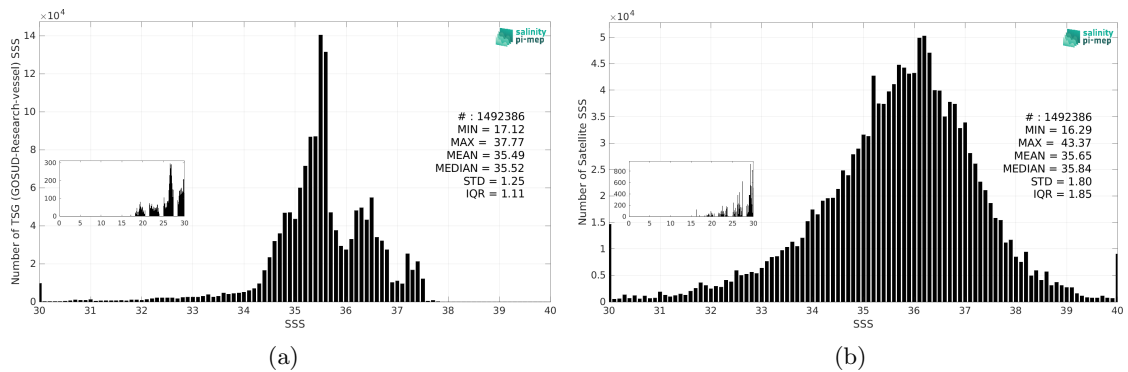
Figure 3: Histograms of SSS from TSG (GOSUD-Research-vessel) (a) and SMAP SSS L2 v5.3 - 40 km (RSS) (b) considering all match-up pairs per bins of 0.1 over the North Atlantic Ocean Pi-MEP region and for the full satellite product period.
