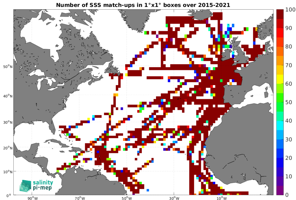
Figure 5: Number of SSS match-ups between TSG (GOSUD-Research-vessel) SSS and the SMAP SSS L2 v5.3 - 40 km (RSS) SSS product for the North Atlantic Ocean Pi-MEP region over 1^\circ \times 1^\circ boxes and for the full satellite product period.
