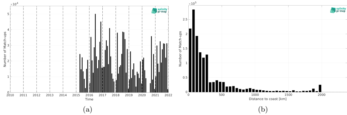
Figure 2: Number of match-ups between TSG (GOSUD-Research-vessel) and SMAP SSS L2 v5.3 - 40 km (RSS) SSS as a function of time (a) and as function of the distance to coast (b) over the North Atlantic Ocean Pi-MEP region and for the full satellite product period.
