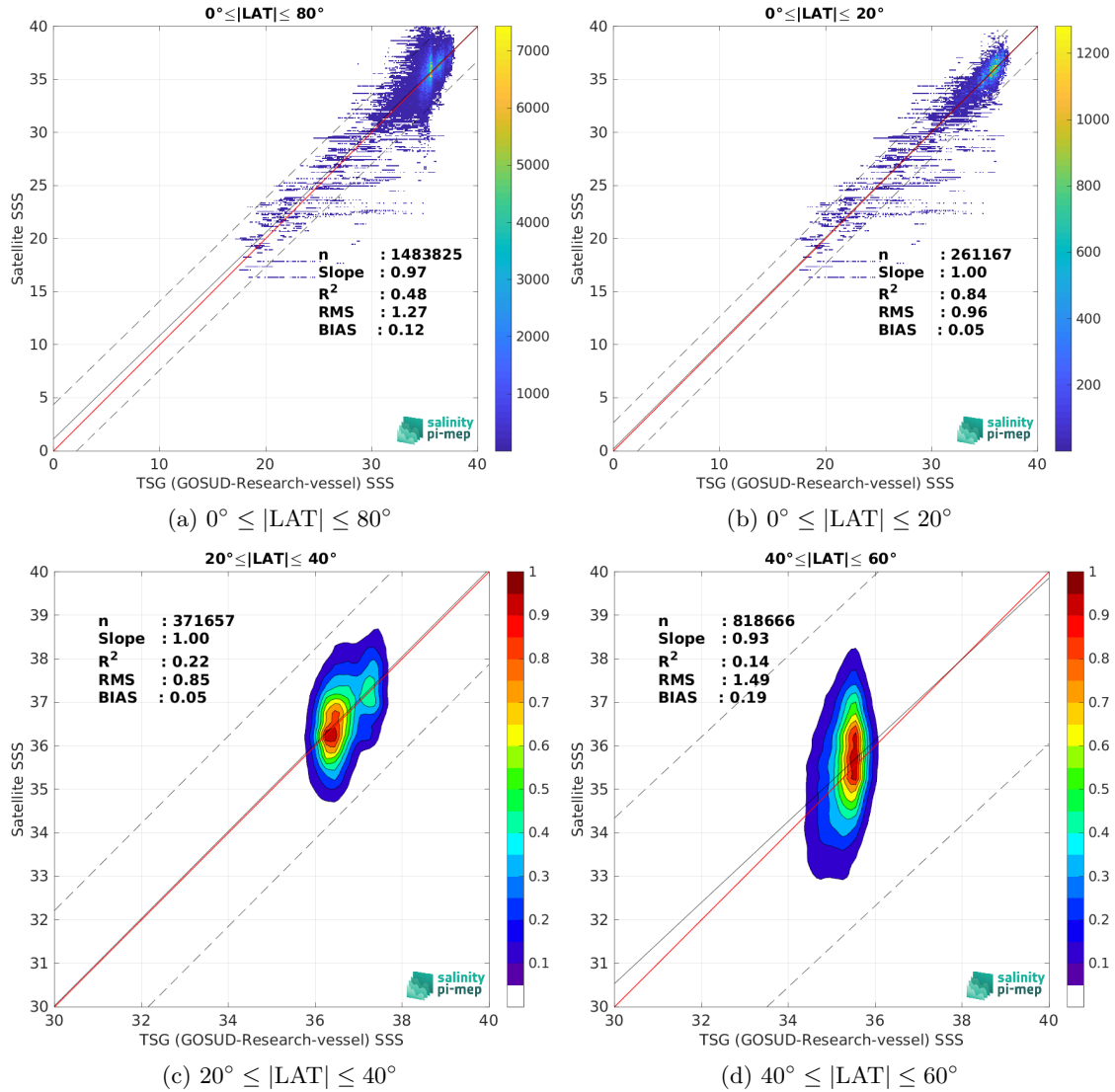
Figure 10: Contour maps of the concentration of SMAP SSS L2 v5.3 - 40 km (RSS) SSS (y-axis) versus TSG (GOSUD-Research-vessel) SSS (x-axis) at match-up pairs for different latitude bands. For each plot, the red line shows x=y . The black thin and dashed lines indicate a linear fit through the data cloud and the \pm 95\% confidence levels, respectively. The number match-up pairs n , the slope and R^2 coefficient of the linear fit, the root mean square (RMS) and the mean bias between satellite and in situ data are indicated for each latitude band in each plots.
