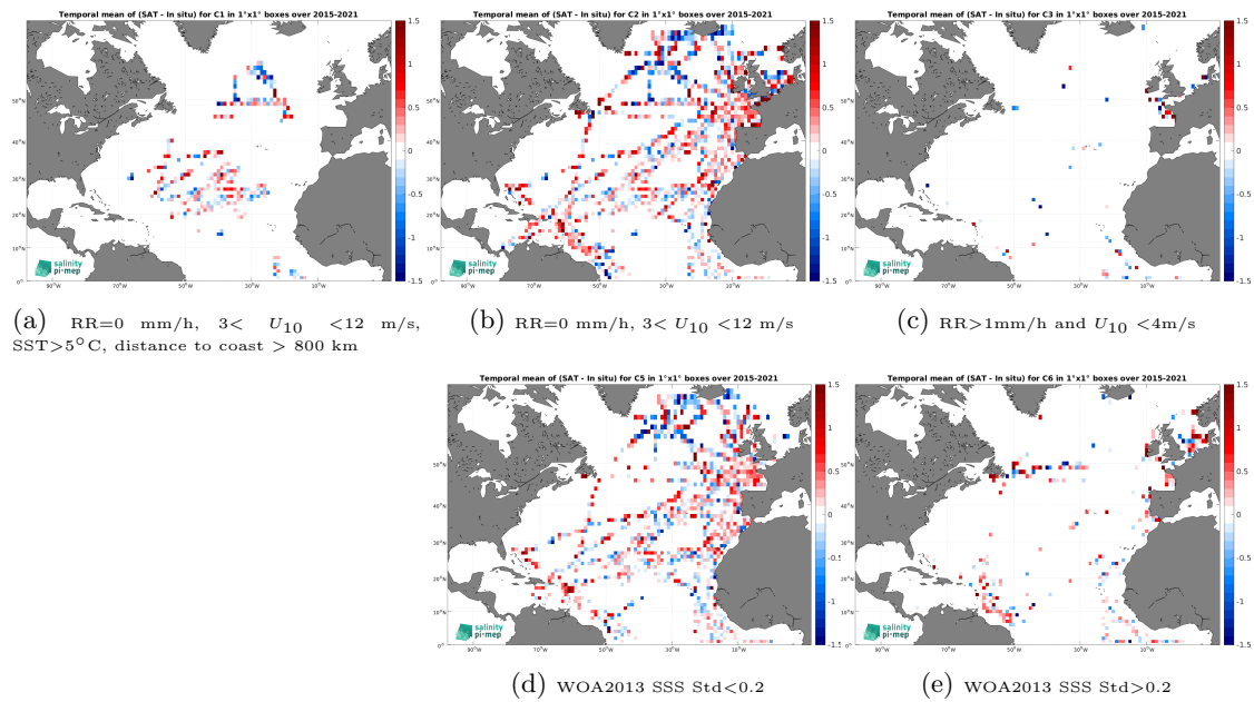
Figure 14: Temporal mean gridded over spatial boxes of size 1^\circ \times 1^\circ of \Delta\text{SSS} (SMAP SSS L2 v5.3 - 40 km (RSS) - TSG (GOSUD-Research-vessel)) for 5 different subdatasets corresponding to:RR=0 mm/h, 3 < U_{10} < 12 m/s, SST > 5°C, distance to coast > 800 km (a), RR=0 mm/h, 3 < U_{10} < 12 m/s (b), RR > 1mm/h and U_{10} < 4 m/s (c), WOA2013 SSS Std < 0.2 (d), WOA2013 SSS Std > 0.2 (e).
