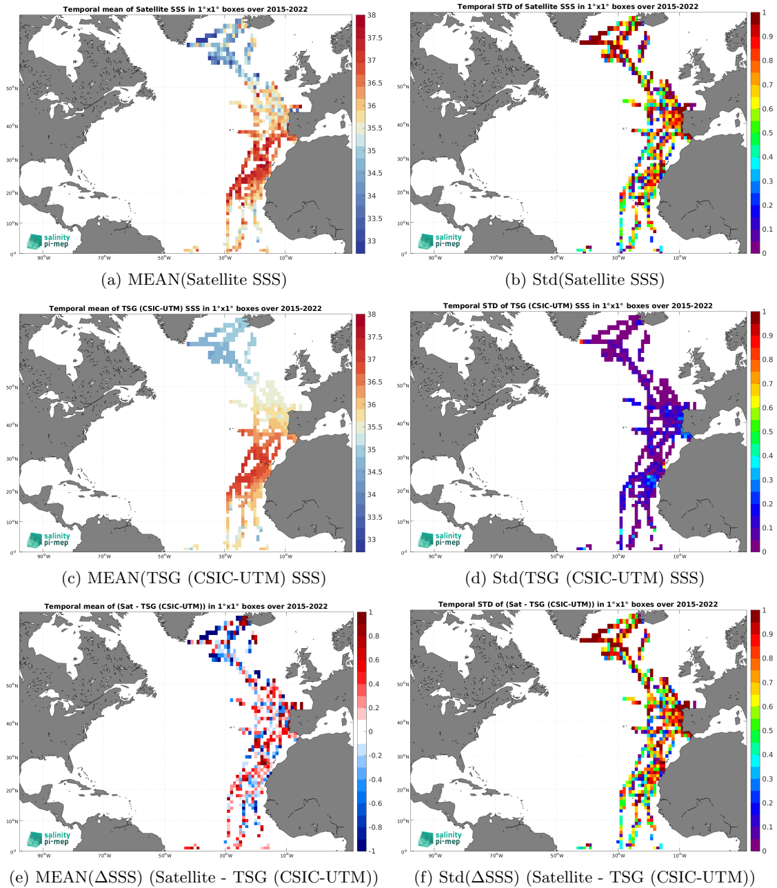
Figure 7: Temporal mean (left) and Std (right) of SSS from SMAP SSS L2 v5.3 - 40 km (RSS) (top), TSG (CSIC-UTM) (middle), and of \Delta SSS (Satellite - TSG (CSIC-UTM)). Only match-up pairs are used to generate these maps.
