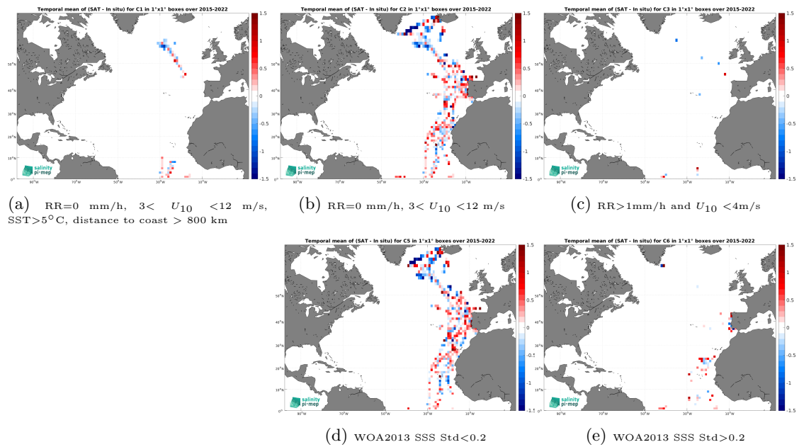
Figure 14: Temporal mean gridded over spatial boxes of size 1^\circ \times 1^\circ of \Delta\text{SSS} (SMAP SSS L2 v5.3 - 40 km (RSS) - TSG (CSIC-UTM)) for 5 different subdatasets corresponding to:RR=0 mm/h, 3 < U_{10} < 12 m/s, SST > 5°C, distance to coast > 800 km (a), RR=0 mm/h, 3 < U_{10} < 12 m/s (b), RR > 1mm/h and U_{10} < 4 m/s (c), WOA2013 SSS Std < 0.2 (d), WOA2013 SSS Std > 0.2 (e).
