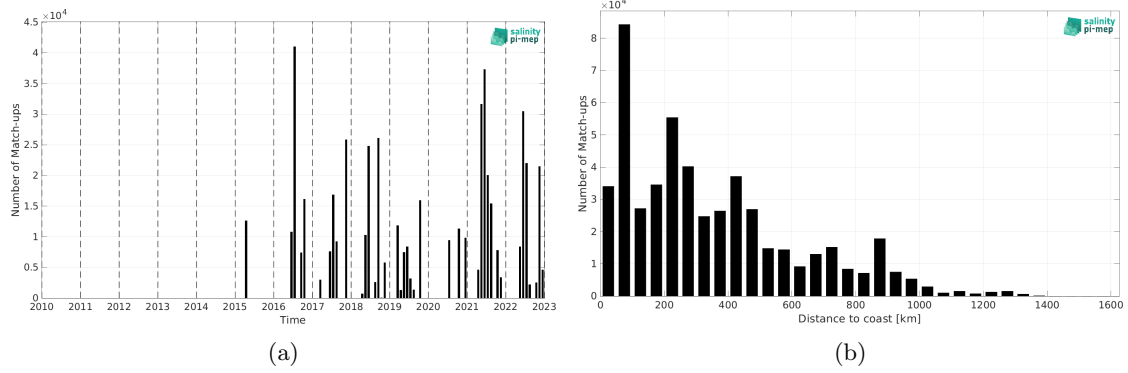
Figure 2: Number of match-ups between TSG (CSIC-UTM) and SMAP SSS L2 v5.3 - 40 km (RSS) SSS as a function of time (a) and as function of the distance to coast (b) over the North Atlantic Ocean Pi-MEP region and for the full satellite product period.
