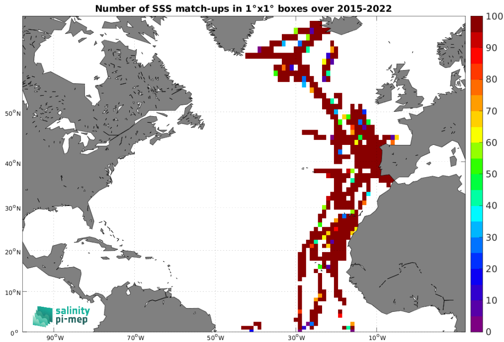
Figure 5: Number of SSS match-ups between TSG (CSIC-UTM) SSS and the SMAP SSS L2 v5.3 - 40 km (RSS) SSS product for the North Atlantic Ocean Pi-MEP region over 1^\circ \times 1^\circ boxes and for the full satellite product period.
