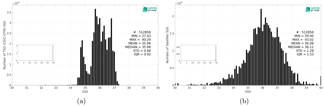
Figure 3: Histograms of SSS from TSG (CSIC-UTM) (a) and SMAP SSS L2 v5.3 - 40 km (RSS) (b) considering all match-up pairs per bins of 0.1 over the North Atlantic Ocean Pi-MEP region and for the full satellite product period.
