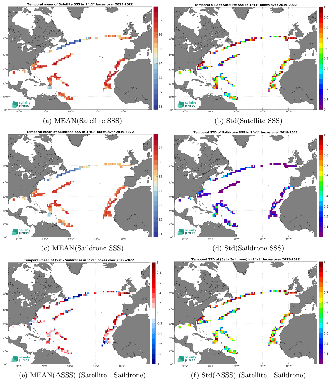
Figure 7: Temporal mean (left) and Std (right) of SSS from SMAP SSS L2 v5.3 - 40 km (RSS) (top), Saildrone (middle), and of \Delta SSS (Satellite - Saildrone). Only match-up pairs are used to generate these maps.
