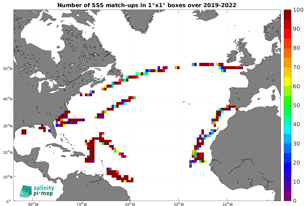
Figure 5: Number of SSS match-ups between Saildrone SSS and the SMAP SSS L2 v5.3 - 40 km (RSS) SSS product for the North Atlantic Ocean Pi-MEP region over 1^\circ \times 1^\circ boxes and for the full satellite product period.
