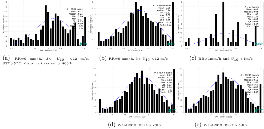
Figure 15: Normalized histogram of \Delta SSS (SMAP SSS L2 v5.3 - 40 km (RSS) - Saildrone) for 5 different subdatasets corresponding to: RR=0 mm/h, 3 < U_{10} < 12 m/s, SST > 5°C, distance to coast > 800 km (a), RR=0 mm/h, 3 < U_{10} < 12 m/s (b), RR > 1mm/h and U_{10} < 4 m/s (c), WOA2013 SSS Std < 0.2 (d), WOA2013 SSS Std > 0.2 (e).
