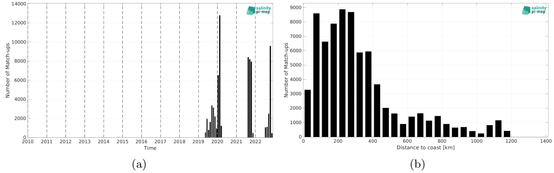
Figure 2: Number of match-ups between Saildrone and SMAP SSS L2 v5.3 - 40 km (RSS) SSS as a function of time (a) and as function of the distance to coast (b) over the North Atlantic Ocean Pi-MEP region and for the full satellite product period.
