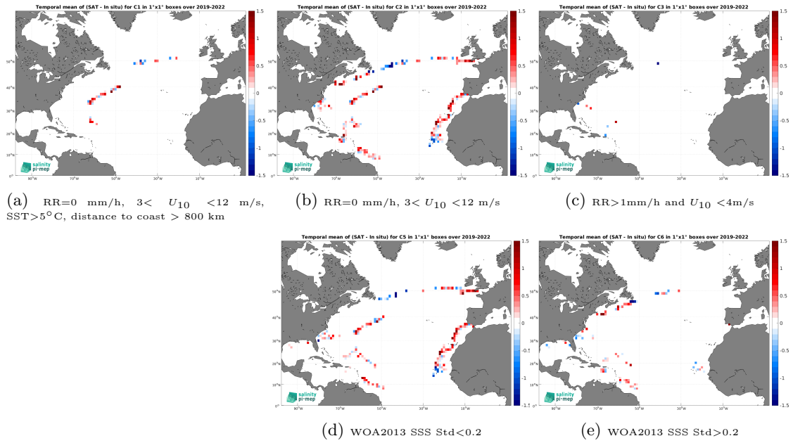
Figure 14: Temporal mean gridded over spatial boxes of size 1^\circ \times 1^\circ of \Delta SSS (SMAP SSS L2 v5.3 - 40 km (RSS) - Sailability) for 5 different subdatasets corresponding to:RR=0 mm/h, 3 < U_{10} < 12 m/s, SST>5°C, distance to coast > 800 km (a), RR=0 mm/h, 3 < U_{10} < 12 m/s (b), RR>1mm/h and U_{10} < 4 m/s (c), WOA2013 SSS Std<0.2 (d), WOA2013 SSS Std>0.2 (e).
