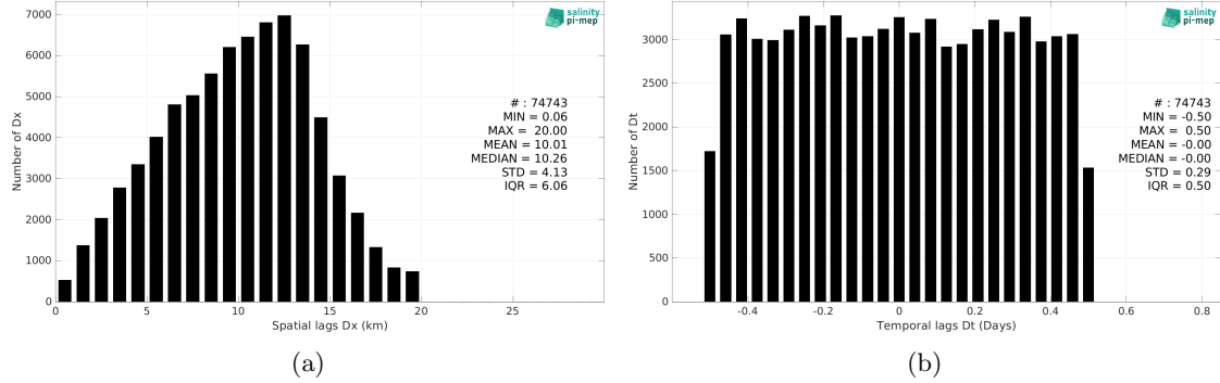
Figure 6: Histograms of the spatial (a) and temporal (b) lags between the location/time of the Saildrone measurement and the date of the corresponding SMAP SSS L2 v5.3 - 40 km (RSS) SSS pixel.
