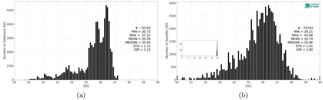
Figure 3: Histograms of SSS from Saildrone (a) and SMAP SSS L2 v5.3 - 40 km (RSS) (b) considering all match-up pairs per bins of 0.1 over the North Atlantic Ocean Pi-MEP region and for the full satellite product period.
