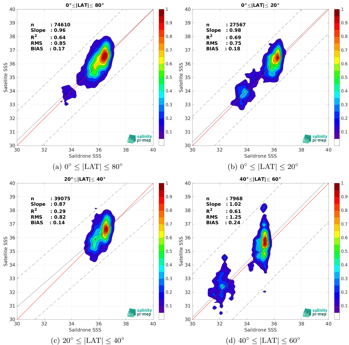
Figure 10: Contour maps of the concentration of SMAP SSS L2 v5.3 - 40 km (RSS) SSS (y-axis) versus Saildrone SSS (x-axis) at match-up pairs for different latitude bands. For each plot, the red line shows x=y . The black thin and dashed lines indicate a linear fit through the data cloud and the \pm 95\% confidence levels, respectively. The number match-up pairs n , the slope and R^2 coefficient of the linear fit, the root mean square (RMS) and the mean bias between satellite and in situ data are indicated for each latitude band in each plots.
