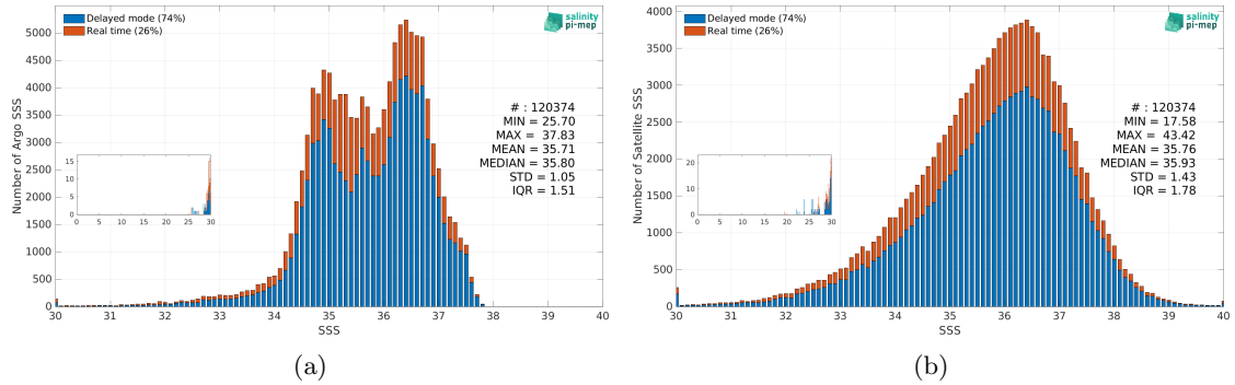
Figure 3: Histograms of SSS from Argo (a) and SMAP SSS L2 v5.3 - 40 km (RSS) (b) considering all match-up pairs per bins of 0.1 over the North Atlantic Ocean Pi-MEP region and for the full satellite product period.
