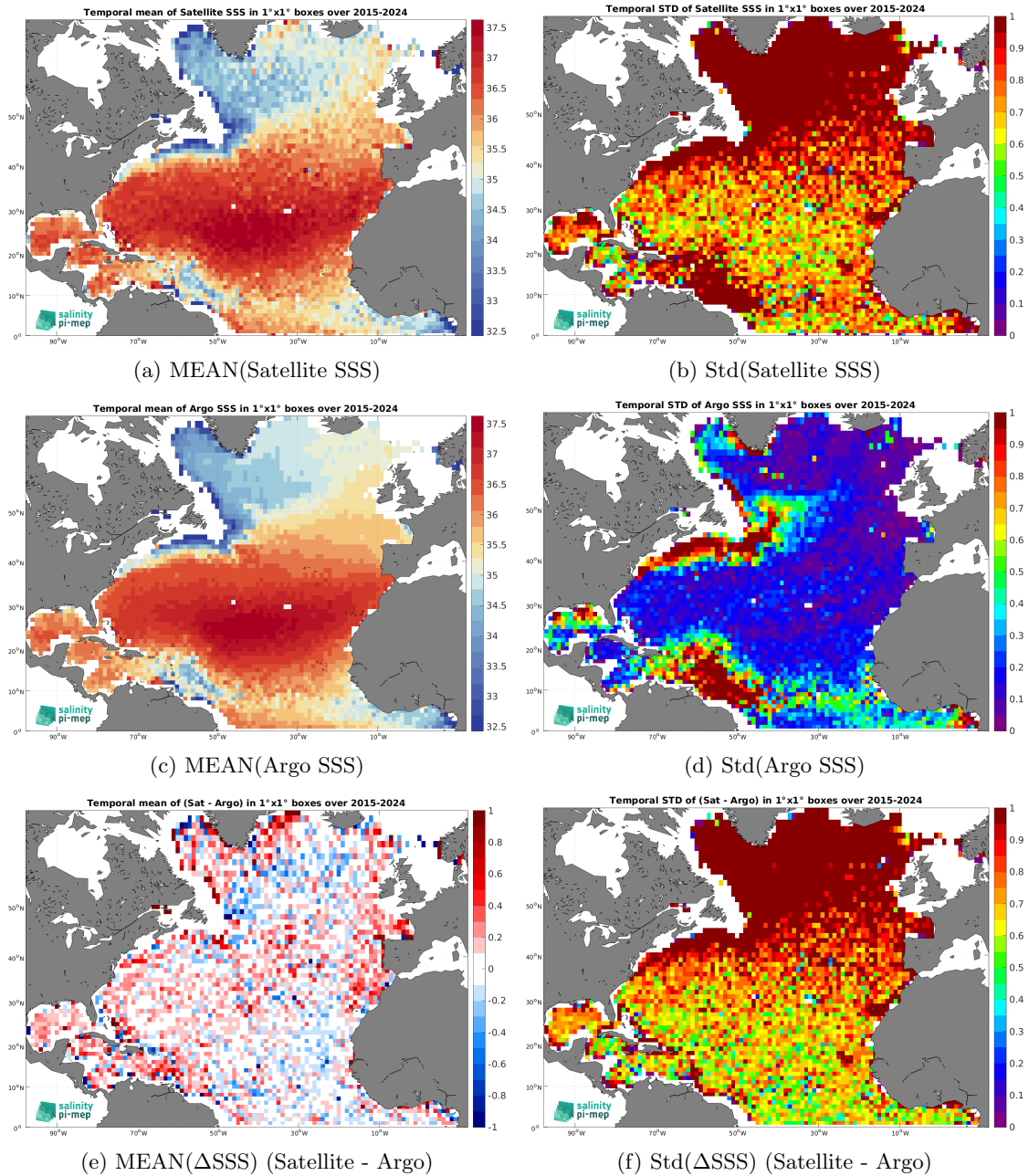
Figure 7: Temporal mean (left) and Std (right) of SSS from SMAP SSS L2 v5.3 - 40 km (RSS) (top), Argo (middle), and of \Delta SSS (Satellite - Argo). Only match-up pairs are used to generate these maps.
