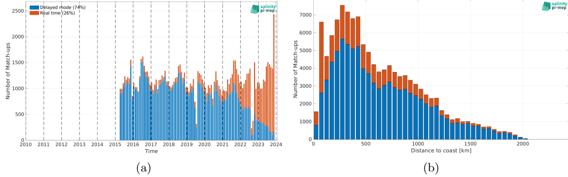
Figure 2: Number of match-ups between Argo and SMAP SSS L2 v5.3 - 40 km (RSS) SSS as a function of time (a) and as function of the distance to coast (b) over the North Atlantic Ocean Pi-MEP region and for the full satellite product period.
