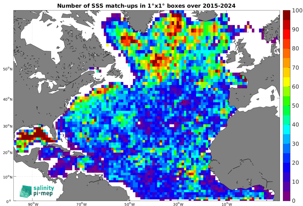
Figure 5: Number of SSS match-ups between Argo SSS and the SMAP SSS L2 v5.3 - 40 km (RSS) SSS product for the North Atlantic Ocean Pi-MEP region over 1^\circ \times 1^\circ boxes and for the full satellite product period.
