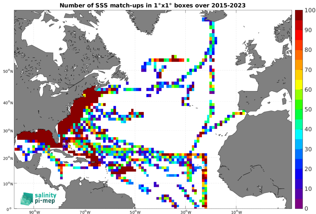
Figure 4: Number of SSS match-ups between TSG (SAMOS) SSS and the SMAP SSS L2 v5 - 40 km (RSS) SSS product for the North Atlantic Ocean Pi-MEP region over 1^\circ \times 1^\circ boxes and for the full satellite product period.
