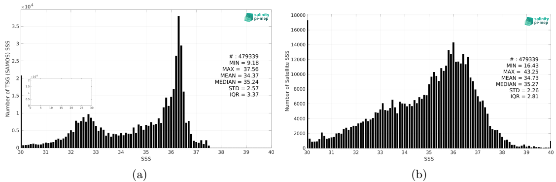
Figure 2: Histograms of SSS from TSG (SAMOS) (a) and SMAP SSS L2 v5 - 40 km (RSS) (b) considering all match-up pairs per bins of 0.1 over the North Atlantic Ocean Pi-MEP region and for the full satellite product period.
