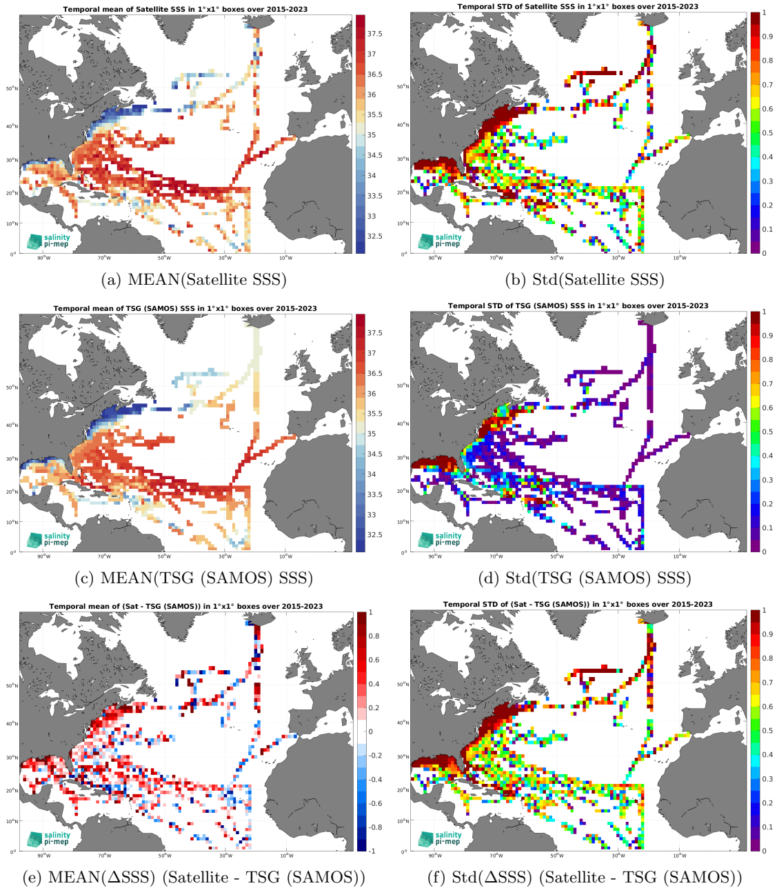
Figure 6: Temporal mean (left) and Std (right) of SSS from SMAP SSS L2 v5 - 40 km (RSS) (top), TSG (SAMOS) (middle), and of \Delta SSS (Satellite - TSG (SAMOS)). Only match-up pairs are used to generate these maps.
