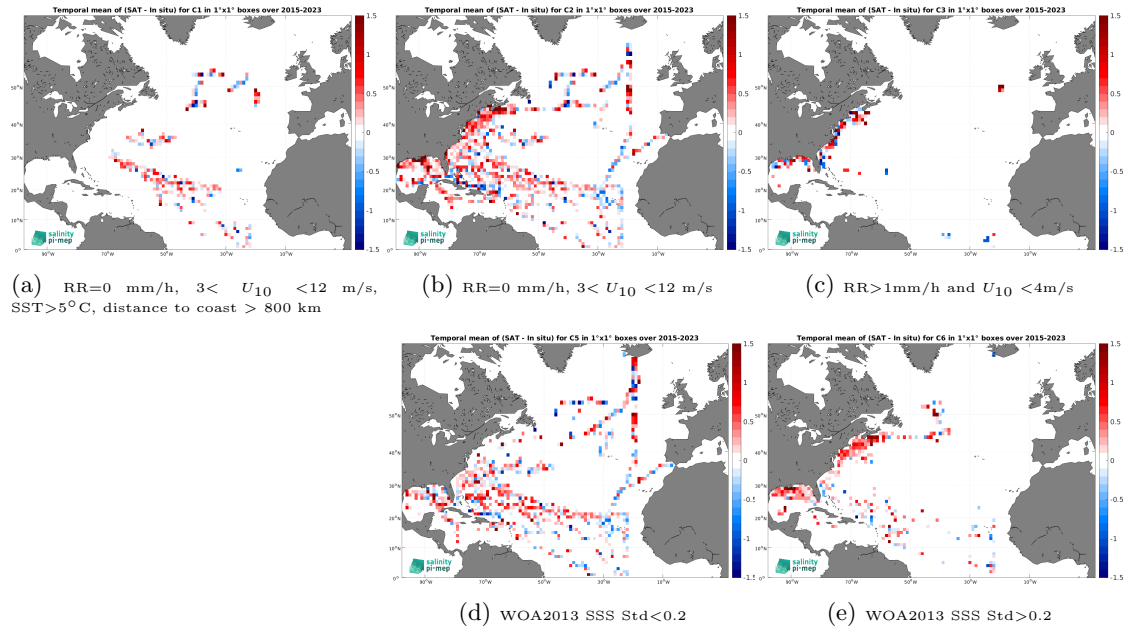
Figure 12: Temporal mean gridded over spatial boxes of size 1^\circ \times 1^\circ of \Delta\text{SSS} (SMAP SSS L2 v5 - 40 km (RSS) - TSG (SAMOS)) for 5 different subdatasets corresponding to:RR=0 mm/h, 3 < U_{10} < 12 m/s, SST >5^\circ\text{C} , distance to coast > 800 km (a), RR=0 mm/h, 3 < U_{10} < 12 m/s (b), RR >1 mm/h and U_{10} < 4 m/s (c), WOA2013 SSS Std <0.2 (d), WOA2013 SSS Std >0.2 (e).
