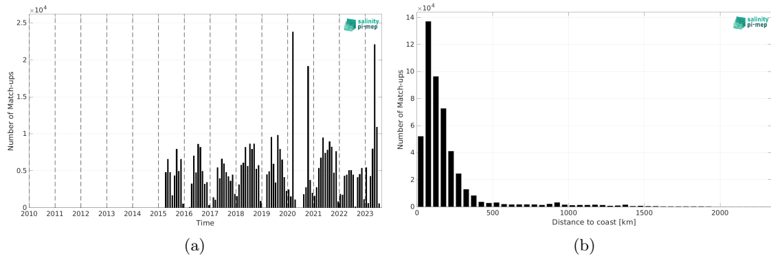
Figure 1: Number of match-ups between TSG (SAMOS) and SMAP SSS L2 v5 - 40 km (RSS) SSS as a function of time (a) and as function of the distance to coast (b) over the North Atlantic Ocean Pi-MEP region and for the full satellite product period.
