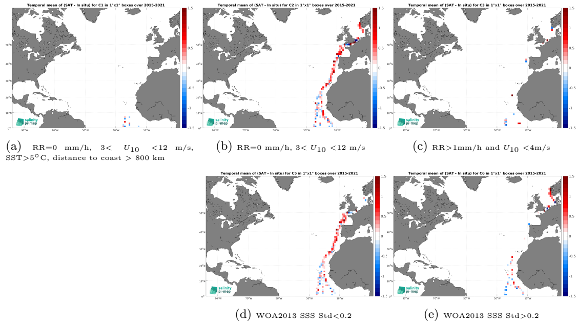
Figure 12: Temporal mean gridded over spatial boxes of size 1^\circ \times 1^\circ of \Delta\text{SSS} (SMAP SSS L2 v5 - 40 km (RSS) - TSG (Polarstern)) for 5 different subdatasets corresponding to:RR=0 mm/h, 3 < U_{10} < 12 m/s, SST >5^\circ\text{C} , distance to coast > 800 km (a), RR=0 mm/h, 3 < U_{10} < 12 m/s (b), RR >1 mm/h and U_{10} < 4 m/s (c), WOA2013 SSS Std <0.2 (d), WOA2013 SSS Std >0.2 (e).
