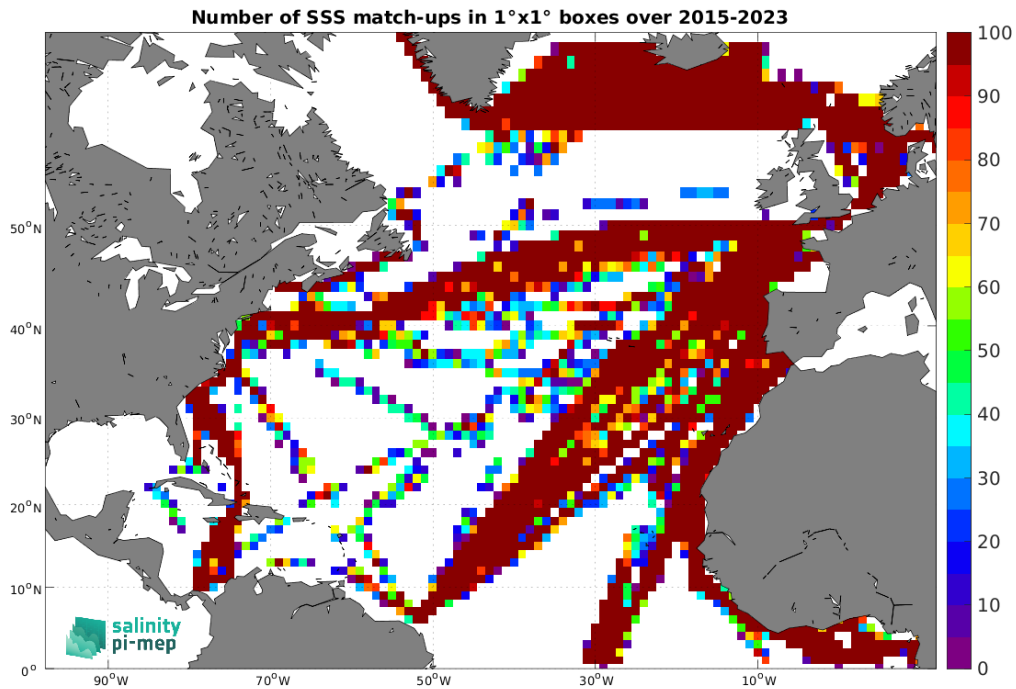
Figure 4: Number of SSS match-ups between TSG (LEGOS-DM) SSS and the SMAP SSS L2 v5 - 40 km (RSS) SSS product for the North Atlantic Ocean Pi-MEP region over 1^\circ \times 1^\circ boxes and for the full satellite product period.
