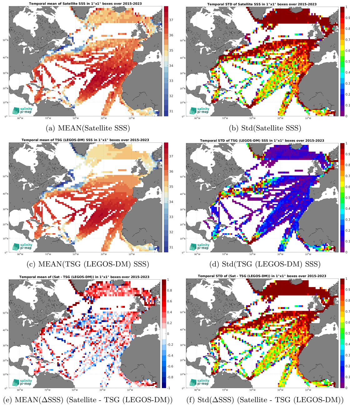
Figure 6: Temporal mean (left) and Std (right) of SSS from SMAP SSS L2 v5 - 40 km (RSS) (top), TSG (LEGOS-DM) (middle), and of \Delta SSS (Satellite - TSG (LEGOS-DM)). Only match-up pairs are used to generate these maps.
