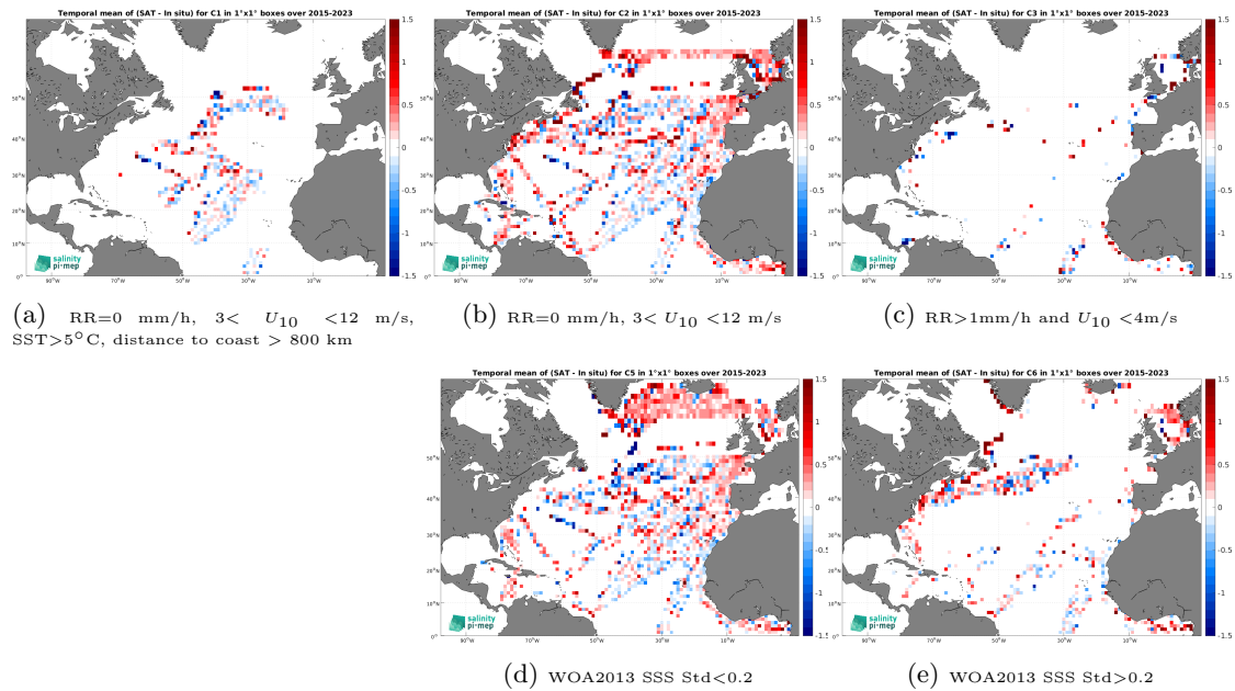
Figure 12: Temporal mean gridded over spatial boxes of size 1^\circ \times 1^\circ of \Delta\text{SSS} (SMAP SSS L2 v5 - 40 km (RSS) - TSG (LEGOS-DM)) for 5 different subdatasets corresponding to:RR=0 mm/h, 3 < U_{10} < 12 m/s, SST >5^\circ\text{C} , distance to coast > 800 km (a), RR=0 mm/h, 3 < U_{10} < 12 m/s (b), RR >1 mm/h and U_{10} < 4 m/s (c), WOA2013 SSS Std <0.2 (d), WOA2013 SSS Std >0.2 (e).
