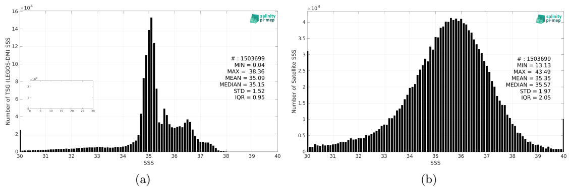
Figure 2: Histograms of SSS from TSG (LEGOS-DM) (a) and SMAP SSS L2 v5 - 40 km (RSS) (b) considering all match-up pairs per bins of 0.1 over the North Atlantic Ocean Pi-MEP region and for the full satellite product period.
