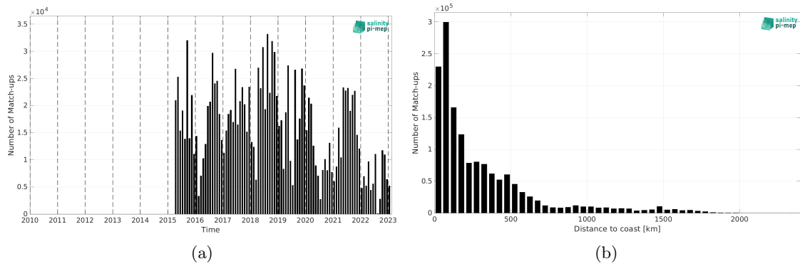
Figure 1: Number of match-ups between TSG (LEGOS-DM) and SMAP SSS L2 v5 - 40 km (RSS) SSS as a function of time (a) and as function of the distance to coast (b) over the North Atlantic Ocean Pi-MEP region and for the full satellite product period.
