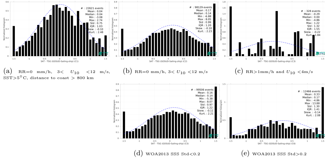
Figure 13: Normalized histogram of \Delta\text{SSS} (SMAP SSS L2 v5 - 40 km (RSS) - TSG (GOSUD-Sailing-ship)) for 5 different subdatasets corresponding to: RR=0 mm/h, 3 < U_{10} < 12 m/s, SST>5°C, distance to coast > 800 km (a), RR=0 mm/h, 3 < U_{10} < 12 m/s (b), RR>1mm/h and U_{10} < 4 m/s (c), WOA2013 SSS Std<0.2 (d), WOA2013 SSS Std>0.2 (e).
