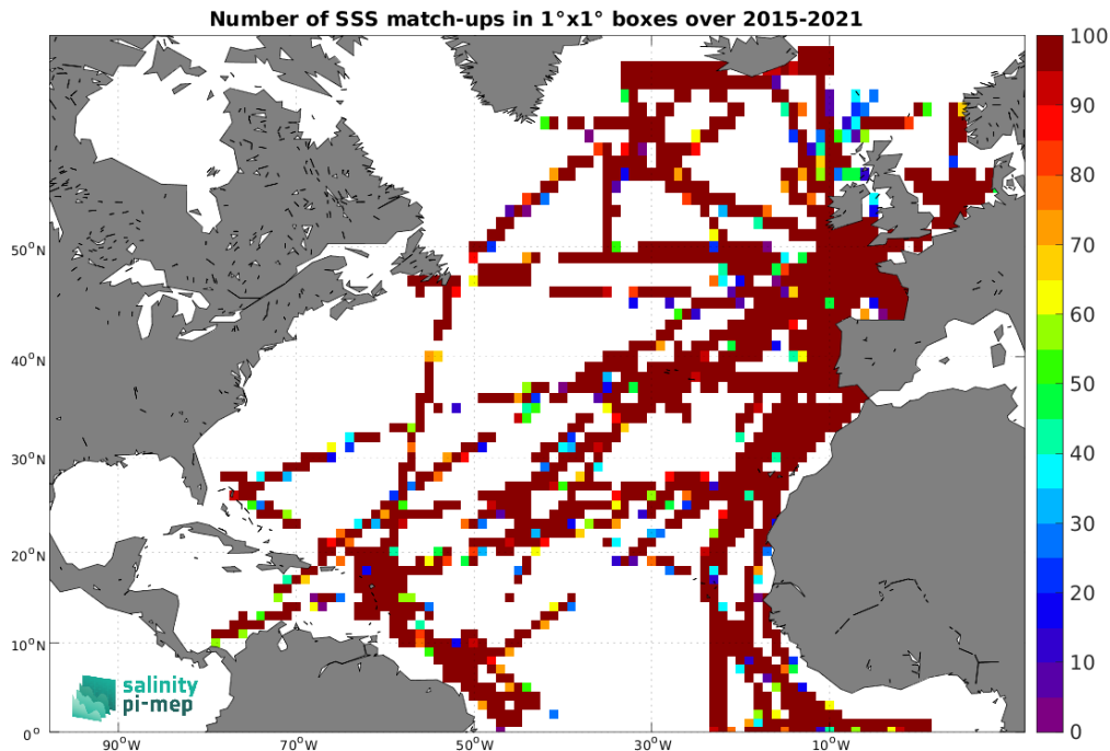
Figure 4: Number of SSS match-ups between TSG (GOSUD-Research-vessel) SSS and the SMAP SSS L2 v5 - 40 km (RSS) SSS product for the North Atlantic Ocean Pi-MEP region over 1^\circ \times 1^\circ boxes and for the full satellite product period.
