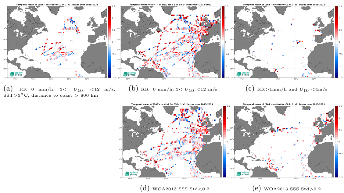
Figure 12: Temporal mean gridded over spatial boxes of size 1^\circ \times 1^\circ of \Delta\text{SSS} (SMAP SSS L2 v5 - 40 km (RSS) - TSG (GOSUD-Research-vessel)) for 5 different subdatasets corresponding to:RR=0 mm/h, 3 < U_{10} < 12 m/s, SST > 5°C, distance to coast > 800 km (a), RR=0 mm/h, 3 < U_{10} < 12 m/s (b), RR > 1mm/h and U_{10} < 4 m/s (c), WOA2013 SSS Std < 0.2 (d), WOA2013 SSS Std > 0.2 (e).
