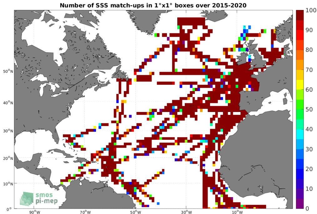
Figure 4: Number of SSS match-ups between TSG (GOSUD-Research-vessel) SSS and the SMAP SSS L2 v5 - 40 km (RSS) SSS product for the North Atlantic Ocean Pi-MEP region over 1°x1° boxes and for the full satellite product period.
