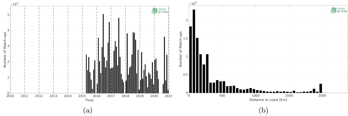
Figure 1: Number of match-ups between TSG (GOSUD-Research-vessel) and SMAP SSS L2 v5 - 40 km (RSS) SSS as a function of time (a) and as function of the distance to coast (b) over the North Atlantic Ocean Pi-MEP region and for the full satellite product period.
