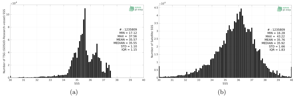
Figure 2: Histograms of SSS from TSG (GOSUD-Research-vessel) (a) and SMAP SSS L2 v5 - 40 km (RSS) (b) considering all match-up pairs per bins of 0.1 over the North Atlantic Ocean Pi-MEP region and for the full satellite product period.
