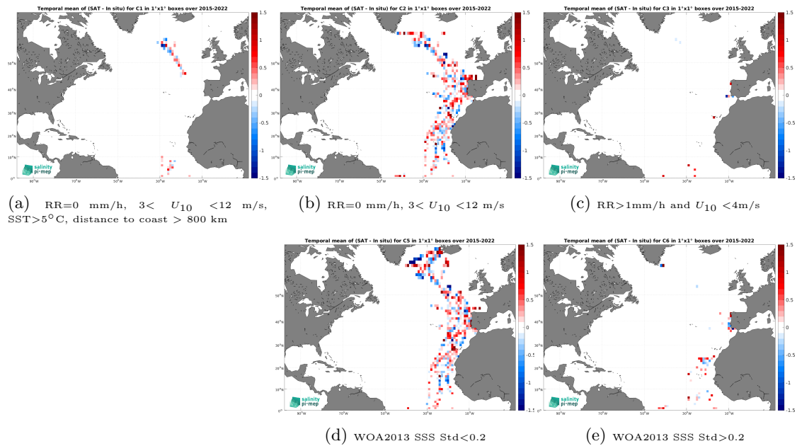
Figure 12: Temporal mean gridded over spatial boxes of size 1^\circ \times 1^\circ of \Delta\text{SSS} (SMAP SSS L2 v5 - 40 km (RSS) - TSG (CSIC-UTM)) for 5 different subdatasets corresponding to:RR=0 mm/h, 3 < U_{10} < 12 m/s, SST >5^\circ\text{C} , distance to coast > 800 km (a), RR=0 mm/h, 3 < U_{10} < 12 m/s (b), RR >1 mm/h and U_{10} < 4 m/s (c), WOA2013 SSS Std <0.2 (d), WOA2013 SSS Std >0.2 (e).
