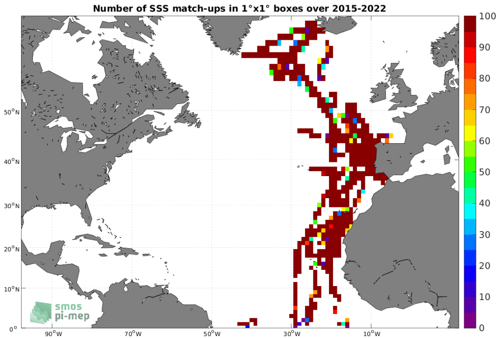
Figure 4: Number of SSS match-ups between TSG (CSIC-UTM) SSS and the SMAP SSS L2 v5 - 40 km (RSS) SSS product for the North Atlantic Ocean Pi-MEP region over 1^\circ \times 1^\circ boxes and for the full satellite product period.
