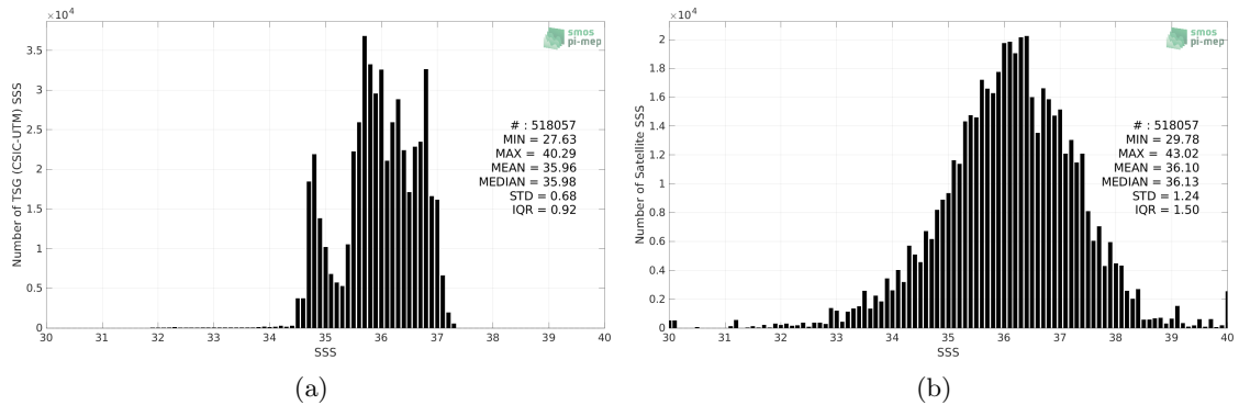
Figure 2: Histograms of SSS from TSG (CSIC-UTM) (a) and SMAP SSS L2 v5 - 40 km (RSS) (b) considering all match-up pairs per bins of 0.1 over the North Atlantic Ocean Pi-MEP region and for the full satellite product period.
