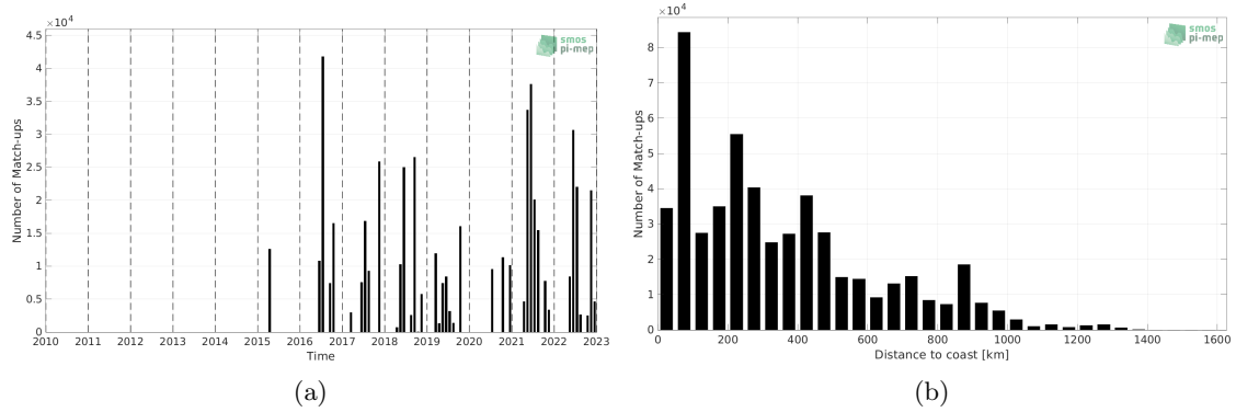
Figure 1: Number of match-ups between TSG (CSIC-UTM) and SMAP SSS L2 v5 - 40 km (RSS) SSS as a function of time (a) and as function of the distance to coast (b) over the North Atlantic Ocean Pi-MEP region and for the full satellite product period.
