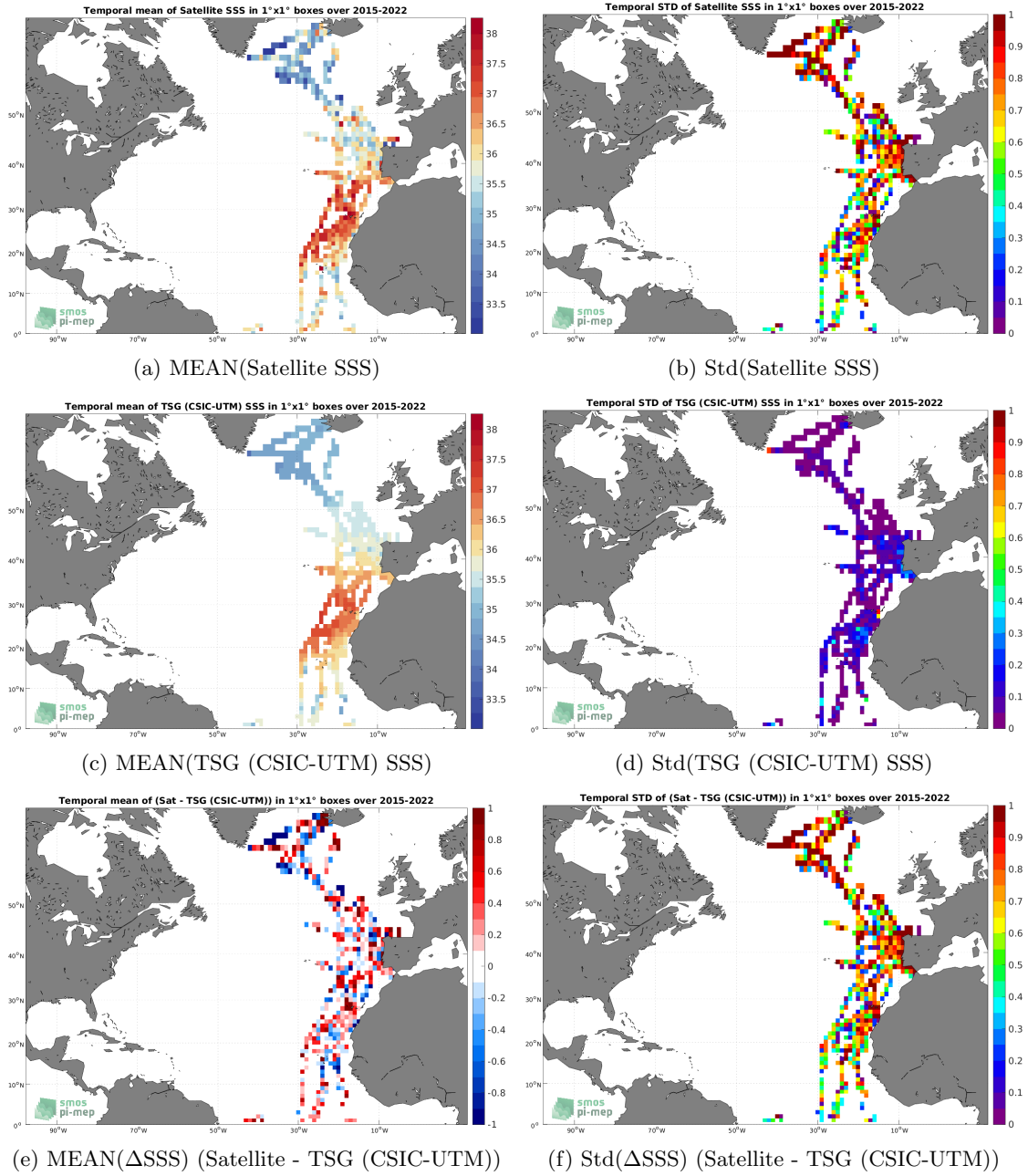
Figure 6: Temporal mean (left) and Std (right) of SSS from SMAP SSS L2 v5 - 40 km (RSS) (top), TSG (CSIC-UTM) (middle), and of \Delta SSS (Satellite - TSG (CSIC-UTM)). Only match-up pairs are used to generate these maps.
