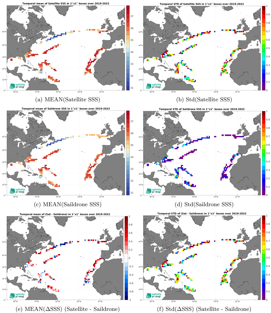
Figure 6: Temporal mean (left) and Std (right) of SSS from SMAP SSS L2 v5 - 40 km (RSS) (top), Saildrone (middle), and of \Delta SSS (Satellite - Saildrone). Only match-up pairs are used to generate these maps.
