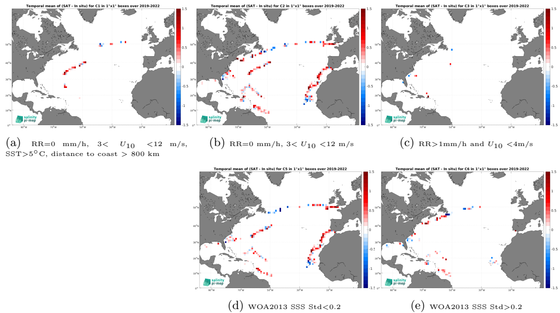
Figure 12: Temporal mean gridded over spatial boxes of size 1^\circ \times 1^\circ of \Delta\text{SSS} (SMAP SSS L2 v5 - 40 km (RSS) - Saldrone) for 5 different subdatasets corresponding to:RR=0 mm/h, 3 < U_{10} < 12 m/s, SST >5^\circ\text{C} , distance to coast > 800 km (a), RR=0 mm/h, 3 < U_{10} < 12 m/s (b), RR >1 mm/h and U_{10} < 4 m/s (c), WOA2013 SSS Std <0.2 (d), WOA2013 SSS Std >0.2 (e).
