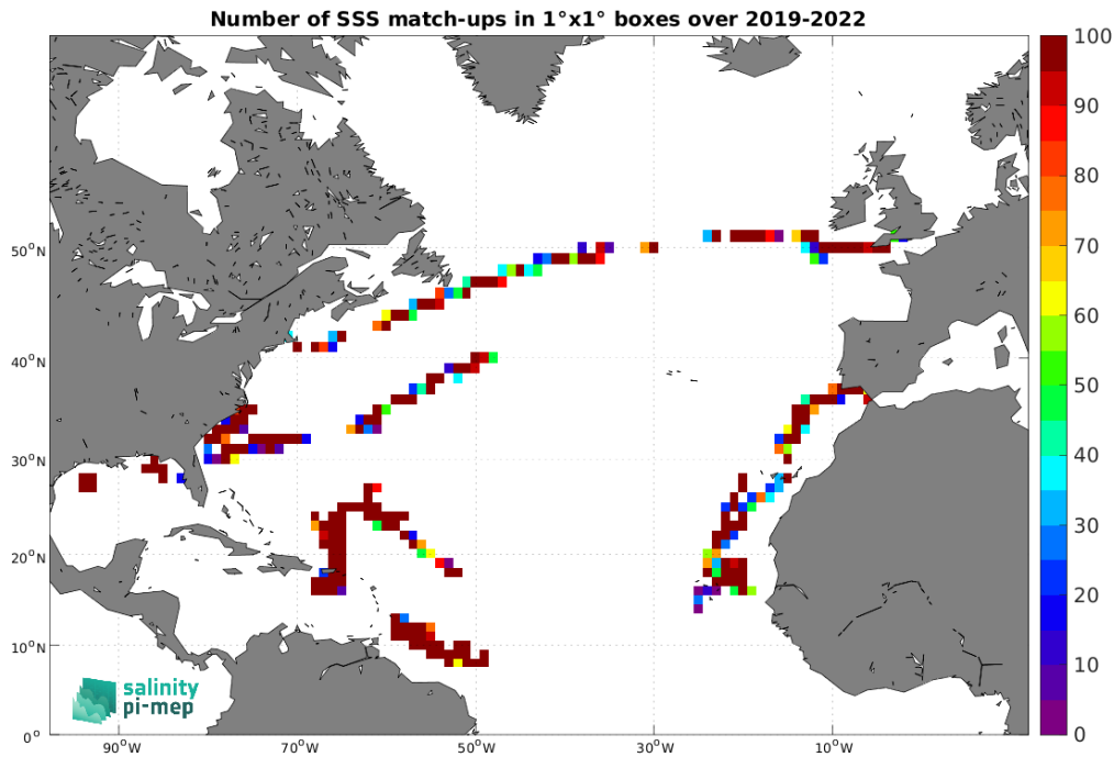
Figure 4: Number of SSS match-ups between Saildrone SSS and the SMAP SSS L2 v5 - 40 km (RSS) SSS product for the North Atlantic Ocean Pi-MEP region over 1^\circ \times 1^\circ boxes and for the full satellite product period.
