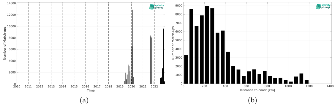
Figure 1: Number of match-ups between Sailability and SMAP SSS L2 v5 - 40 km (RSS) SSS as a function of time (a) and as function of the distance to coast (b) over the North Atlantic Ocean Pi-MEP region and for the full satellite product period.
