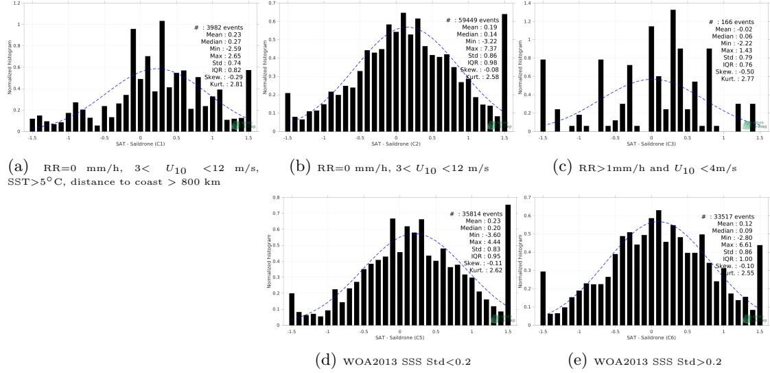
Figure 13: Normalized histogram of \Delta SSS (SMAP SSS L2 v5 - 40 km (RSS) - Saildrone) for 5 different subdatasets corresponding to: RR=0 mm/h, 3 < U_{10} < 12 m/s, SST>5°C, distance to coast > 800 km (a), RR=0 mm/h, 3 < U_{10} < 12 m/s (b), RR>1mm/h and U_{10} < 4 m/s (c), WOA2013 SSS Std<0.2 (d), WOA2013 SSS Std>0.2 (e).
