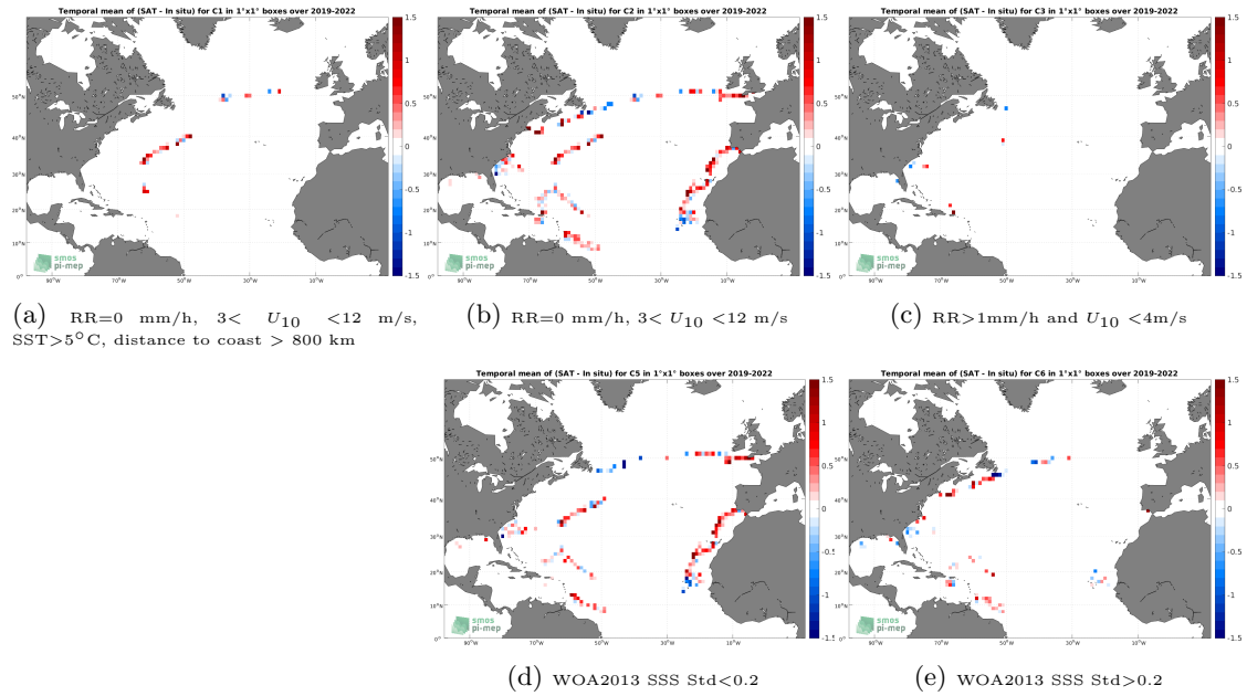
Figure 12: Temporal mean gridded over spatial boxes of size 1^\circ \times 1^\circ of \Delta SSS (SMAP SSS L2 v5 - 40 km (RSS) - Saldrone) for 5 different subdatasets corresponding to:RR=0 mm/h, 3 < U_{10} < 12 m/s, SST >5^\circ C, distance to coast > 800 km (a), RR=0 mm/h, 3 < U_{10} < 12 m/s (b), RR >1 mm/h and U_{10} < 4 m/s (c), WOA2013 SSS Std <0.2 (d), WOA2013 SSS Std >0.2 (e).
