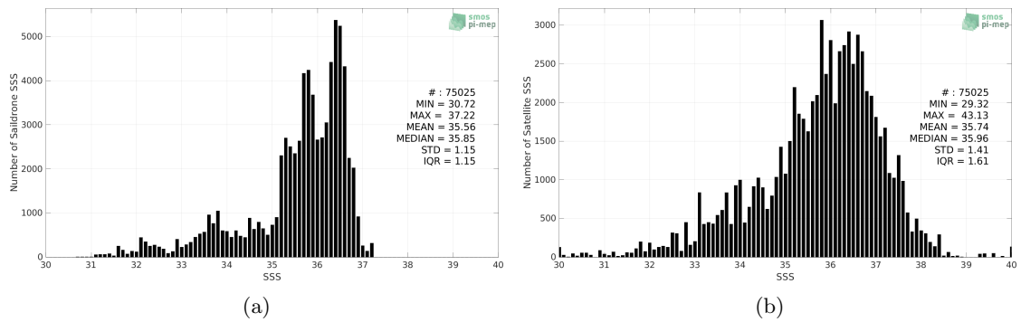
Figure 2: Histograms of SSS from Sailerdrone (a) and SMAP SSS L2 v5 - 40 km (RSS) (b) considering all match-up pairs per bins of 0.1 over the North Atlantic Ocean Pi-MEP region and for the full satellite product period.
