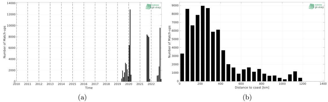
Figure 1: Number of match-ups between Sailerdrone and SMAP SSS L2 v5 - 40 km (RSS) SSS as a function of time (a) and as function of the distance to coast (b) over the North Atlantic Ocean Pi-MEP region and for the full satellite product period.
