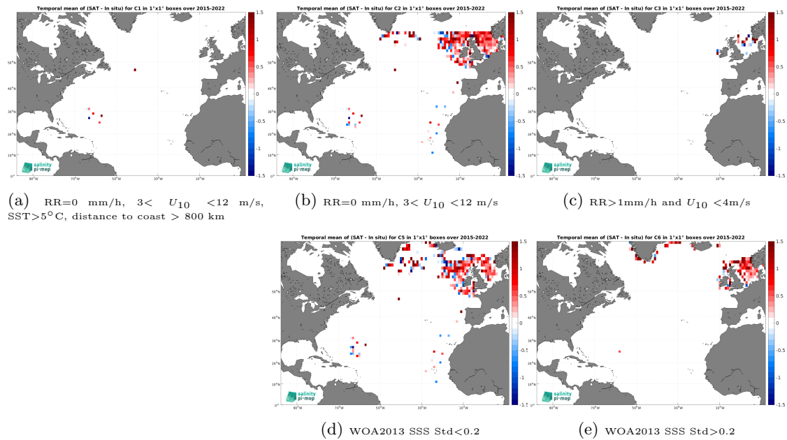
Figure 12: Temporal mean gridded over spatial boxes of size 1^\circ \times 1^\circ of \Delta\text{SSS} (SMAP SSS L2 v5 - 40 km (RSS) - ICES) for 5 different subdatasets corresponding to:RR=0 mm/h, 3 < U_{10} < 12 m/s, SST >5^\circ\text{C} , distance to coast > 800 km (a), RR=0 mm/h, 3 < U_{10} < 12 m/s (b), RR >1 mm/h and U_{10} < 4 m/s (c), WOA2013 SSS Std <0.2 (d), WOA2013 SSS Std >0.2 (e).
