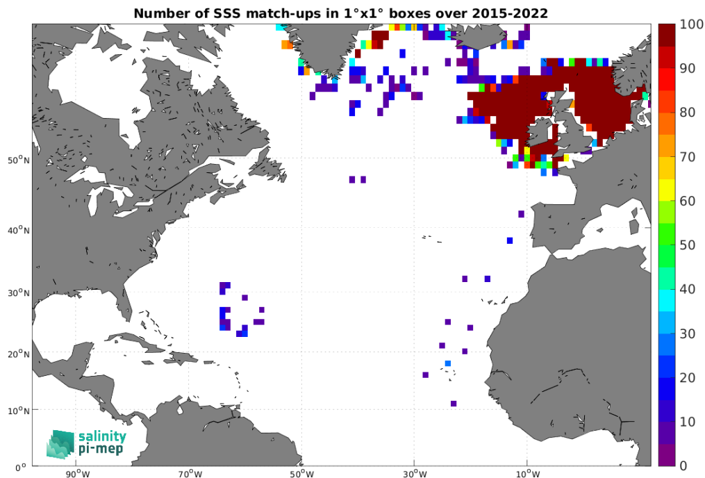
Figure 4: Number of SSS match-ups between ICES SSS and the SMAP SSS L2 v5 - 40 km (RSS) SSS product for the North Atlantic Ocean Pi-MEP region over 1^\circ \times 1^\circ boxes and for the full satellite product period.
