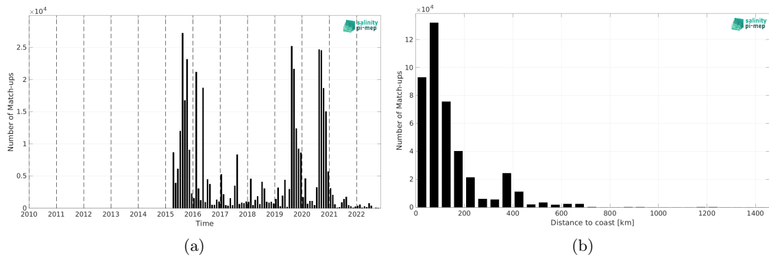
Figure 1: Number of match-ups between ICES and SMAP SSS L2 v5 - 40 km (RSS) SSS as a function of time (a) and as function of the distance to coast (b) over the North Atlantic Ocean Pi-MEP region and for the full satellite product period.
