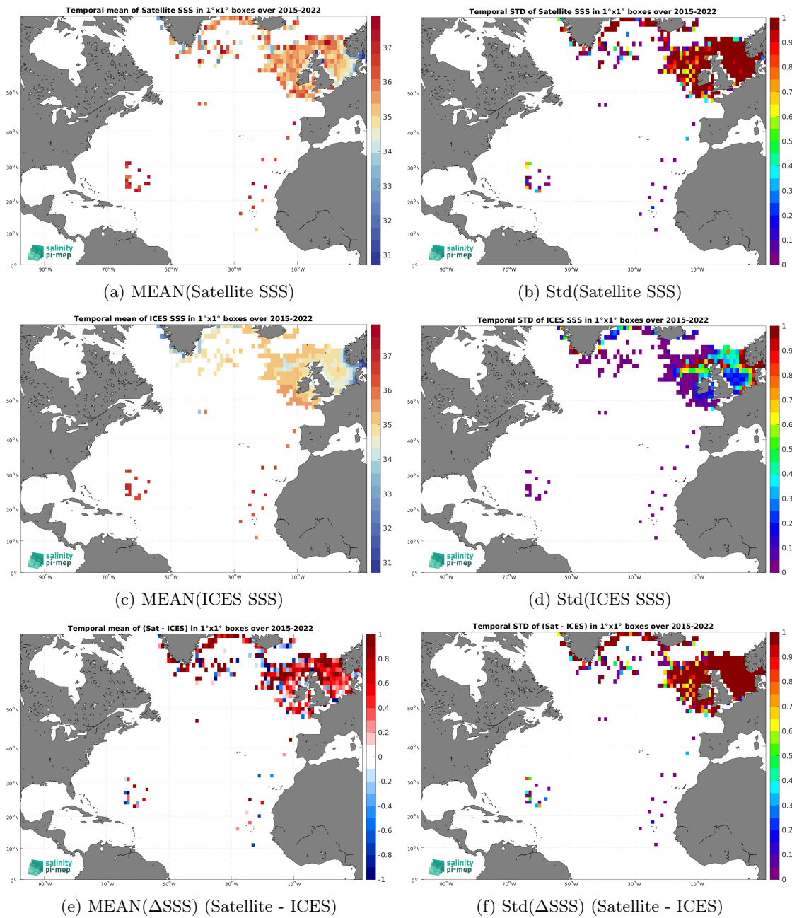
Figure 6: Temporal mean (left) and Std (right) of SSS from SMAP SSS L2 v5 - 40 km (RSS) (top), ICES (middle), and of \Delta SSS (Satellite - ICES). Only match-up pairs are used to generate these maps.
