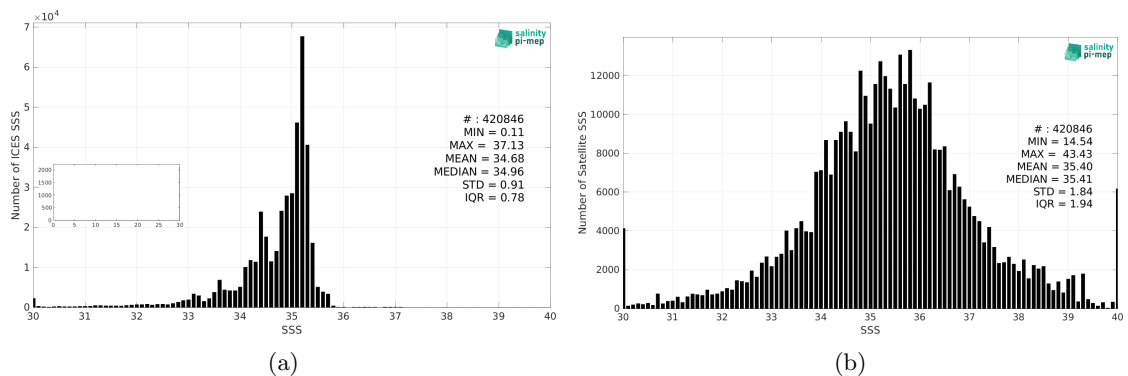
Figure 2: Histograms of SSS from ICES (a) and SMAP SSS L2 v5 - 40 km (RSS) (b) considering all match-up pairs per bins of 0.1 over the North Atlantic Ocean Pi-MEP region and for the full satellite product period.
