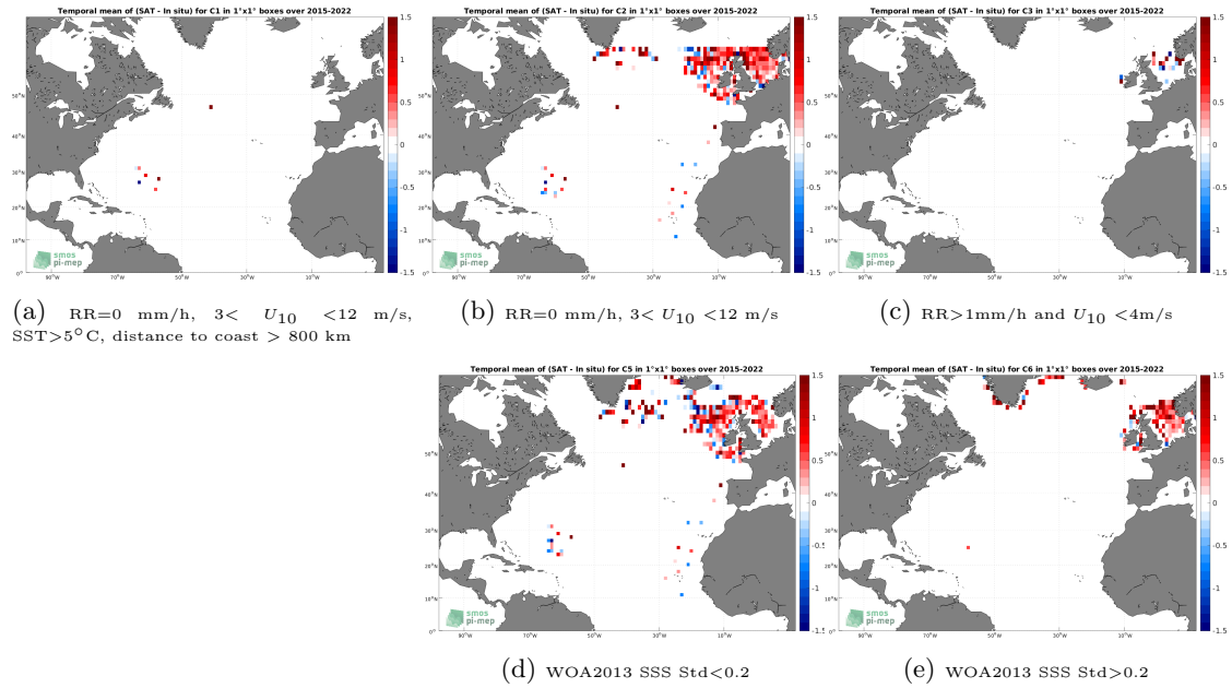
Figure 12: Temporal mean gridded over spatial boxes of size 1^\circ \times 1^\circ of \Delta SSS (SMAP SSS L2 v5 - 40 km (RSS) - ICES) for 5 different subdatasets corresponding to:RR=0 mm/h, 3 < U_{10} < 12 m/s, SST >5^\circ C, distance to coast > 800 km (a), RR=0 mm/h, 3 < U_{10} < 12 m/s (b), RR >1 mm/h and U_{10} < 4 m/s (c), WOA2013 SSS Std <0.2 (d), WOA2013 SSS Std >0.2 (e).
