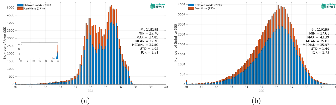
Figure 2: Histograms of SSS from Argo (a) and SMAP SSS L2 v5 - 40 km (RSS) (b) considering all match-up pairs per bins of 0.1 over the North Atlantic Ocean Pi-MEP region and for the full satellite product period.
