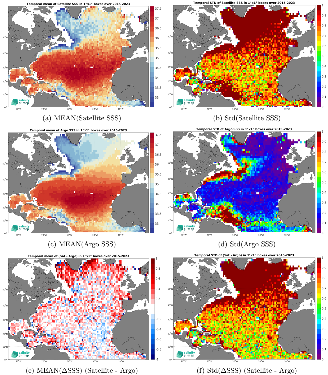
Figure 6: Temporal mean (left) and Std (right) of SSS from SMAP SSS L2 v5 - 40 km (RSS) (top), Argo (middle), and of \Delta SSS (Satellite - Argo). Only match-up pairs are used to generate these maps.
