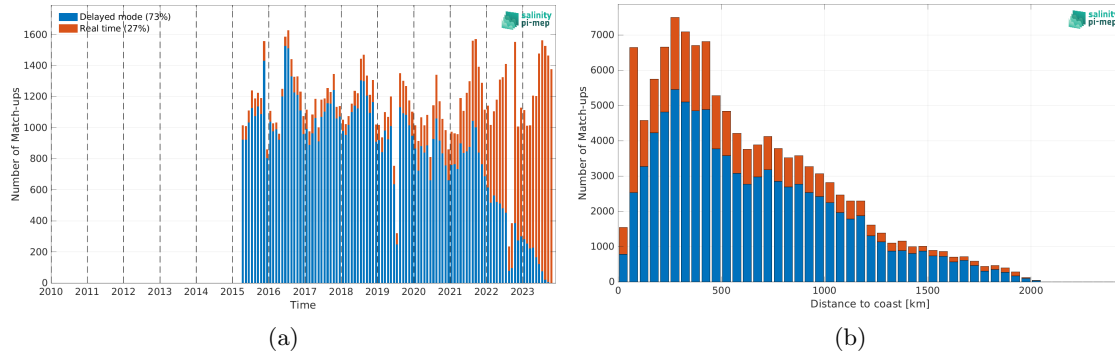
Figure 1: Number of match-ups between Argo and SMAP SSS L2 v5 - 40 km (RSS) SSS as a function of time (a) and as function of the distance to coast (b) over the North Atlantic Ocean Pi-MEP region and for the full satellite product period.
