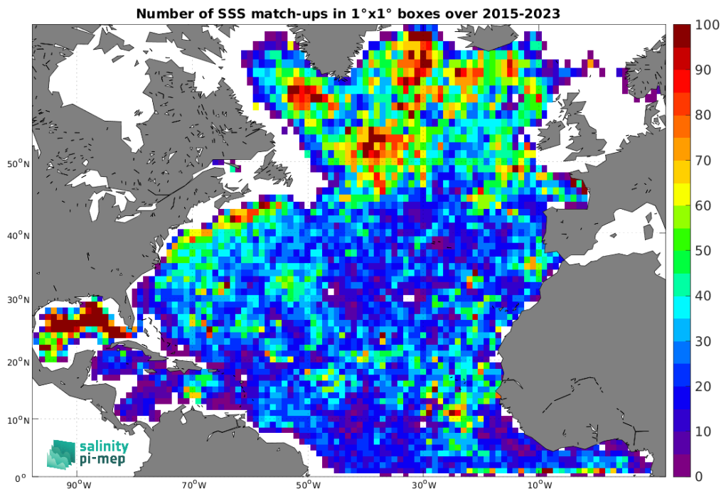
Figure 4: Number of SSS match-ups between Argo SSS and the SMAP SSS L2 v5 - 40 km (RSS) SSS product for the North Atlantic Ocean Pi-MEP region over 1^\circ \times 1^\circ boxes and for the full satellite product period.
